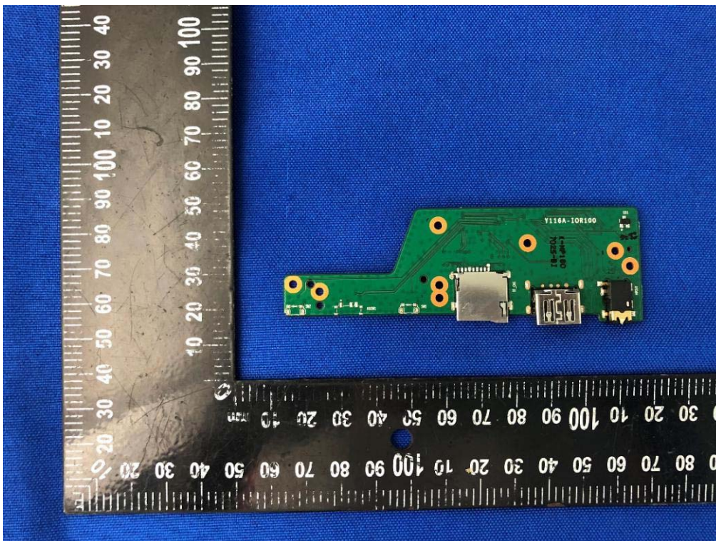
MAIN BOARD REAR VIEW (Sample 1)
