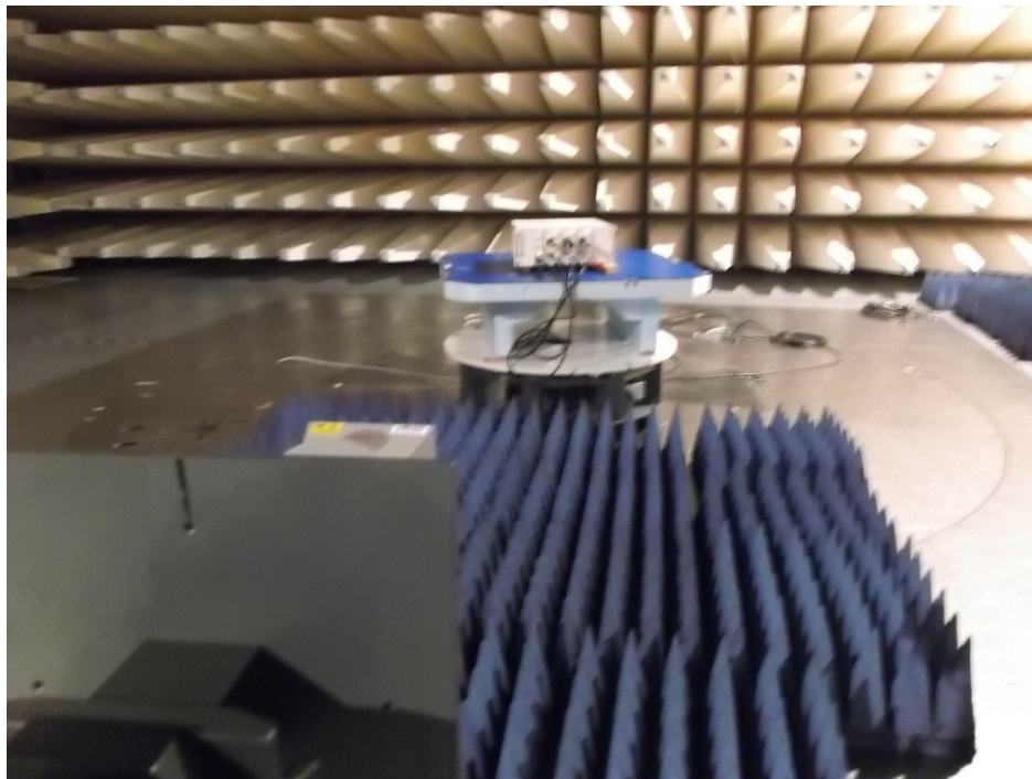
Test setup: Field Strength Emission 18 – 26.5 GHz @3m in the SAC
