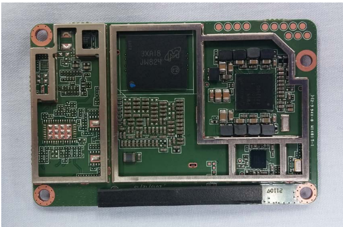
Rear_remove shield can
