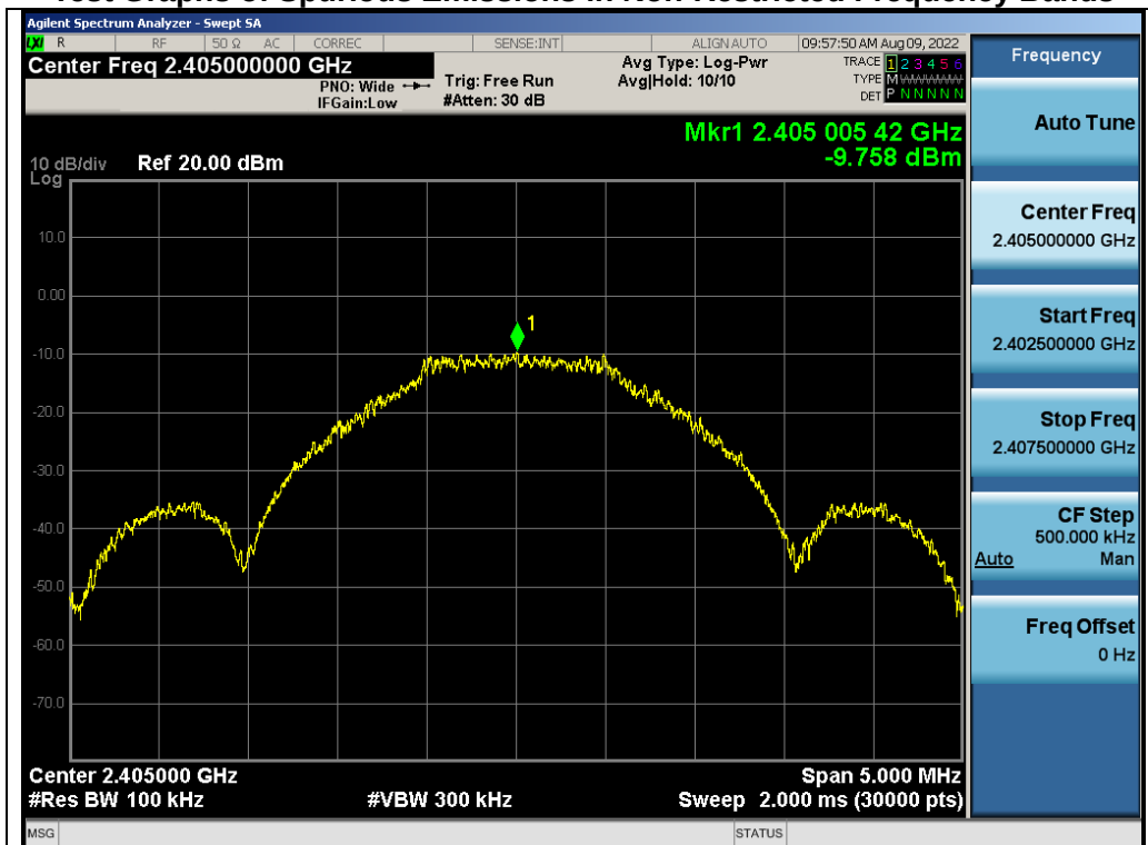
Test_Graph_GFSK_ANT1_2405_Reference Level
