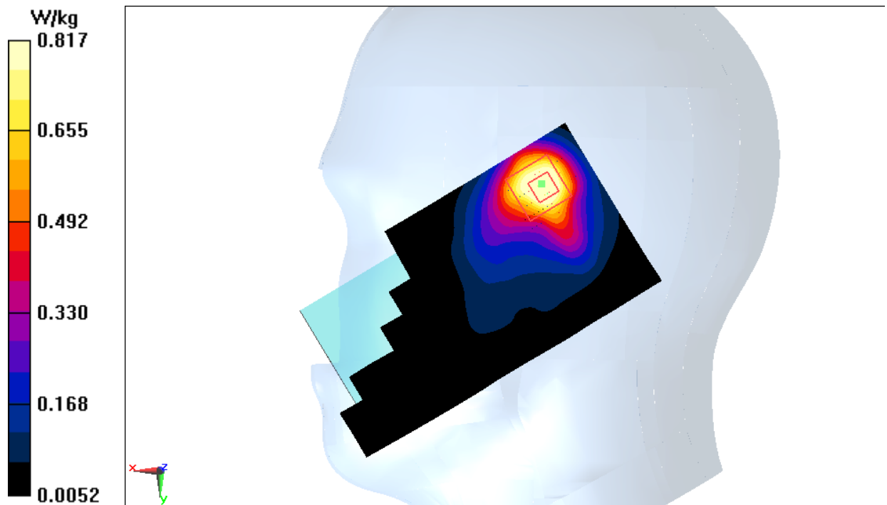
Fig.11 2450 MHz
