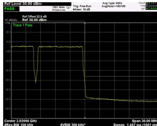
High Band Edge, 2 Carrier, Modulation: 64QAM, BW=10MHz
