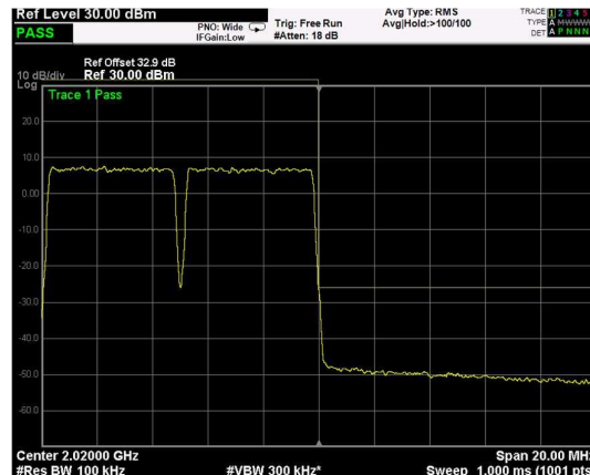
High Band Edge, 2 Carrier, Modulation: 256QAM, BW=5MHz
