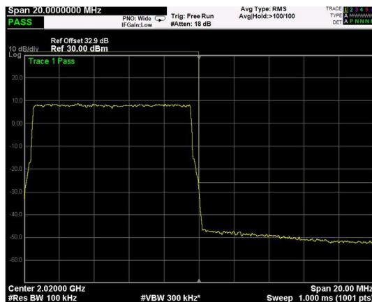
High Band Edge, 1 Carrier, Modulation: 16QAM, BW=10MHz
