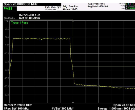
High Band Edge, 1 Carrier, Modulation: 64QAM, BW=10MHz
