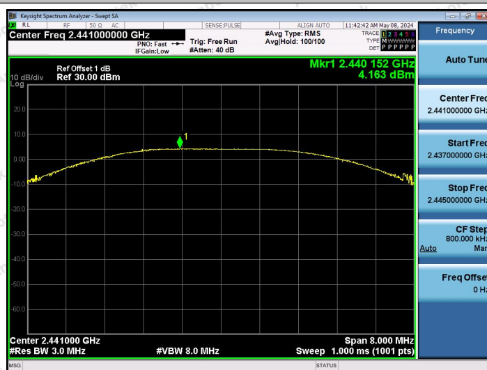
2.4G-Ant1-2441-PASS
