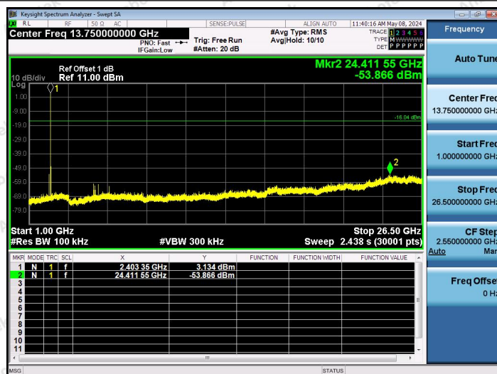
2.4G-Ant1-2403-1000~26500-PASS
