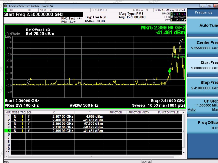
2.4G-Ant1-Hop_2403-PASS
