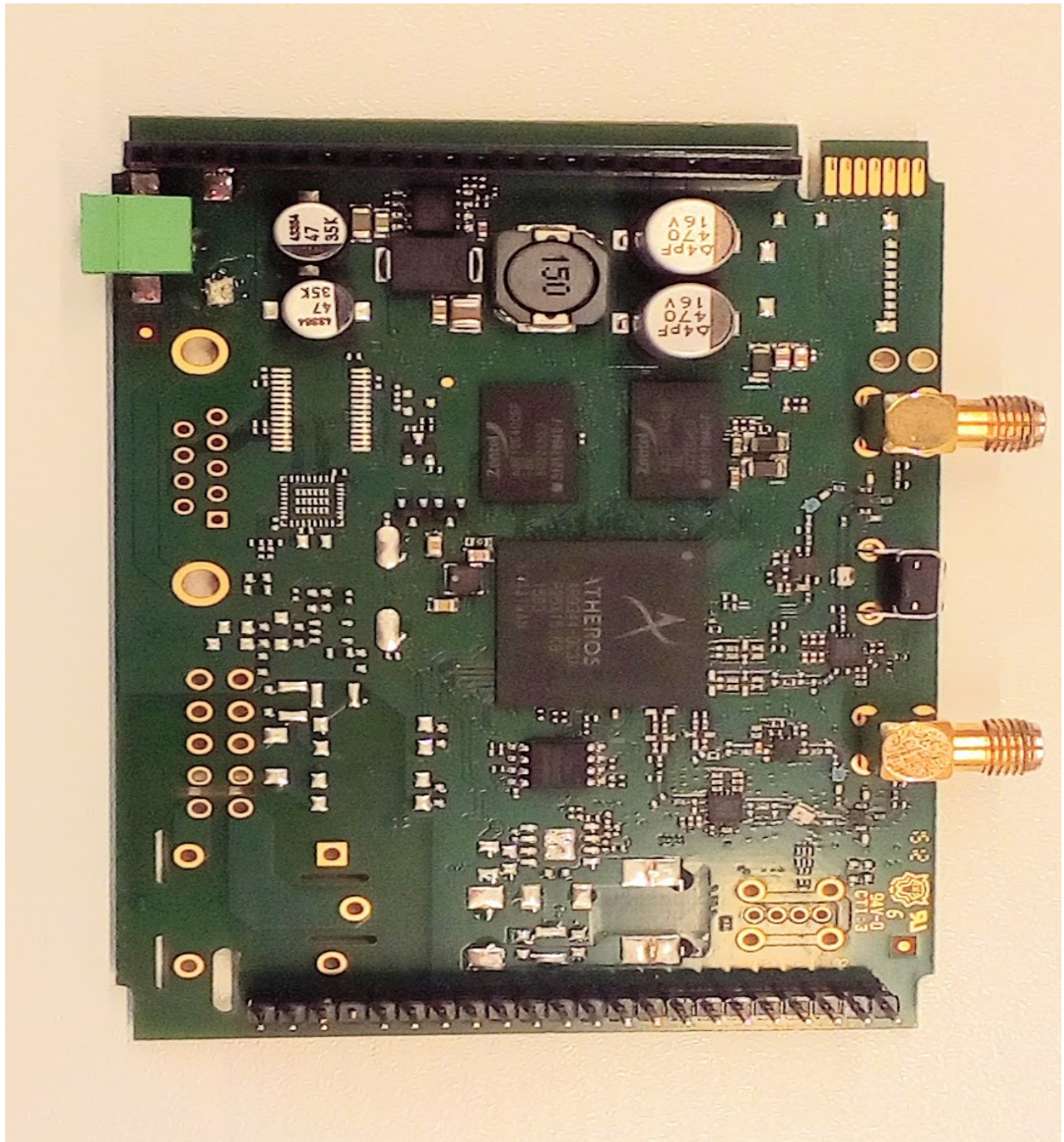
RUT950 Main Top
