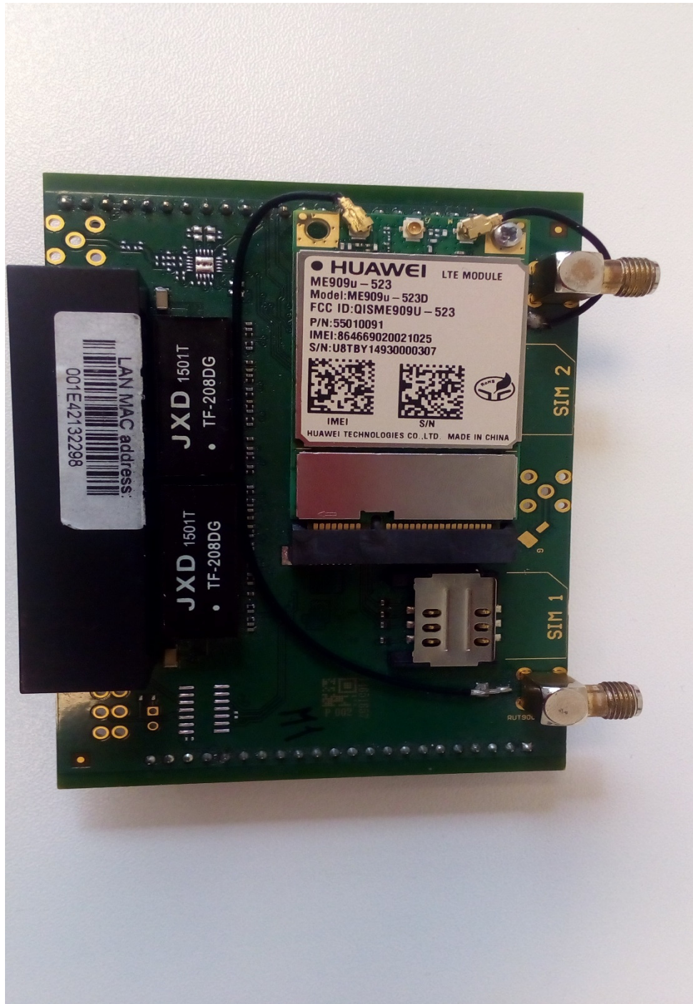
RUT950 RF Top
