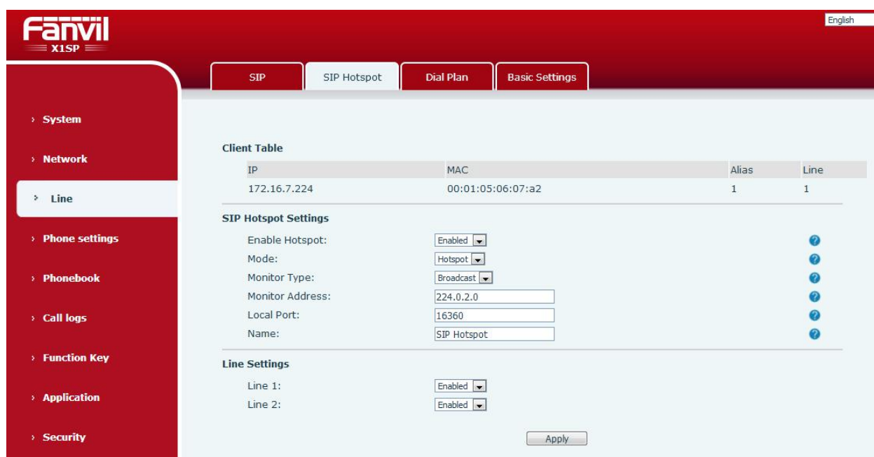
Picture 82 - SIP hotspot server configuration
