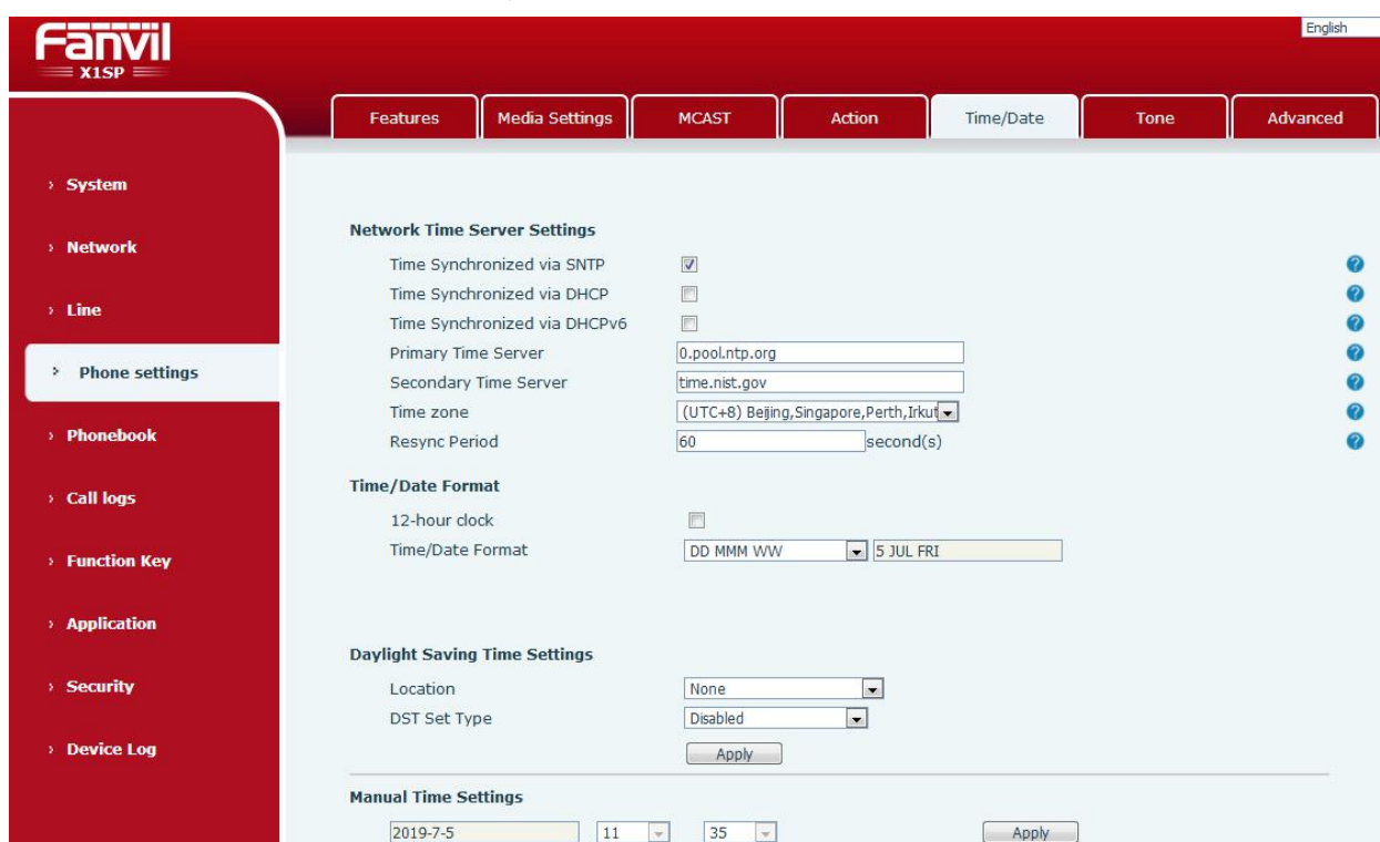
Picture 87 - Set time & date on webpage
