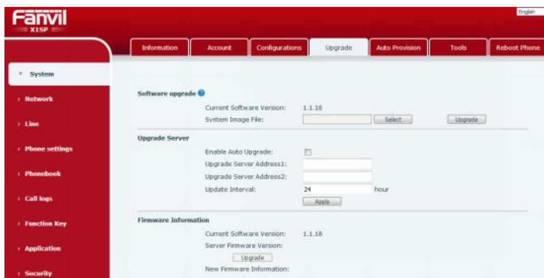
Picture 125 - Web page firmware upgrade
