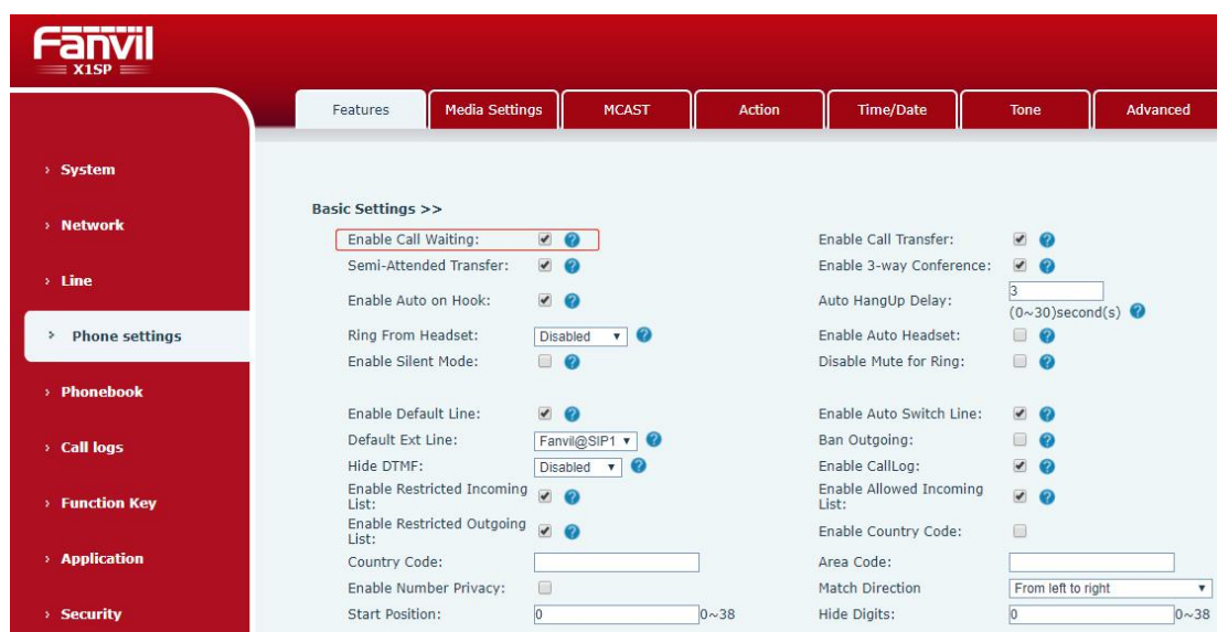
Picture 42 - Web call waiting setting
