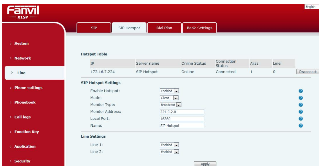
Picture 83 - SIP hotspot client configuration
