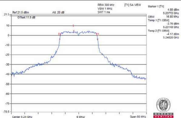
802.11n (HT20) / Chain 0 / Ch 48
