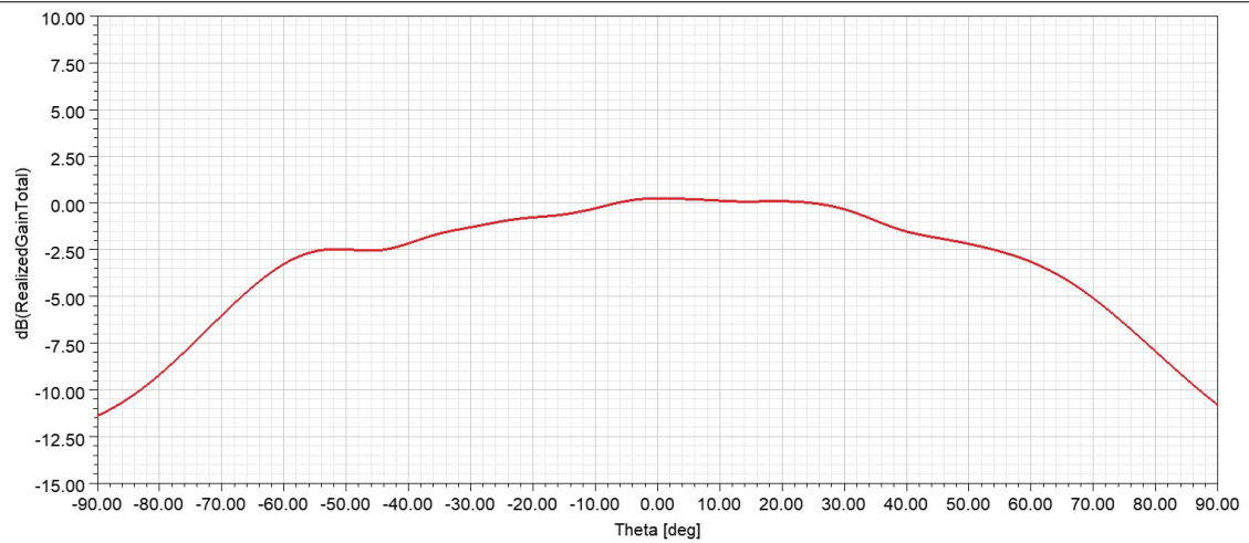
方位面方向图(TX1)Freq:62.0GHz
