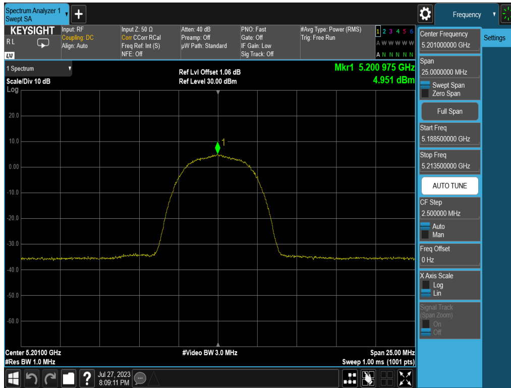
Plot 7-29. PSD (HDR8, 5201MHz)
