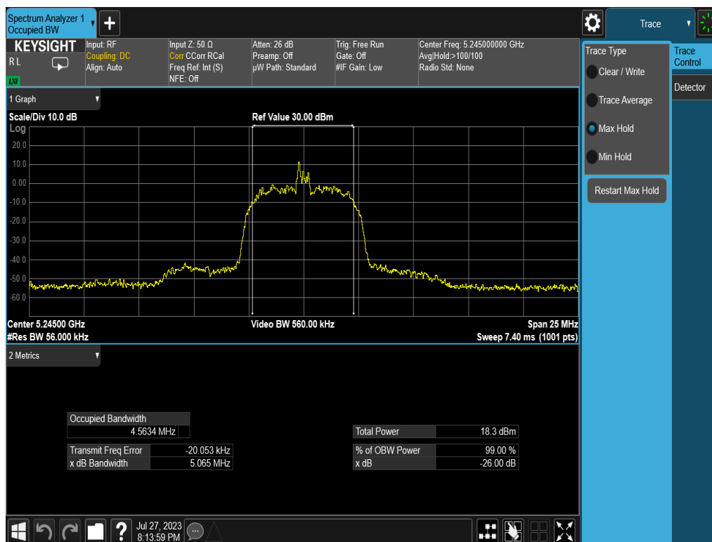
Plot 7-6. 26dB BW & 99% OBW (HDR8, 5245MHz)
