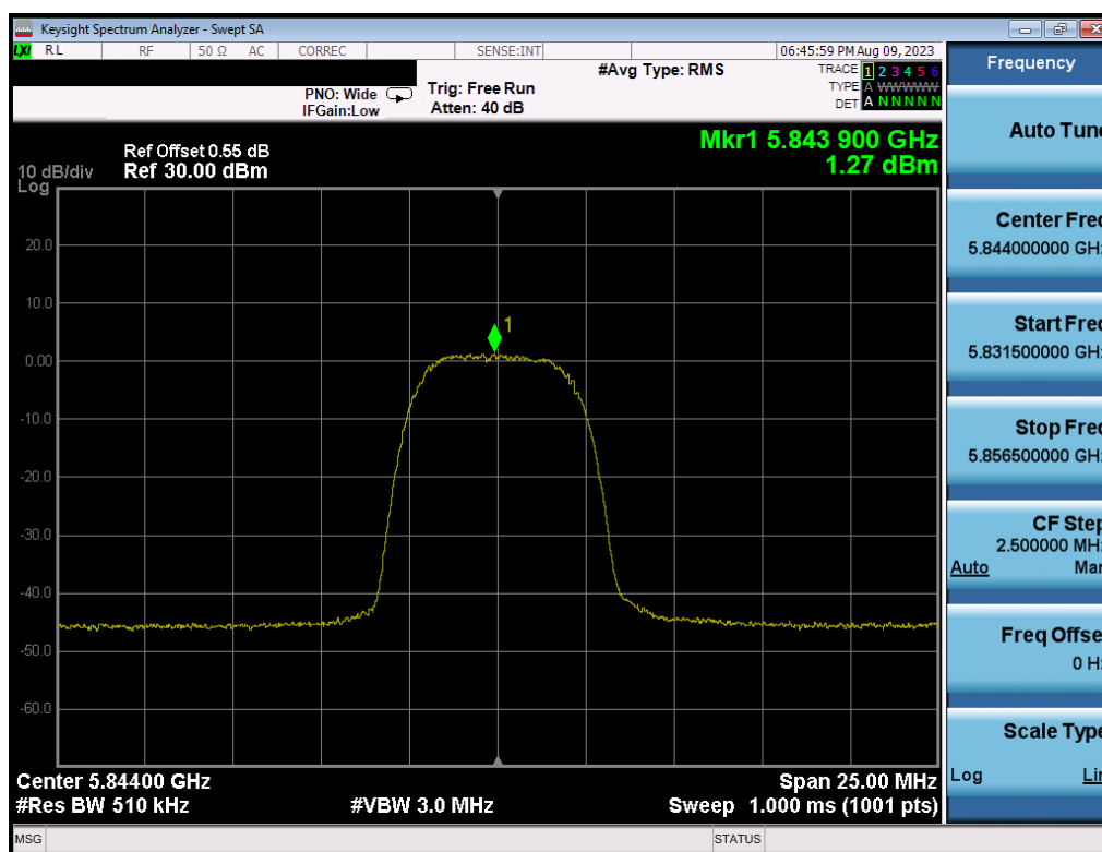
Plot 7-48. PSD (HDRp8, 5844MHz)
