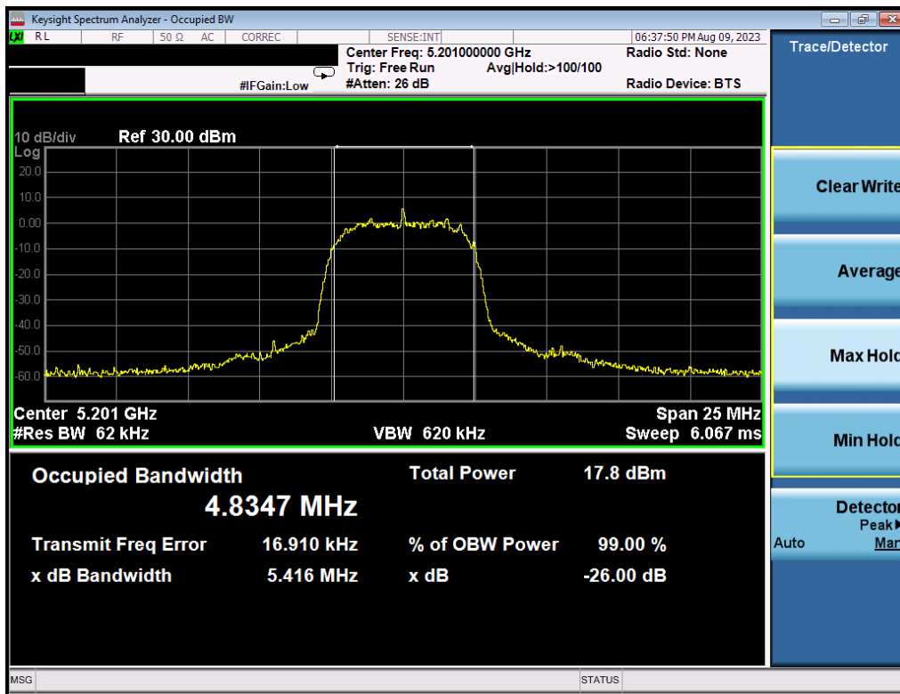
Plot 7-11. 26dB BW & 99% OBW (HDRp8, 5201MHz)
