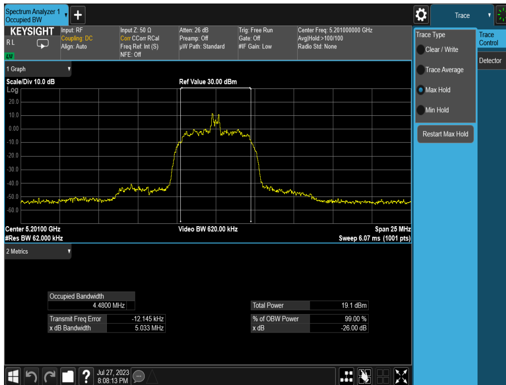
Plot 7-5. 26dB BW & 99% OBW (HDR8, 5201MHz)
