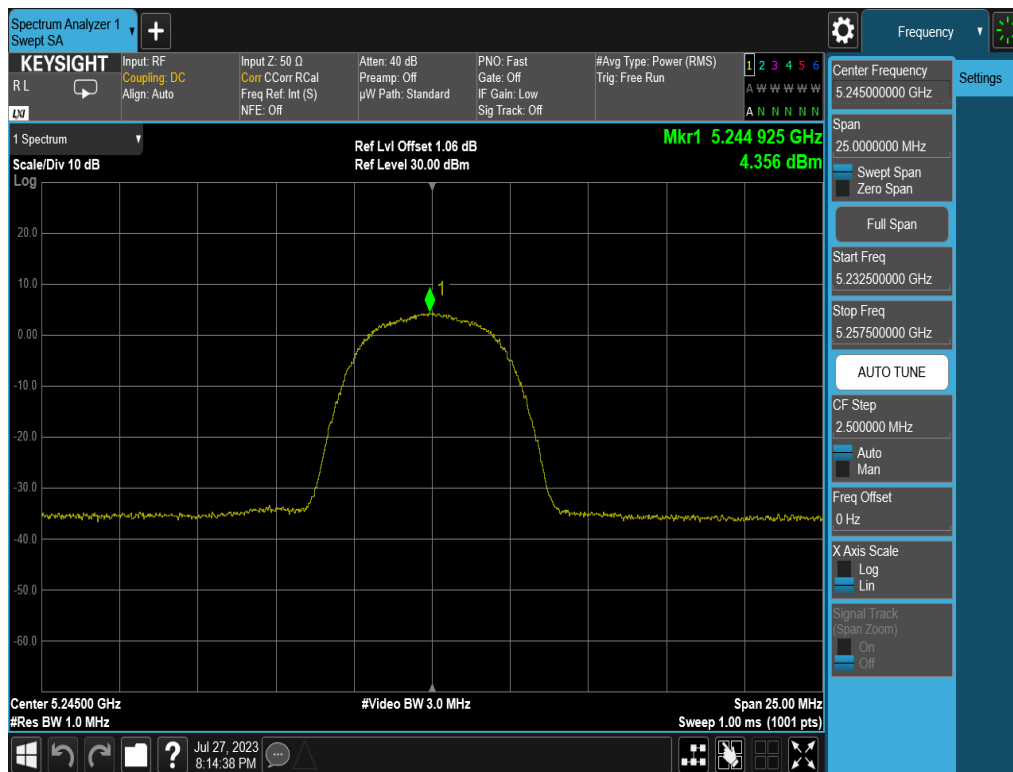
Plot 7-30. PSD (HDR8, 5245MHz)
