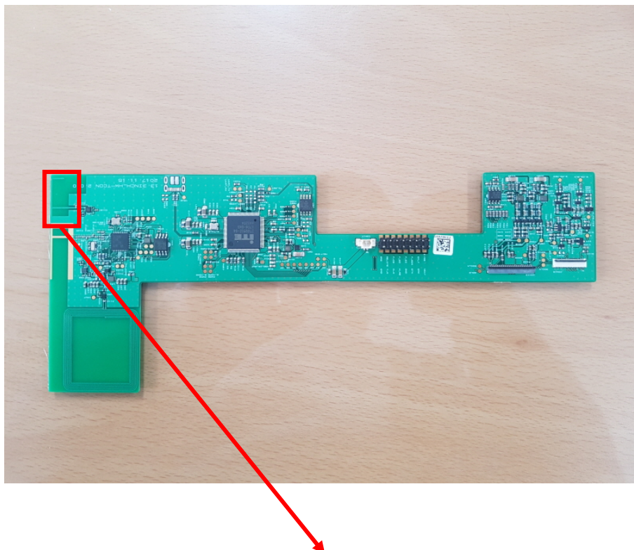
Zigbee receiving Antenna (Wake Up)
