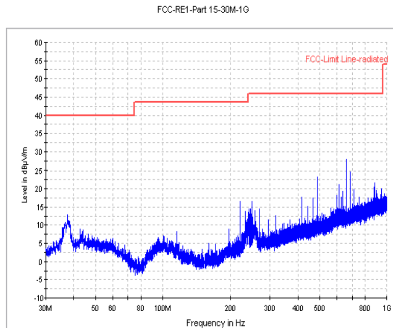
Fig. 52 Radiated Spurious Emission ( \pi/4 DQPSK, Ch0, 30 MHz ~1 GHz)
