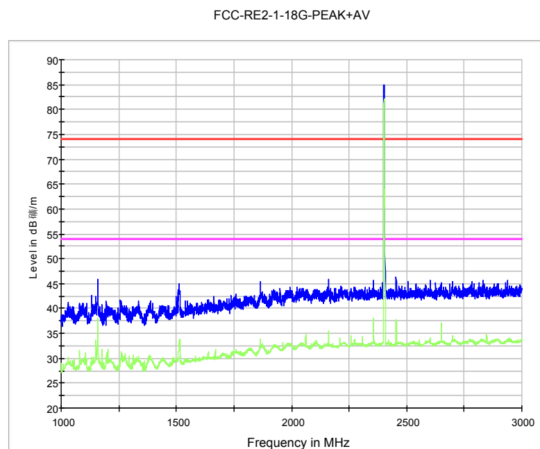
Fig. 64 Radiated Spurious Emission (8DPSK, Ch0, 1 GHz ~3 GHz)
