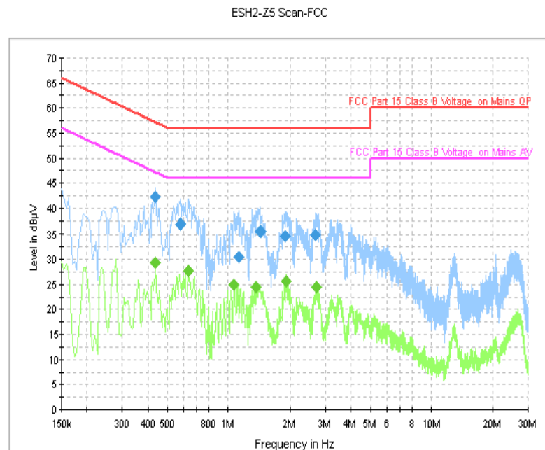
Fig. 101 AC Power line Conducted Emission (Traffic, AE3)
