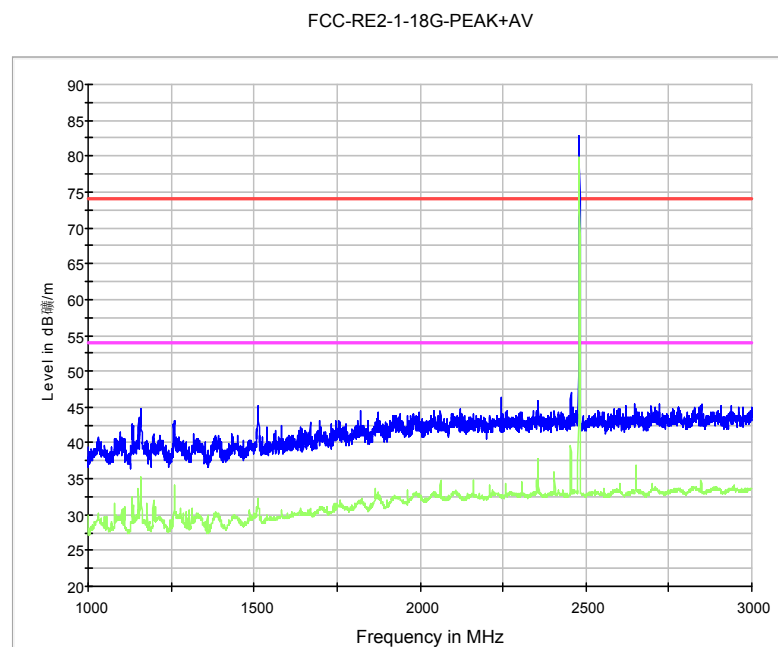
Fig. 70 Radiated Spurious Emission (8DPSK, Ch78, 1 GHz ~3 GHz)
