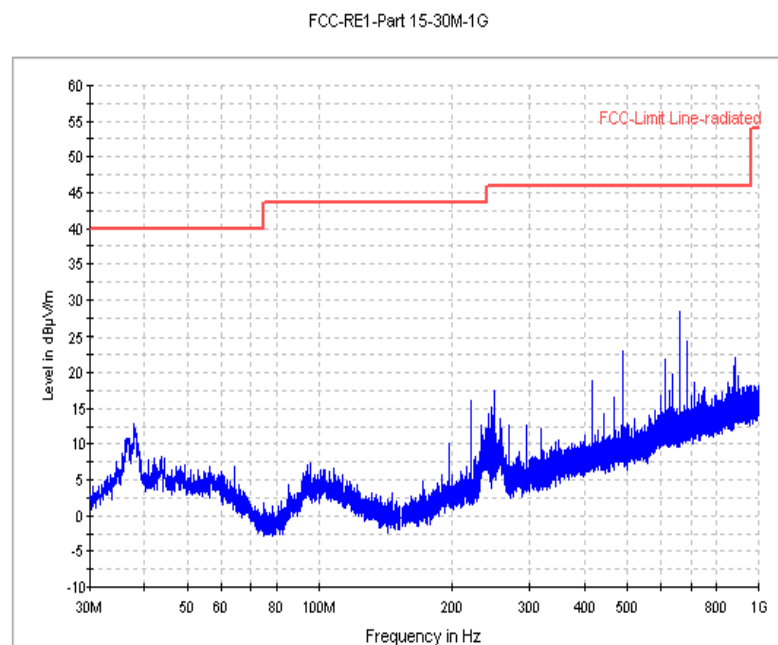
Fig. 66 Radiated Spurious Emission (8DPSK, Ch39, 30 MHz ~1 GHz)
