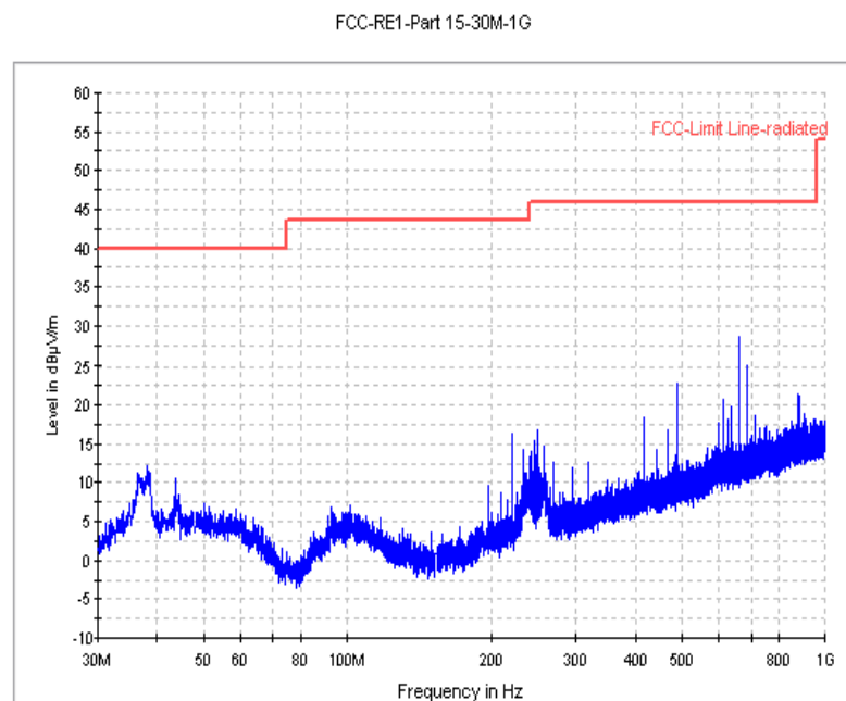
Fig. 44 Radiated Spurious Emission (GFSK, Ch39, 30 MHz ~1 GHz)
