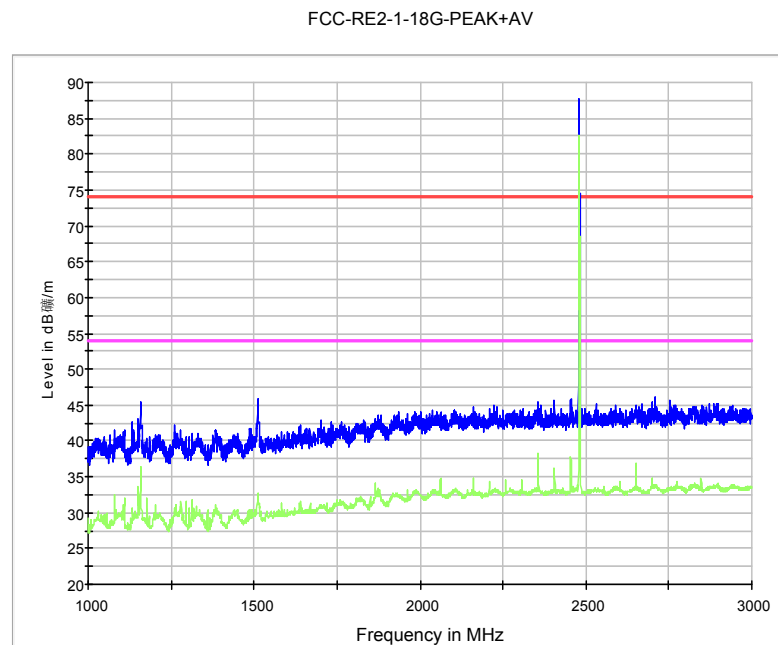
Fig. 48 Radiated Spurious Emission (GFSK, Ch78, 1 GHz ~3 GHz)
