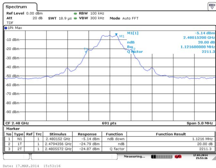
Fig. 77 Occupied 20dB Bandwidth (GFSK, Ch 78)
