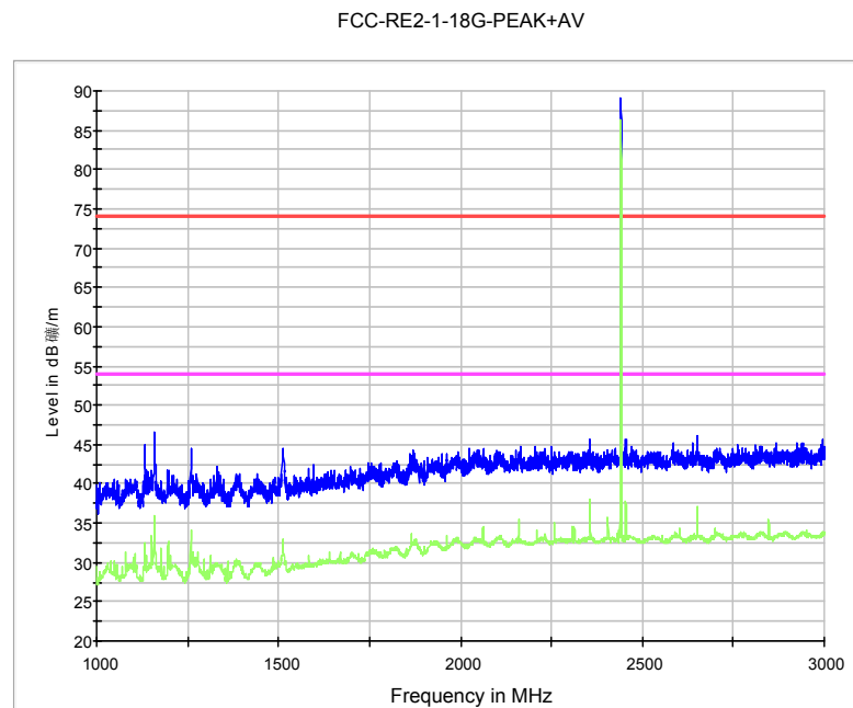
Fig. 67 Radiated Spurious Emission (8DPSK, Ch39, 1 GHz ~3 GHz)
