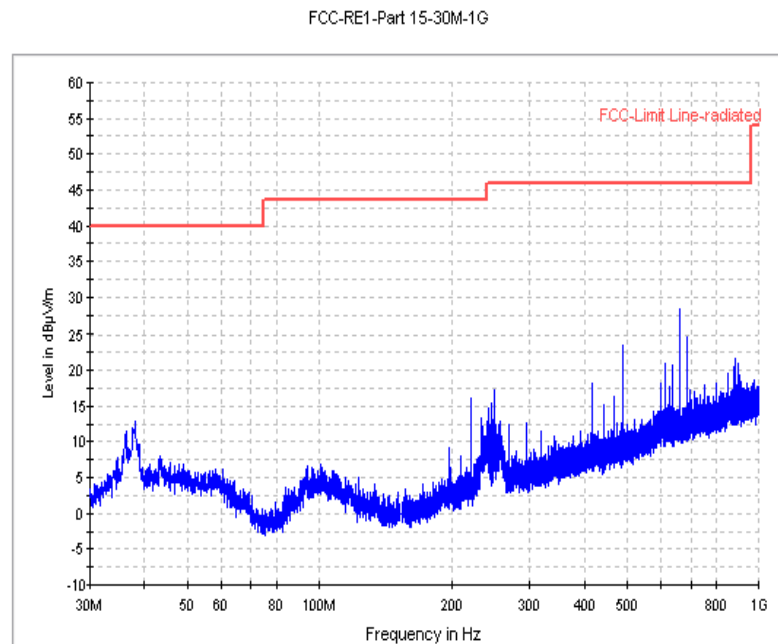
Fig. 63 Radiated Spurious Emission (8DPSK, Ch0, 30 MHz ~1 GHz)
