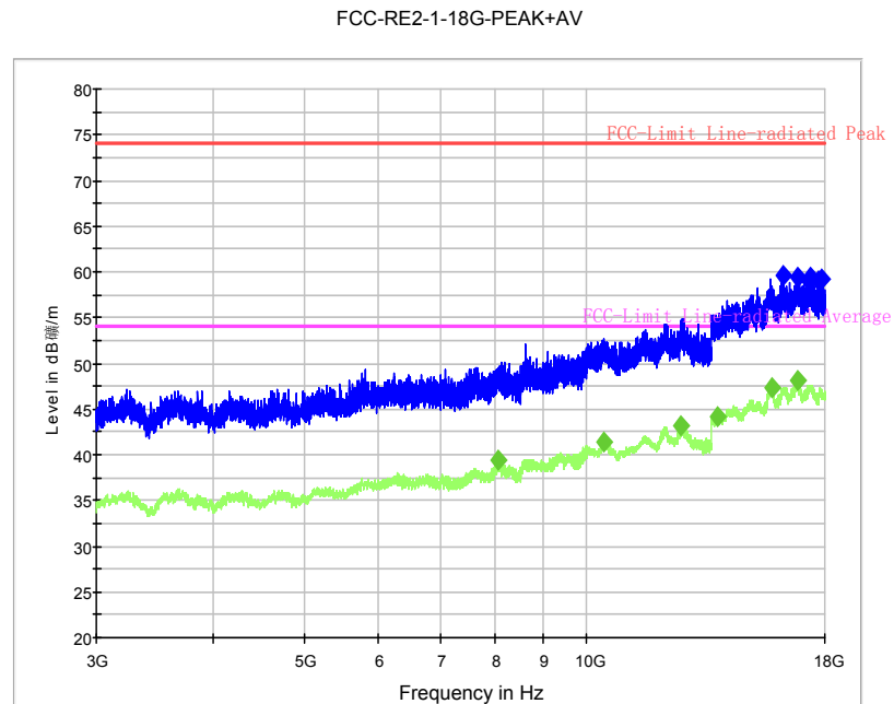
Fig. 57 Radiated Spurious Emission ( \pi/4 DQPSK, Ch39, 3 GHz ~18 GHz)
