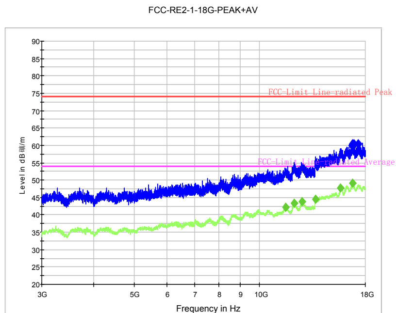
Fig. 71 Radiated Spurious Emission (8DPSK, Ch78, 3 GHz ~18 GHz)
