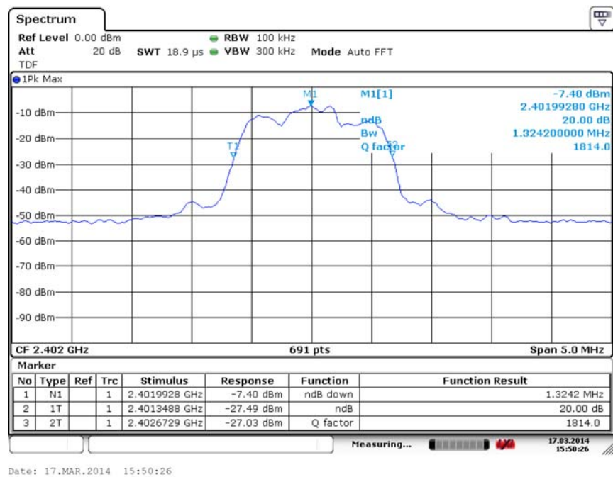
Fig. 81 Occupied 20dB Bandwidth (8DPSK, Ch 0)
