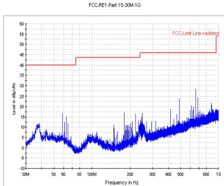
Fig. 55 Radiated Spurious Emission ( \pi/4 DQPSK, Ch39, 30 MHz ~1 GHz)
