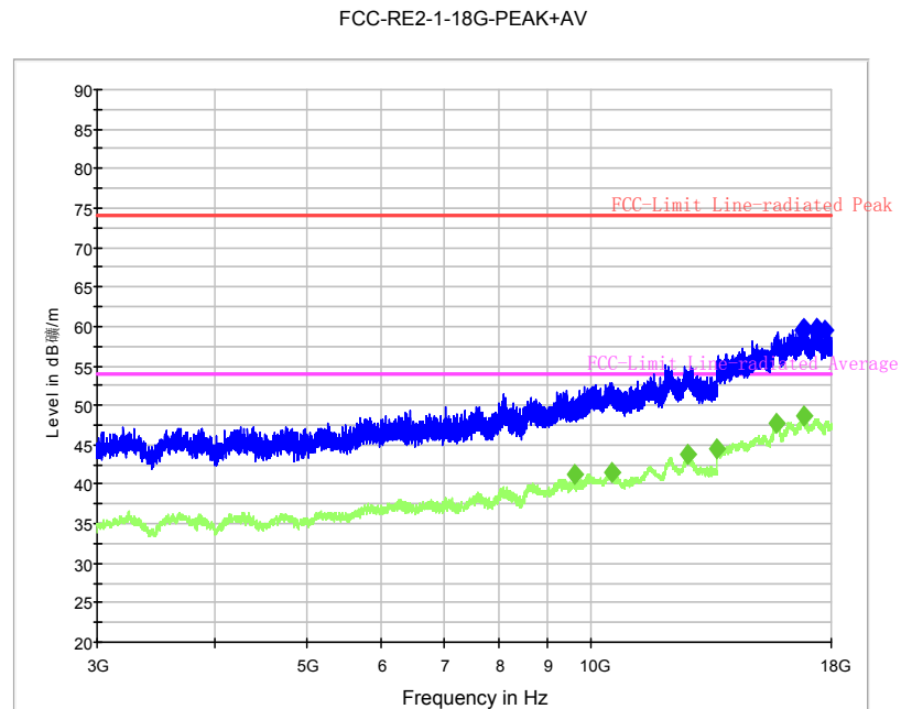
Fig. 65 Radiated Spurious Emission (8DPSK, Ch0, 3 GHz ~18 GHz)
