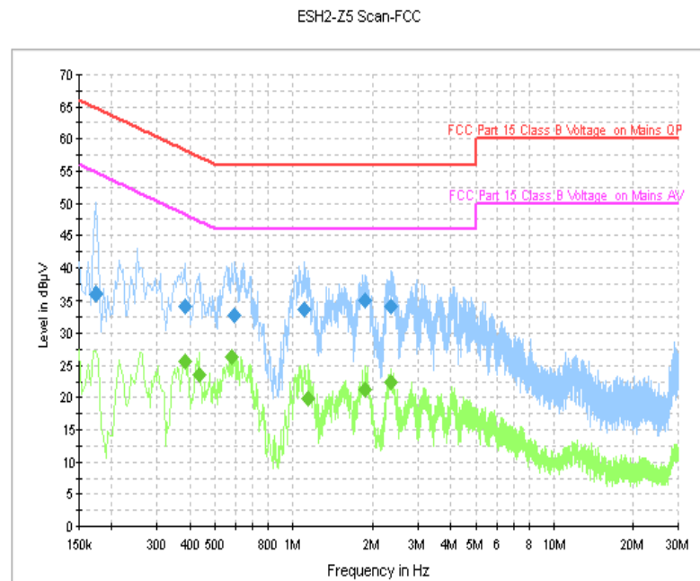
Fig. 99 AC Power line Conducted Emission (Traffic, AE2)
