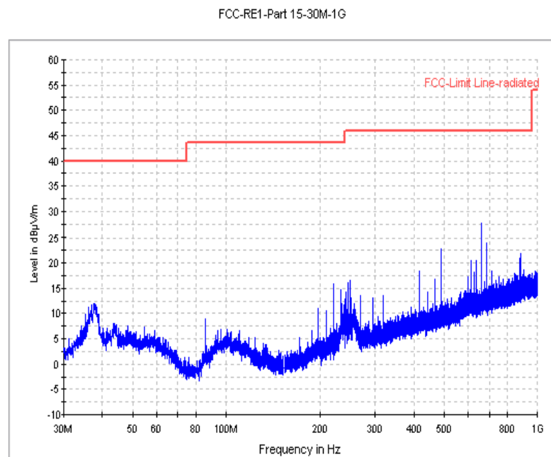
Fig. 47 Radiated Spurious Emission (GFSK, Ch78, 30 MHz ~1 GHz)
