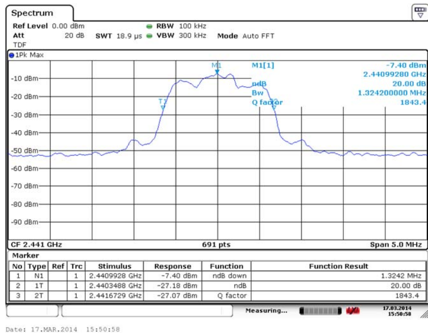
Fig. 82 Occupied 20dB Bandwidth (8DPSK, Ch 39)
