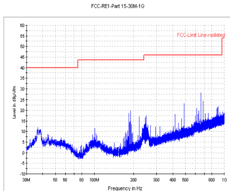
Fig. 58 Radiated Spurious Emission ( \pi/4 DQPSK, Ch78, 30 MHz ~1 GHz)
