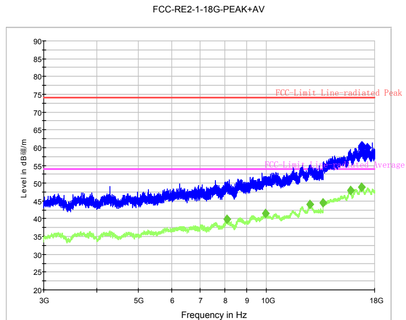
Fig. 54 Radiated Spurious Emission ( \pi/4 DQPSK, Ch0, 3 GHz ~18 GHz)
