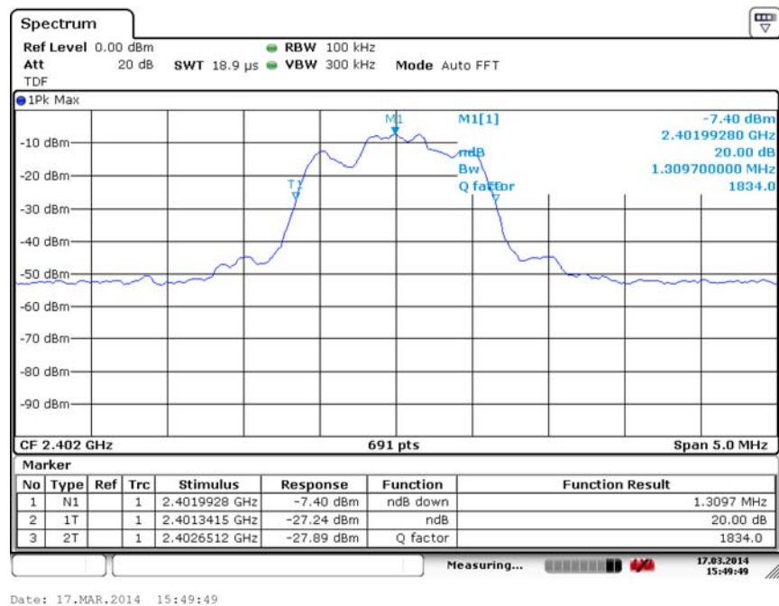
Fig. 78 Occupied 20dB Bandwidth ( \pi/4 DQPSK, Ch 0)
