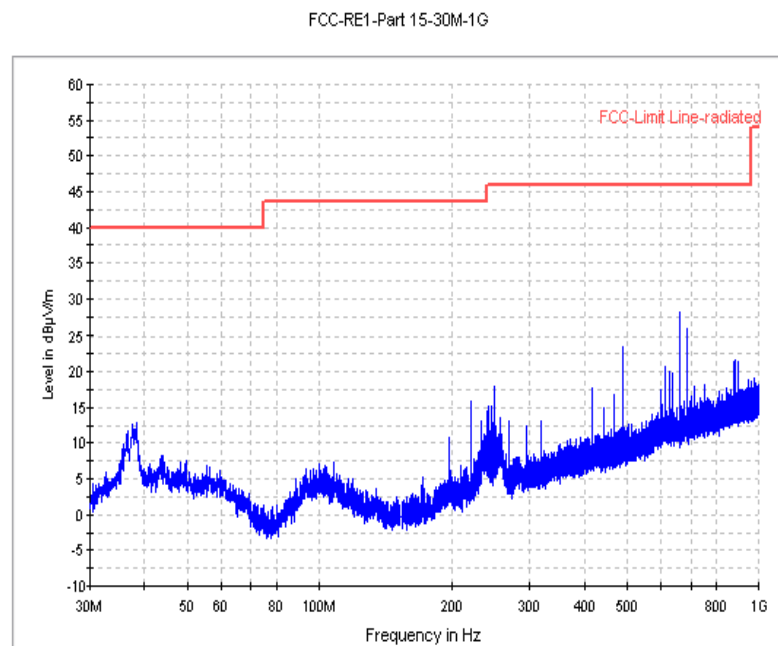
Fig. 69 Radiated Spurious Emission (8DPSK, Ch78, 30 MHz ~1 GHz)
