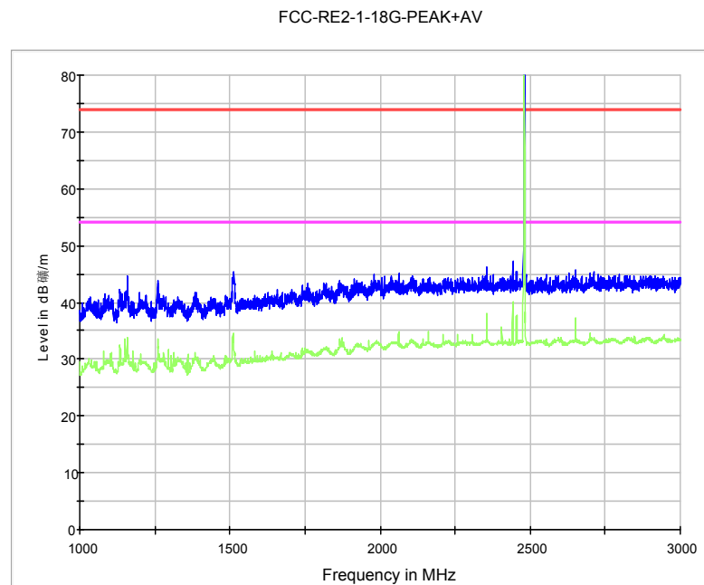
Fig. 45 Radiated Spurious Emission (GFSK, Ch39, 1 GHz ~3 GHz)
