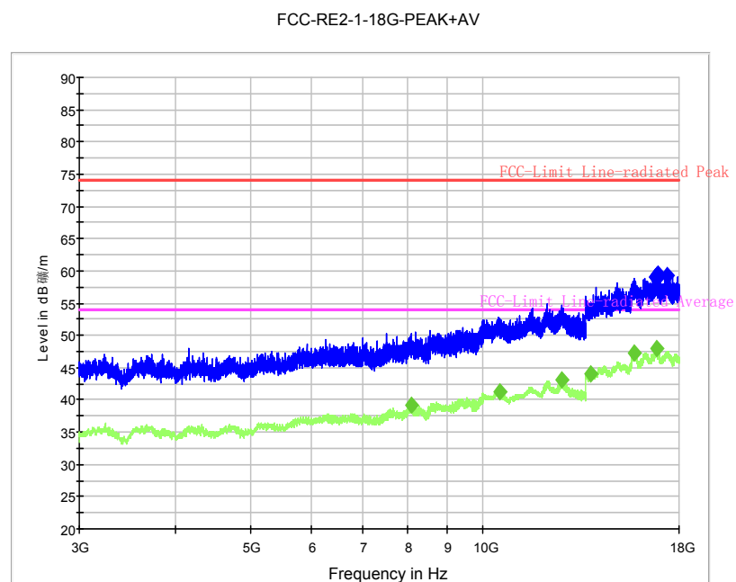
Fig. 60 Radiated Spurious Emission ( \pi/4 DQPSK, Ch78, 3 GHz ~18 GHz)
