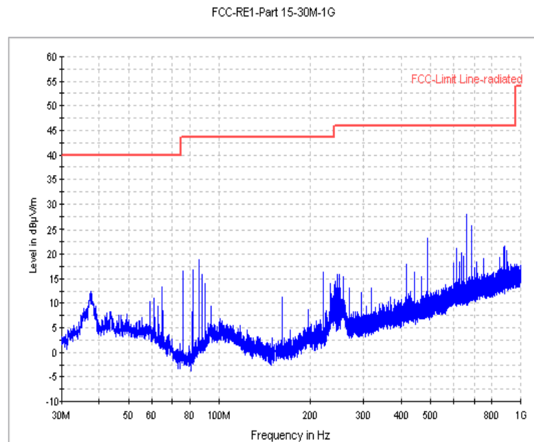
Fig. 41 Radiated Spurious Emission (GFSK, Ch0, 30 MHz ~1 GHz)
