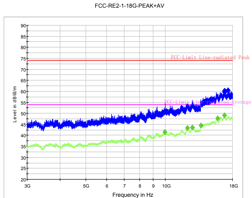
Fig. 68 Radiated Spurious Emission (8DPSK, Ch39, 3 GHz ~18 GHz)
