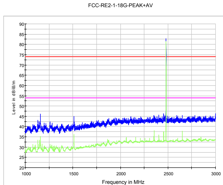
Fig. 59 Radiated Spurious Emission ( \pi/4 DQPSK, Ch78, 1 GHz ~3 GHz)
