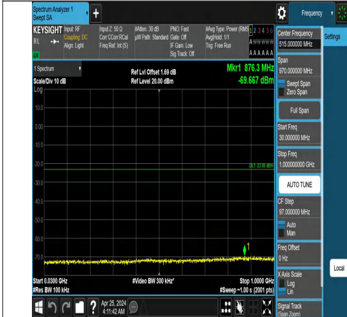
Band66_5MHz_QPSK_131997_1RB#0_30~1000_30~1000
