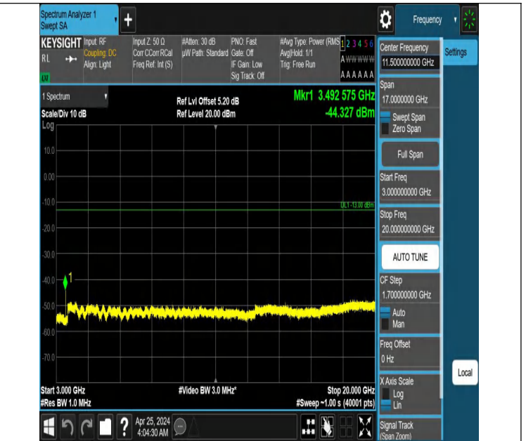
Band66_3MHz_QPSK_132322_1RB#14_3000~20000_3000~2000
