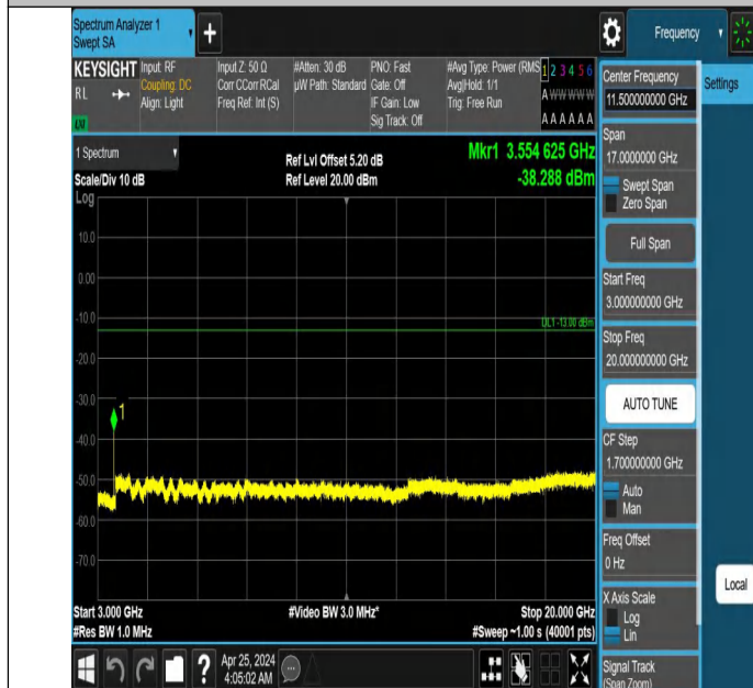
Band66_3MHz_QPSK_132657_1RB#0_3000~20000_3000~2000
