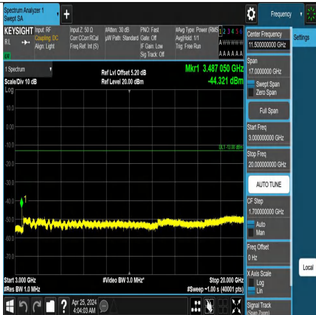
Band66_3MHz_QPSK_132322_1RB#0_3000~20000_3000~2000 0
