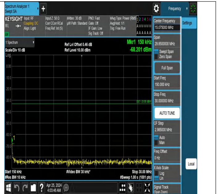
Band66_3MHz_QPSK_132322_1RB#0_0.15~30_0.15~30
