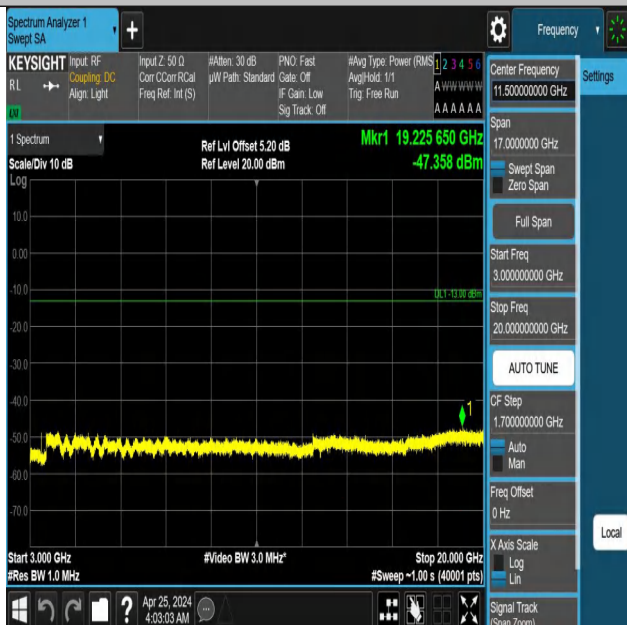
Band66_3MHz_QPSK_131987_1RB#0_3000~20000_3000~2000
