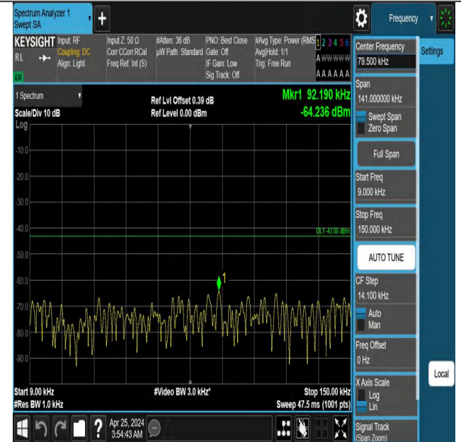
Band66_1.4MHz_QPSK_132322_1RB#5_0.009~0.15_0.009~0.15
