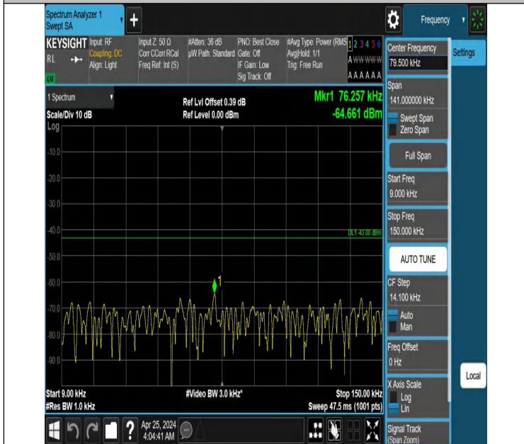
Band66_3MHz_QPSK_132657_1RB#0_0.009~0.15_0.009~0.15
