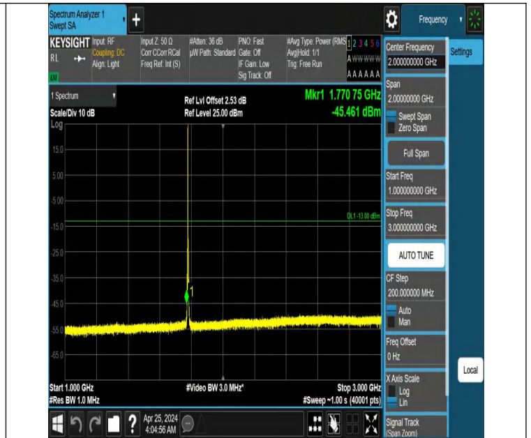
Band66_3MHz_QPSK_132657_1RB#0_1000~3000_1000~3000
