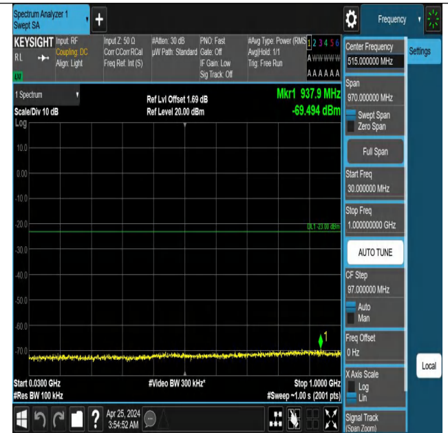
Band66_1.4MHz_QPSK_132322_1RB#5_30~1000_30~1000
