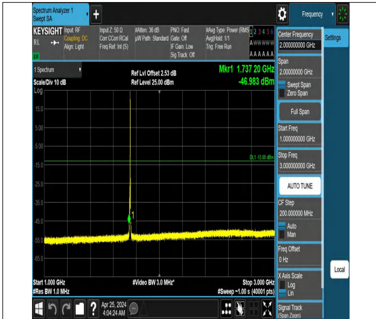
Band66_3MHz_QPSK_132322_1RB#14_1000~3000_1000~3000
