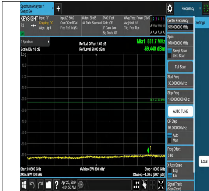
Band66_3MHz_QPSK_132657_1RB#0_30~1000_30~1000
