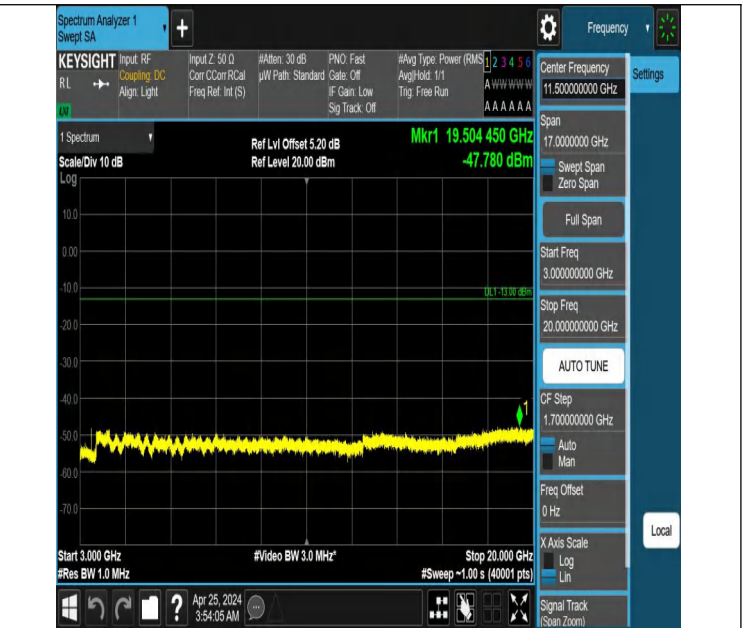
Band66_1.4MHz_QPSK_131979_1RB#5_3000~20000_3000~20000
