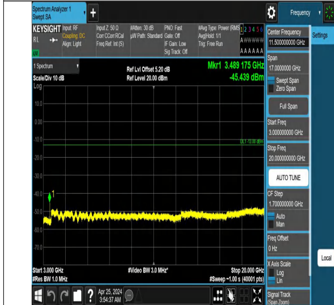
Band66_1.4MHz_QPSK_132322_1RB#0_3000~20000_3000~2000
