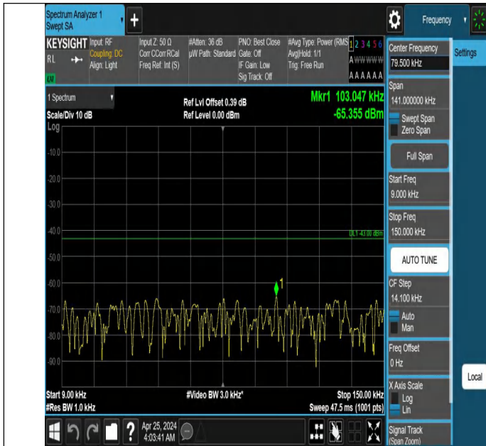
Band66_3MHz_QPSK_132322_1RB#0_0.009~0.15_0.009~0.15
