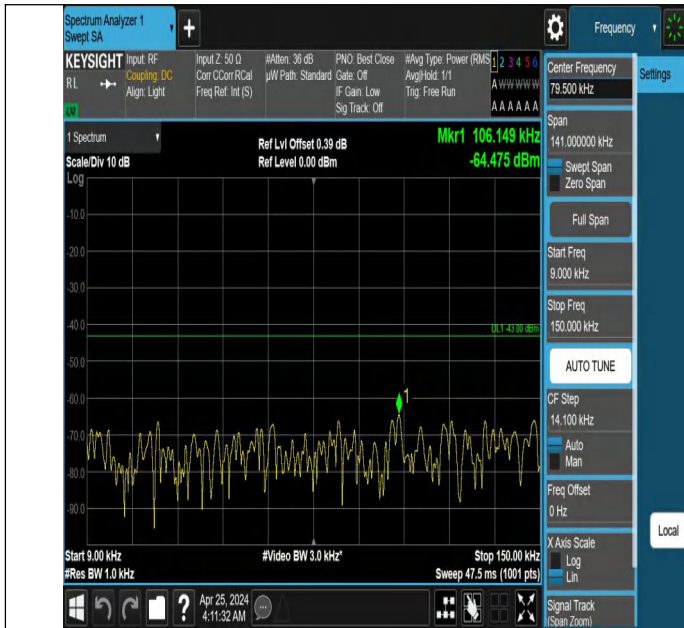
Band66_5MHz_QPSK_131997_1RB#0_0.009~0.15_0.009~0.15
