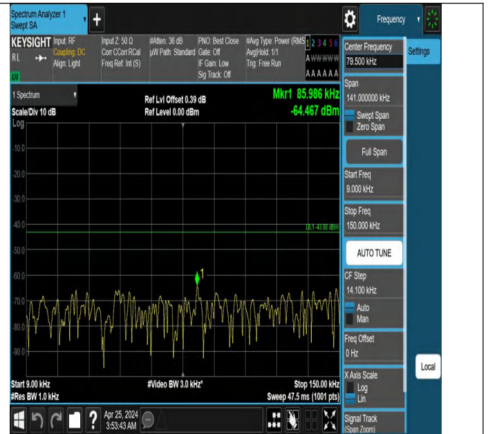
Band66_1.4MHz_QPSK_131979_1RB#5_0.009~0.15_0.009~0.15
