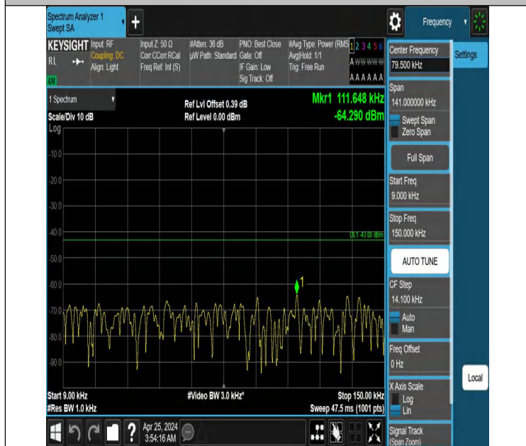
Band66_1.4MHz_QPSK_132322_1RB#0_0.009~0.15_0.009~0.15
