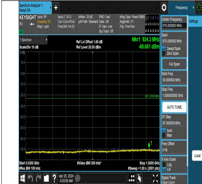
Band66_3MHz_QPSK_132322_1RB#0_30~1000_30~1000
