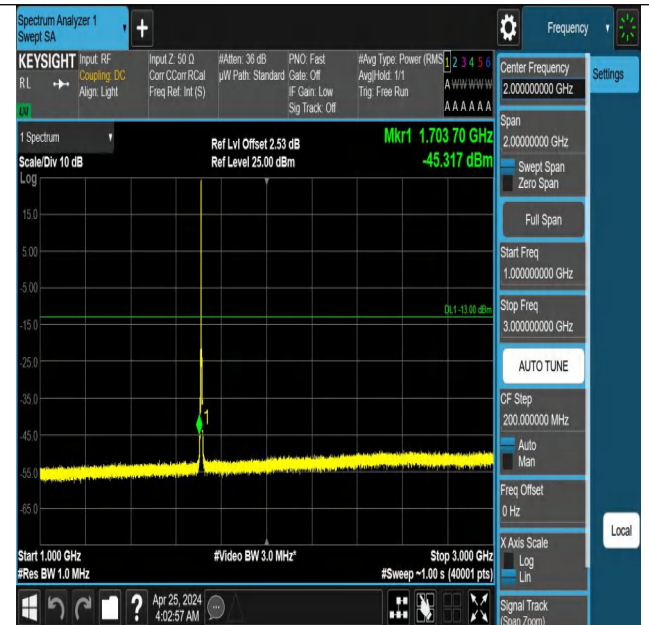
Band66_3MHz_QPSK_131987_1RB#0_1000~3000_1000~3000
