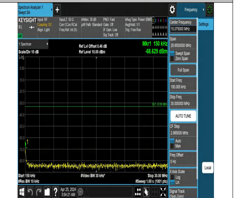
Band66_1.4MHz_QPSK_132322_1RB#0_0.15~30_0.15~30
