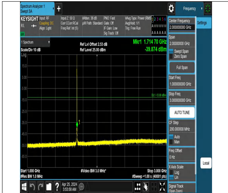
Band66_1.4MHz_QPSK_131979_1RB#5_1000~3000_1000~3000
