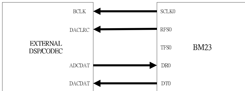
FIGURE 2-9: MASTER MODE REFERENCE CONNECTION
