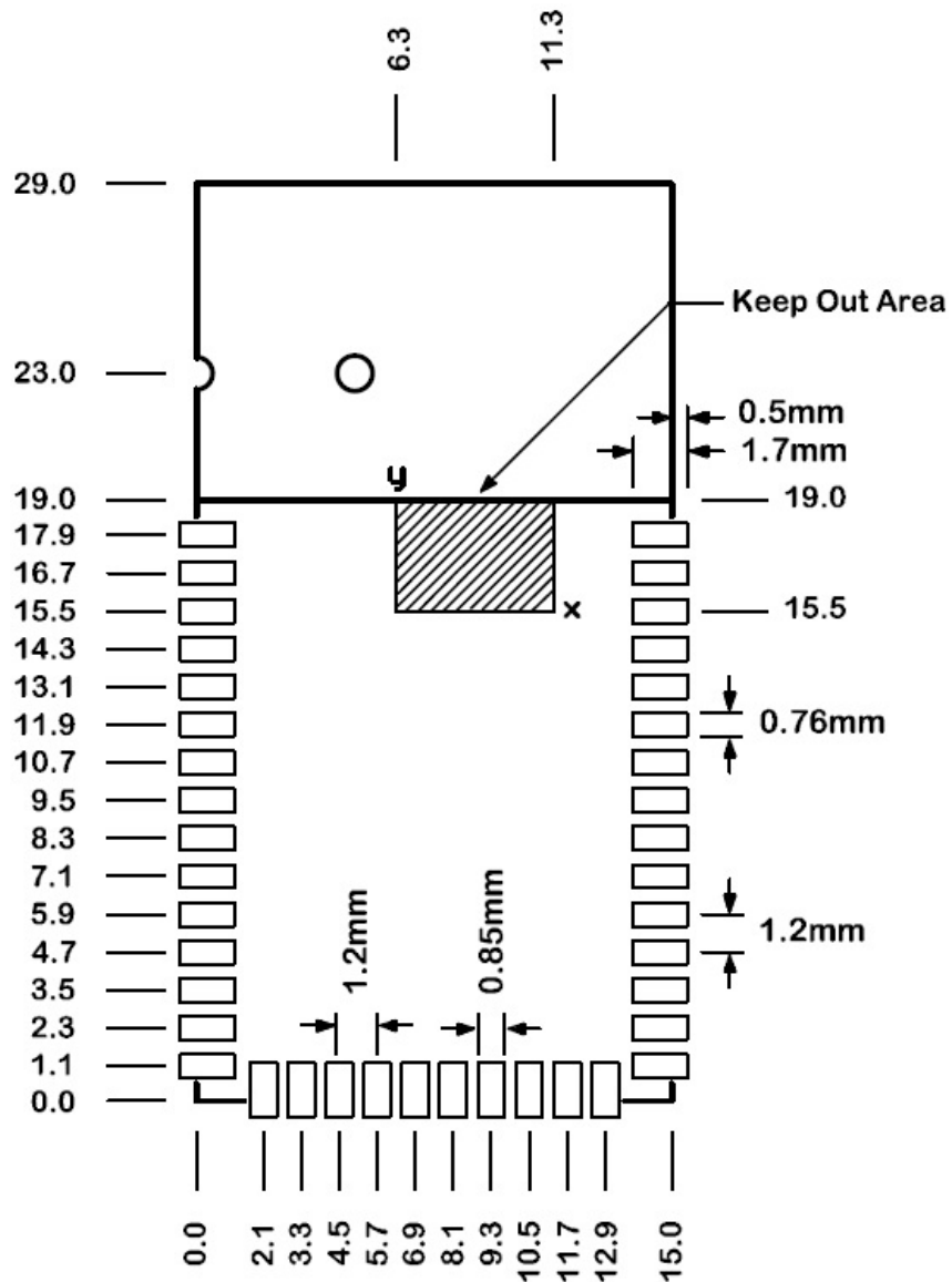
FIGURE 7-4: BM23 PCB FOOT PRINT
