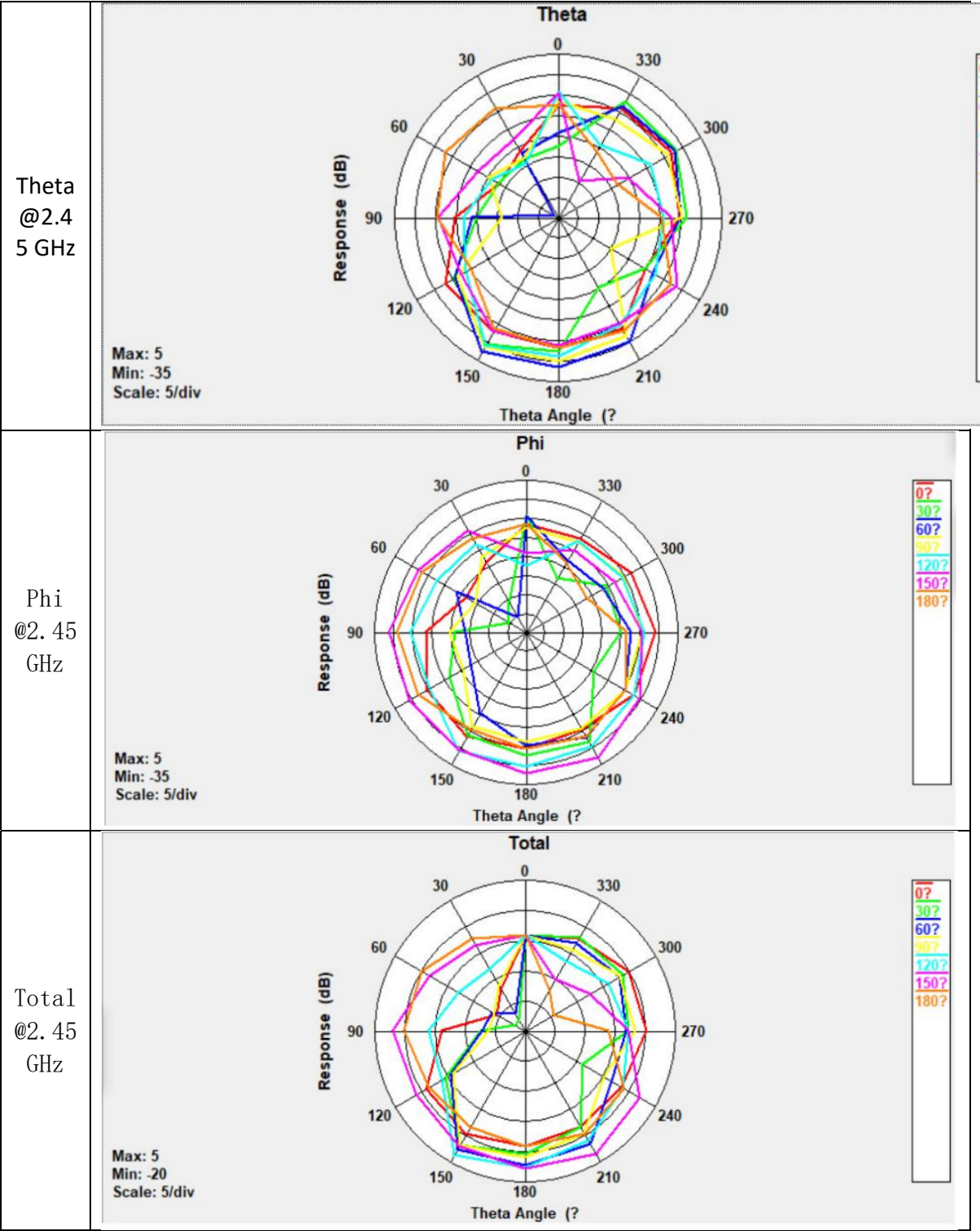
Antenna Pattern/Gain Measurement data/Table:
