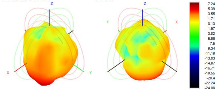
5520.0MHz H+V, Eff: 62.8%
