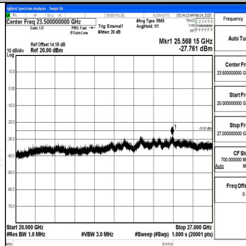
Band38_15MHz_QPSK_38000_1RB#0_20000~27000_20000~27000
