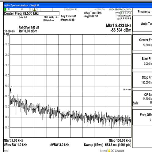
Band38_15MHz_16QAM_38000_1RB#0_0.009~0.15_0.009~0.15
