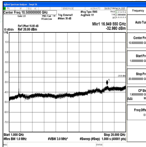
Band38_15MHz_QPSK_38000_1RB#0_1000~20000_1000~20000
