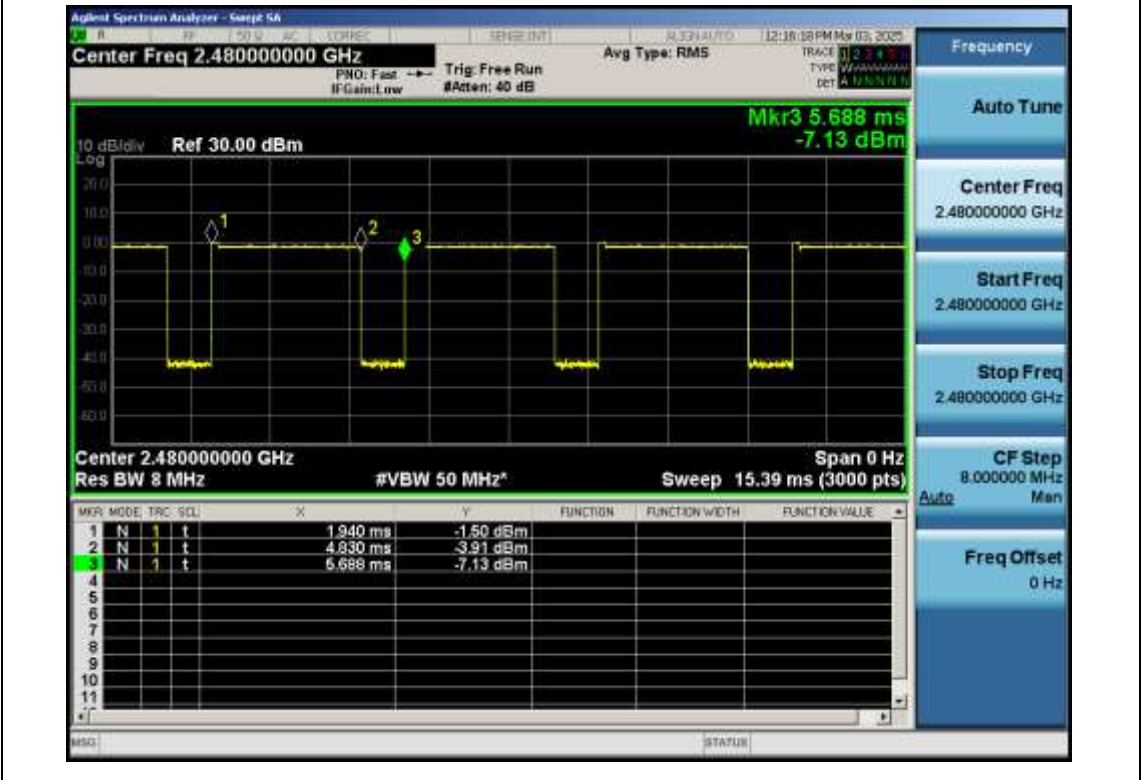
EDR-π /4-DQPSK-Ant1-2480
