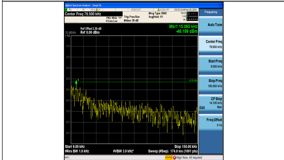
Band4_5MHz_QPSK_19975_25RB#0_0.009~0.15_0.009~0.15
