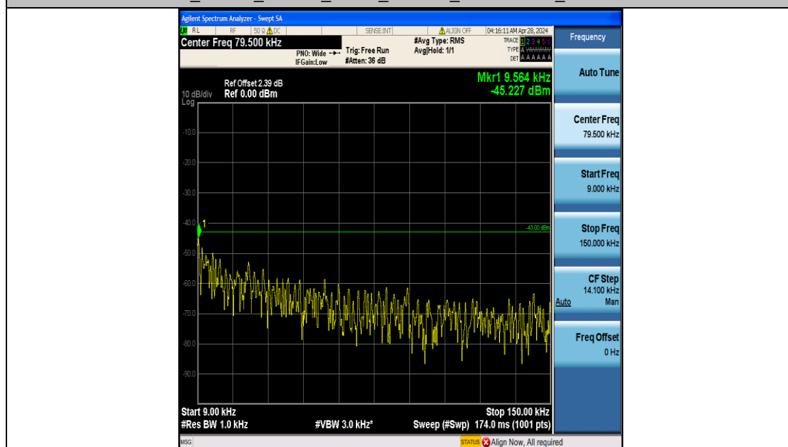
Band4_15MHz_QPSK_20175_75RB#0_0.009~0.15_0.009~0.15
