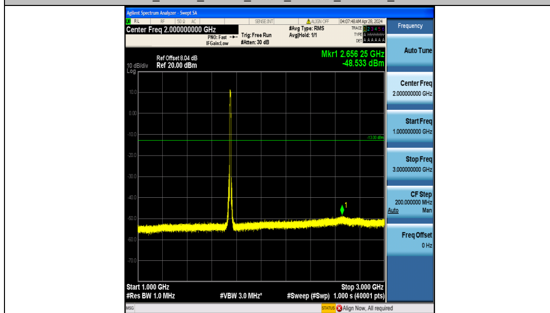
Band4_10MHz_16QAM_20350_50RB#0_1000~3000_1000~3000
