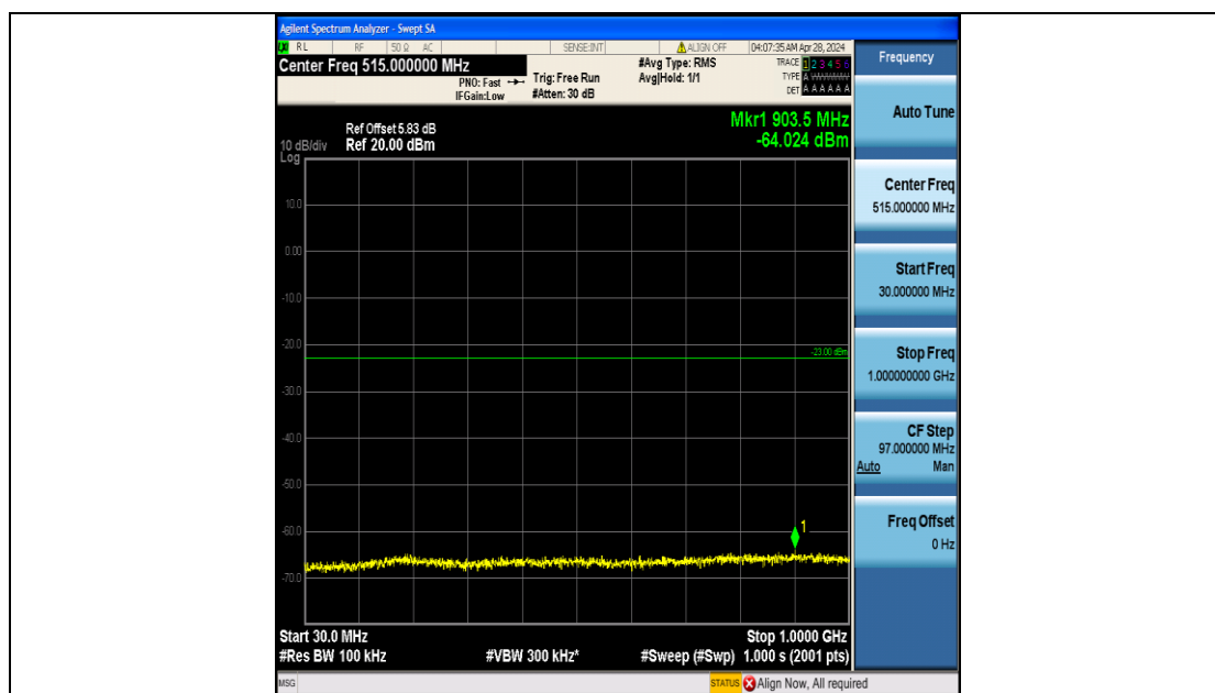
Band4_10MHz_16QAM_20350_50RB#0_30~1000_30~1000
