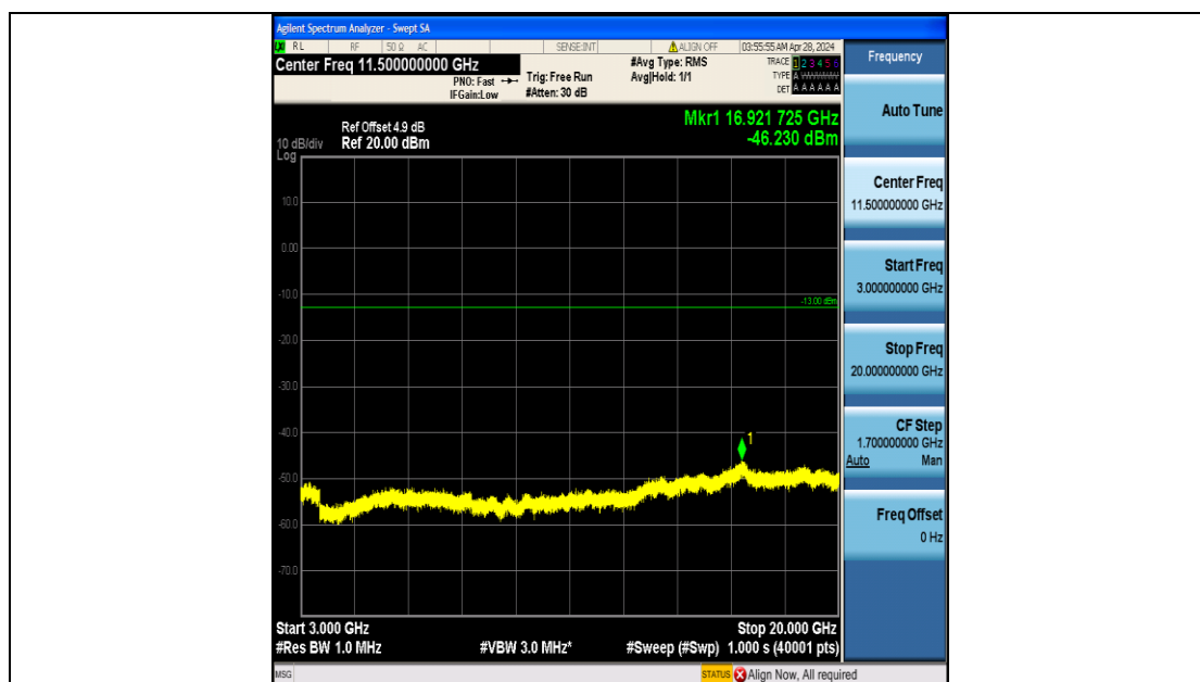
Band4_5MHz_16QAM_20175_25RB#0_3000~20000_3000~20000
