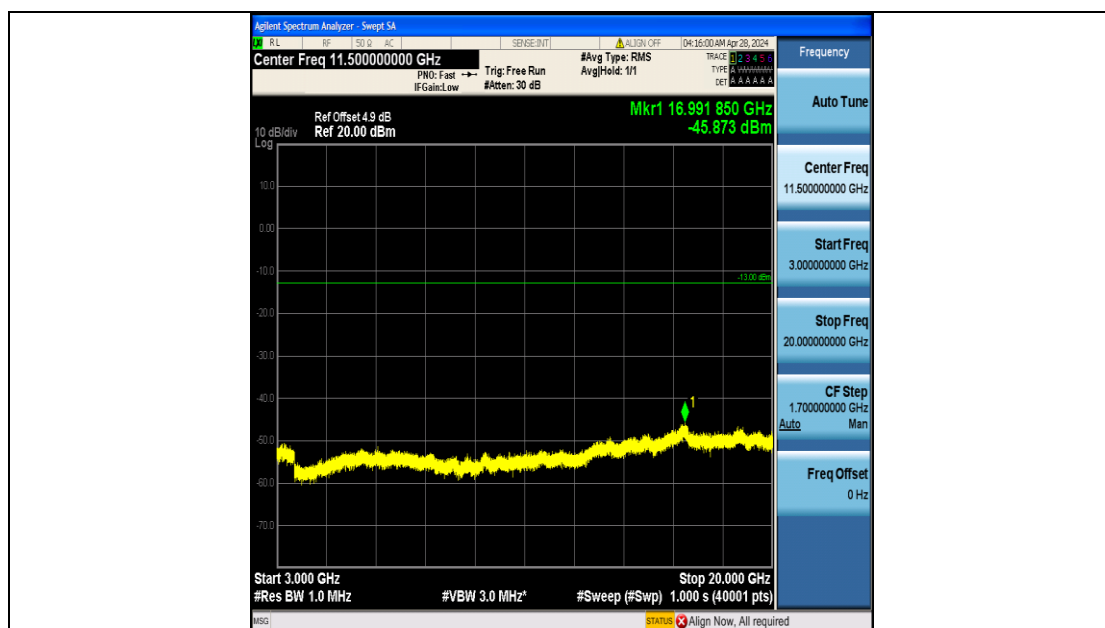
Band4_15MHz_16QAM_20025_75RB#0_3000~20000_3000~20000
