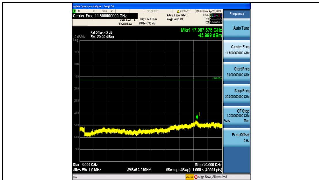
Band4_3MHz_16QAM_20385_15RB#0_3000~20000_3000~20000
