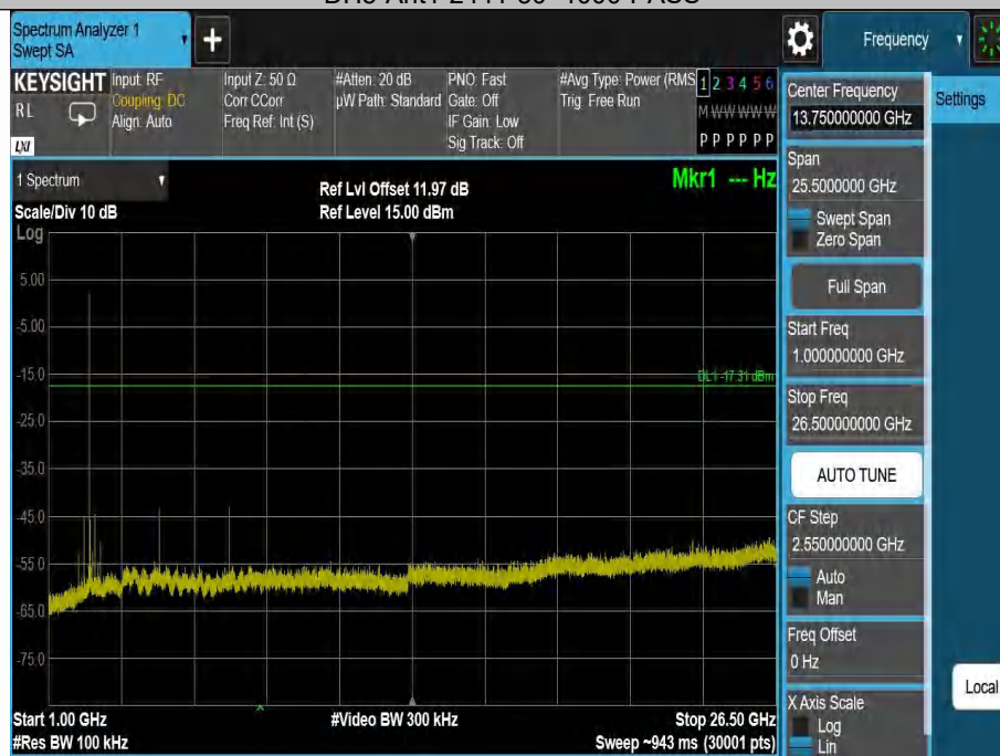
DH5-Ant1-2441-1000~26500-PASS
