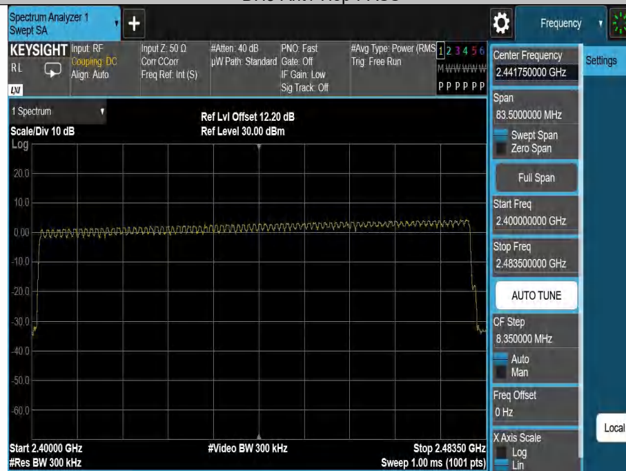
2DH5-Ant1-Hop-PASS
