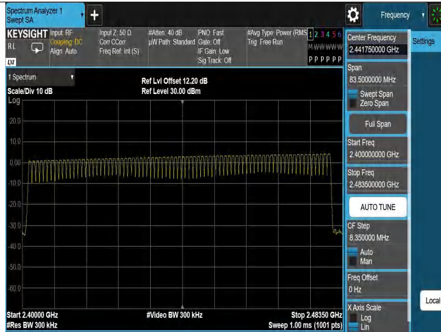
DH5-Ant1-Hop-PASS
