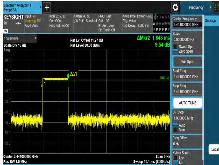
2DH3-Ant1-Hop-PASS
