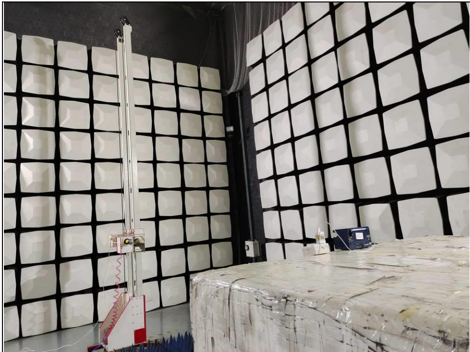
Above 1GHz
