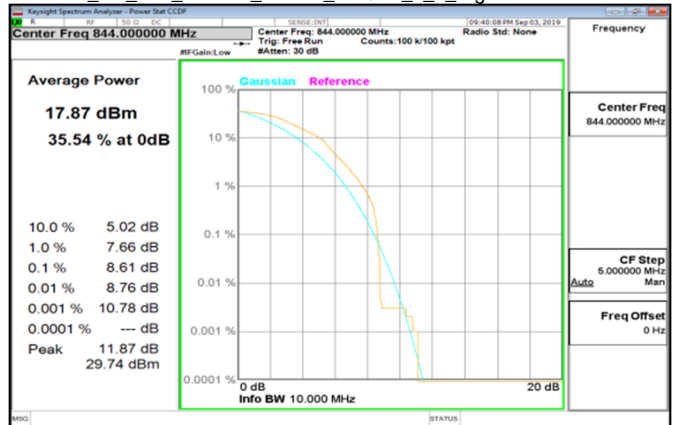
Cat_M1_LTE_Band26_10MHz_16QAM_6_0_HighCH26990-844
