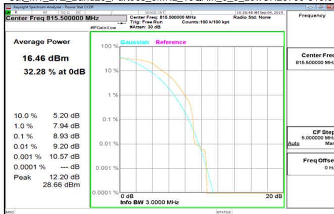
Cat_M1_LTE_Band26_Part90s_3MHz_16QAM_6_0_LowCH26705-815.5
