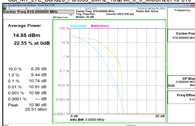
Cat_M1_LTE_Band26_Part90s_3MHz_16QAM_6_0_MidCH26740-819
