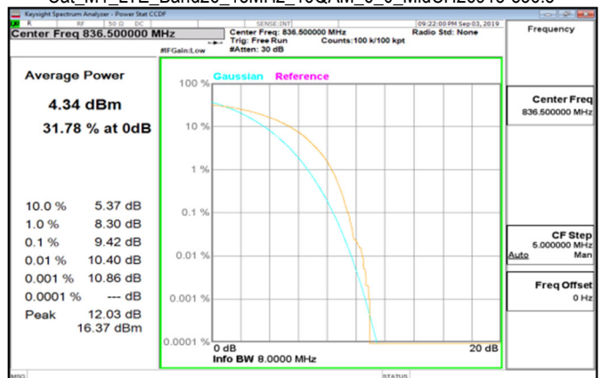
Cat_M1_LTE_Band26_15MHz_16QAM_6_0_MidCH26915-836.5
