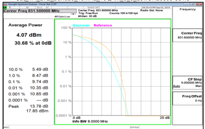
Cat_M1_LTE_Band26_15MHz_16QAM_6_0_LowCH26865-831.5
