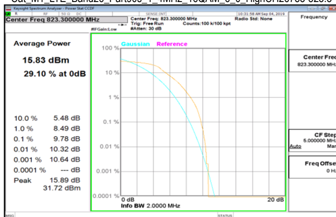
Cat_M1_LTE_Band26_Part90s_1_4MHz_16QAM_6_0_HighCH26783-823.3
