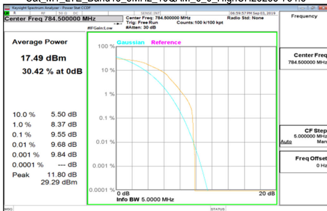
Cat_M1_LTE_Band13_5MHz_16QAM_6_0_HighCH23255-784.5
