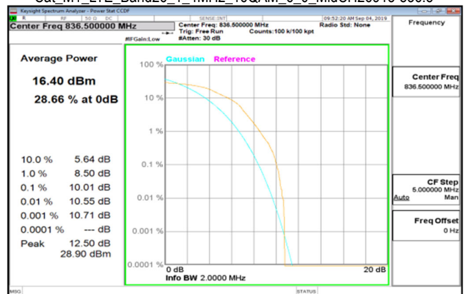
Cat_M1_LTE_Band26_1_4MHz_16QAM_6_0_MidCH26915-836.5
