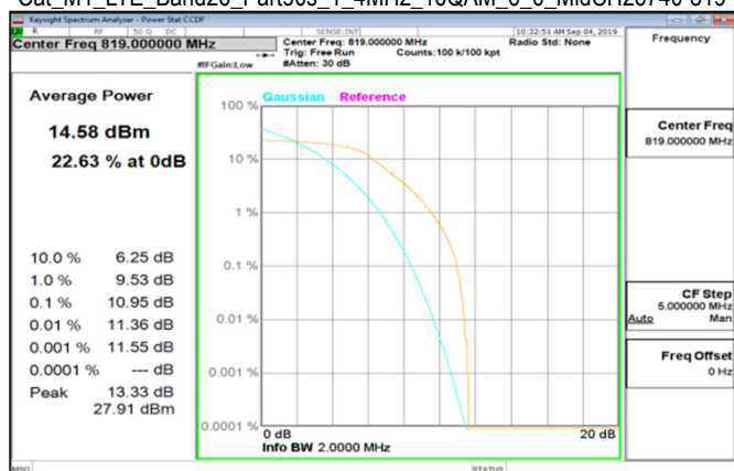
Cat_M1_LTE_Band26_Part90s_1_4MHz_16QAM_6_0_MidCH26740-819
