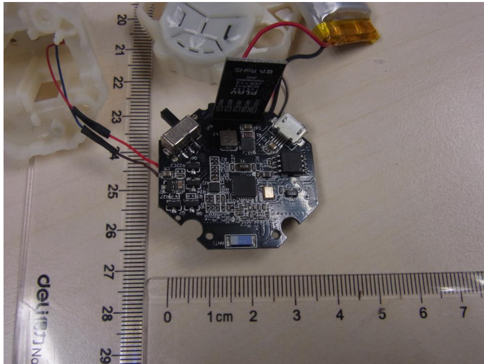
Fig. 3: Internal view
