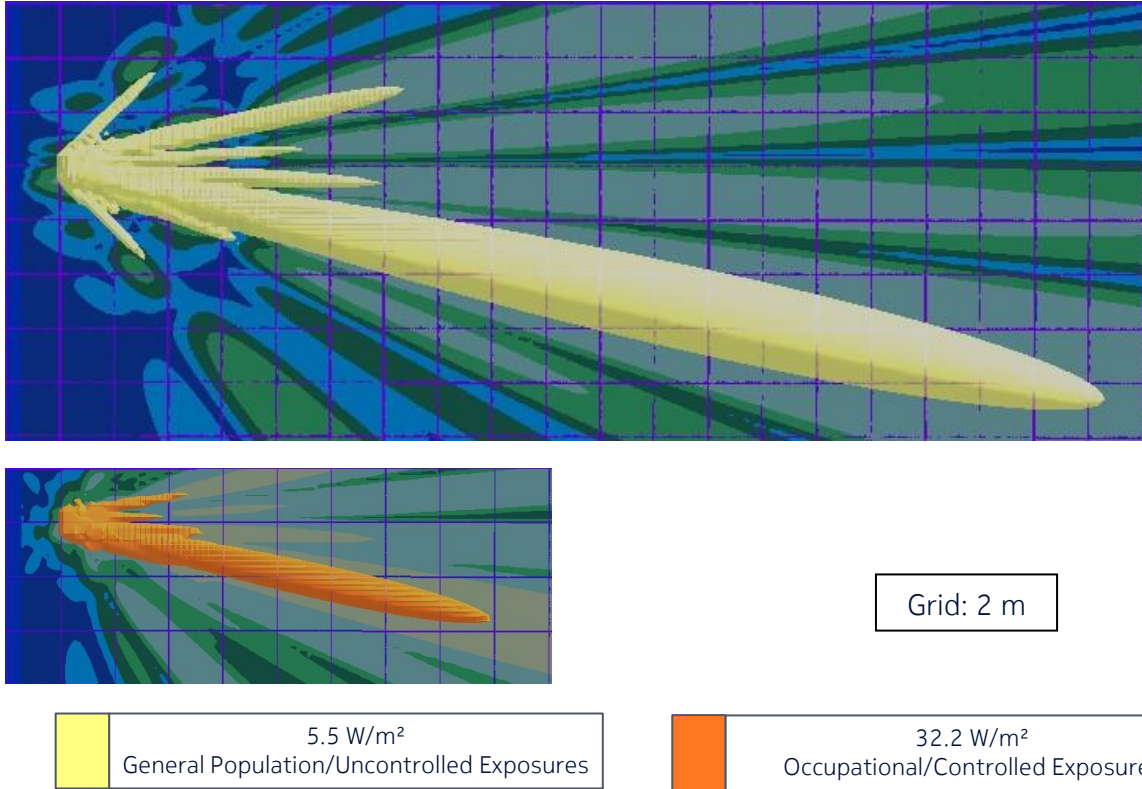
Figure 14 – Side view of the power density for the time-averaged maximum transmitted power of 424 W and beam oriented in azimuth = +3° & elevation = +13° with a gain of 24.0 dBi (Canada)
