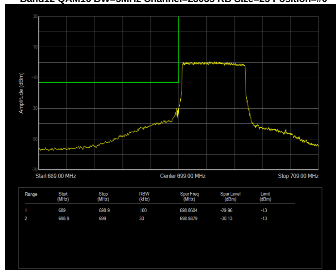
Band12 QAM16 BW=5MHz Channel=23035 RB Size=25 Position=#0
