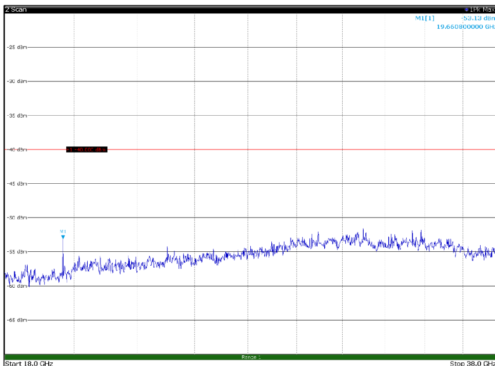
Channel: BOTTOM, Modulation: 64QAM, BW=15MHz, Range: 18GHz - 38GHz, Polarization: Horizontal
