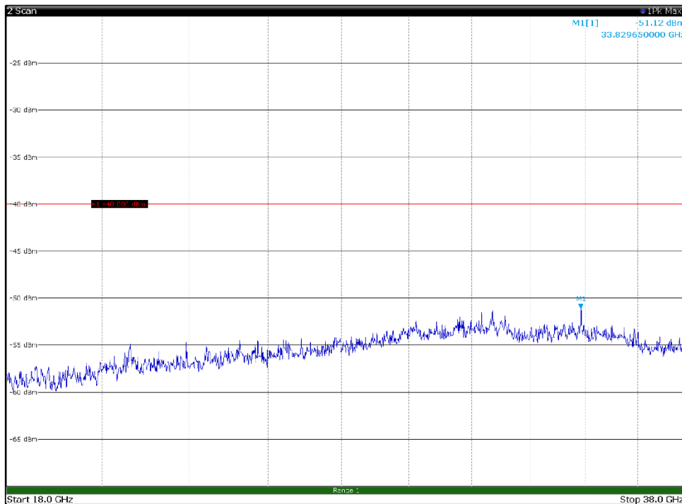
Channel: TOP, Modulation: 64QAM, BW=10MHz, Range: 18GHz - 38GHz, Polarization: Vertical
