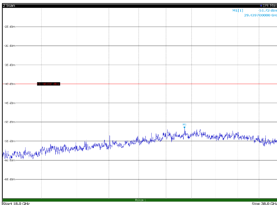
Channel: BOTTOM, Modulation: 64QAM, BW=15MHz, Range: 18GHz - 38GHz, Polarization: Vertical
