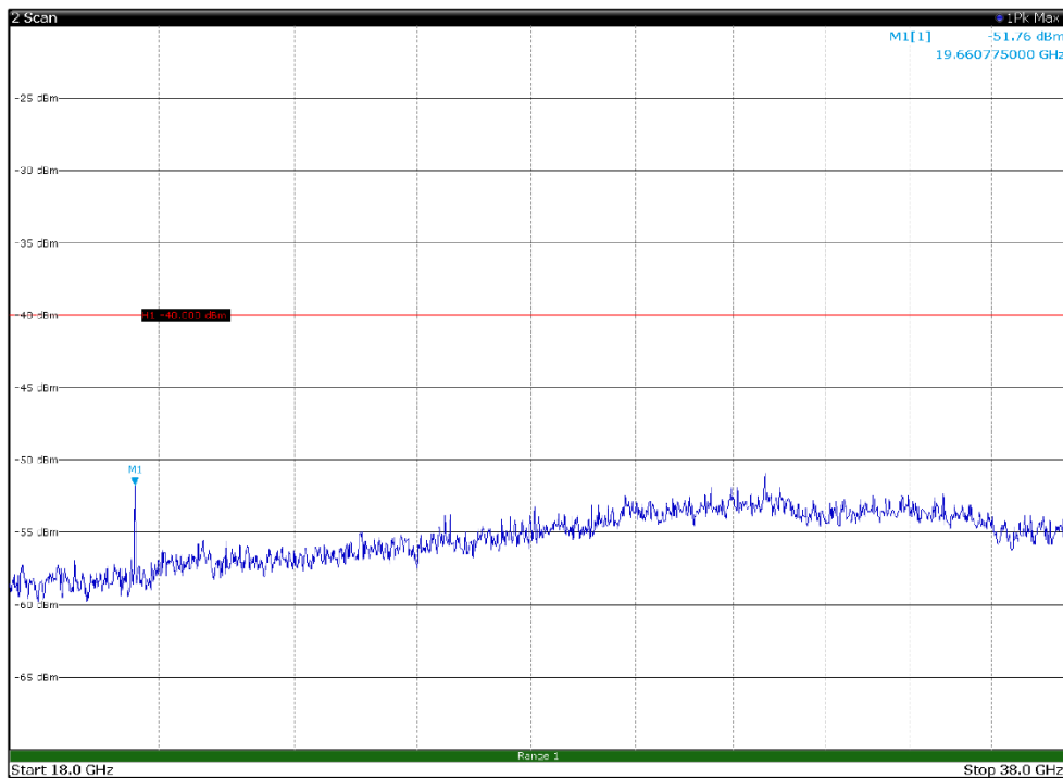
Channel: TOP, Modulation: 16QAM, BW=20MHz, Range: 18GHz - 38GHz, Polarization: Horizontal
