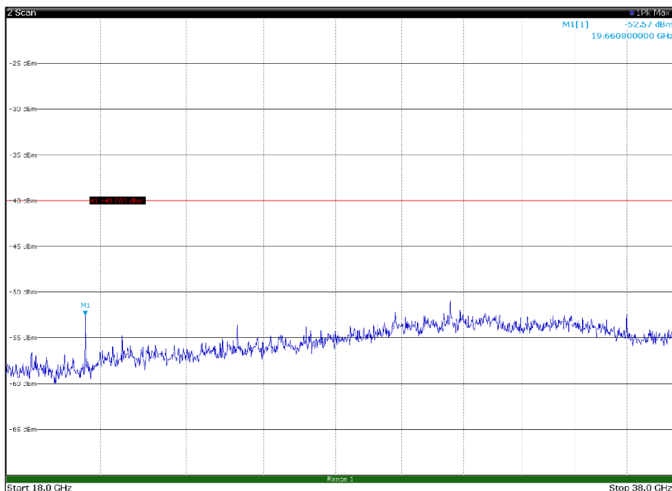
Channel: BOTTOM, Modulation: QPSK, BW=20MHz, Range: 18GHz - 38GHz, Polarization: Horizontal
