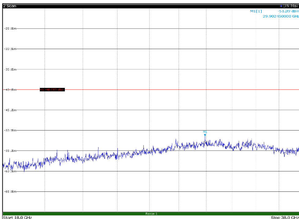
Channel: BOTTOM, Modulation: QPSK, BW=20MHz, Range: 18GHz - 38GHz, Polarization: Vertical
