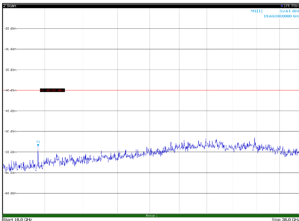
Channel: BOTTOM, Modulation: 256QAM, BW=10MHz, Range: 18GHz - 38GHz, Polarization: Horizontal
