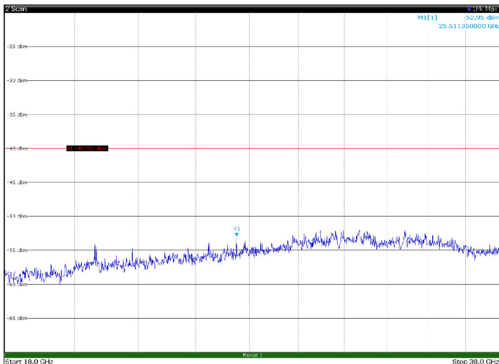
Channel: TOP, Modulation: 16QAM, BW=20MHz, Range: 18GHz - 38GHz, Polarization: Vertical
