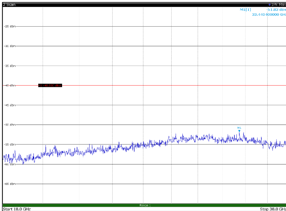
Channel: TOP, Modulation: 64QAM, BW=15MHz, Range: 18GHz - 38GHz, Polarization: Vertical
