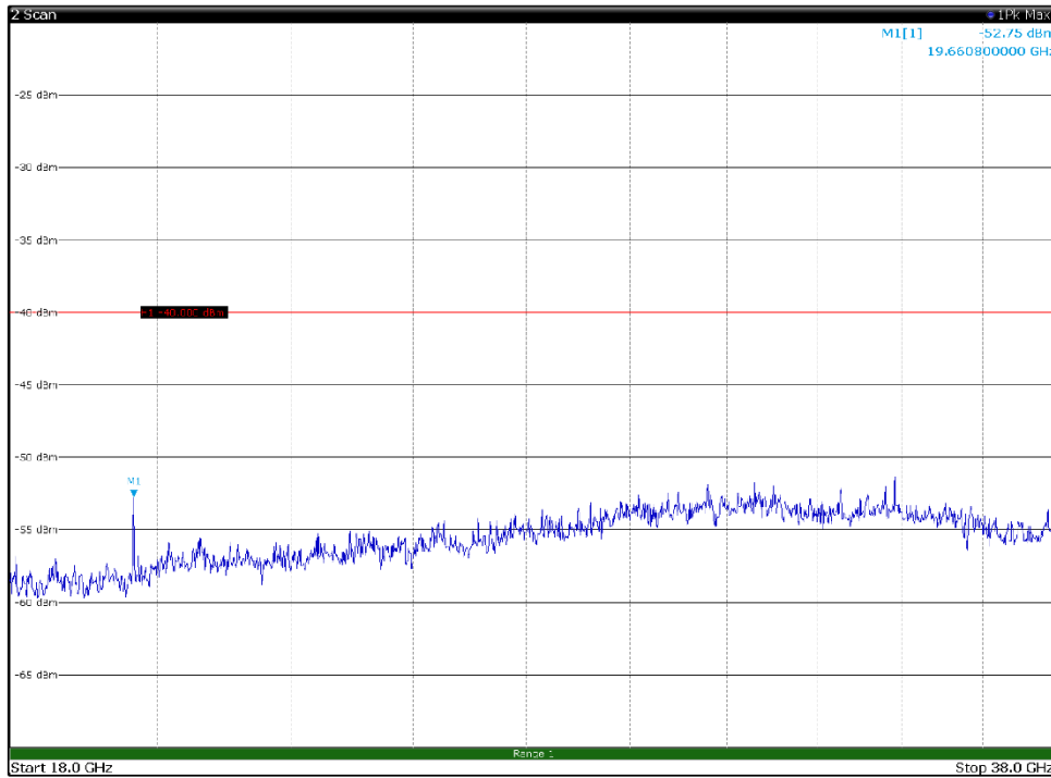
Channel: TOP, Modulation: 64QAM, BW=10MHz, Range: 18GHz - 38GHz, Polarization: Horizontal
