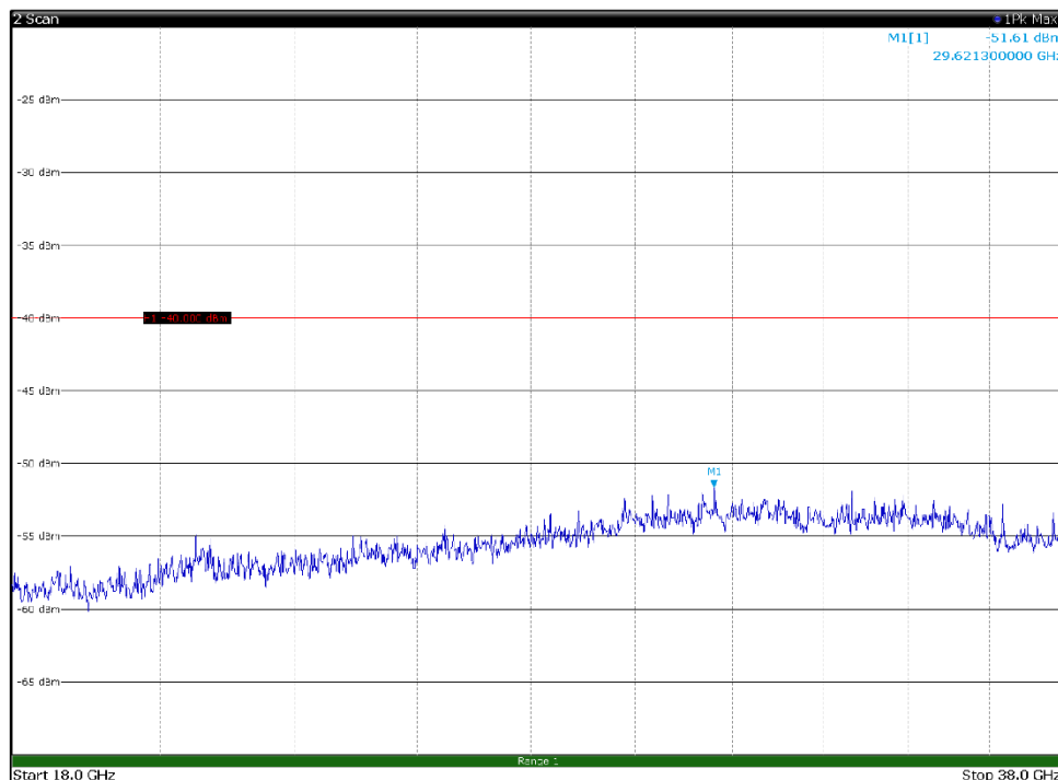
Channel: TOP, Modulation: 16QAM, BW=15MHz, Range: 18GHz - 38GHz, Polarization: Vertical
