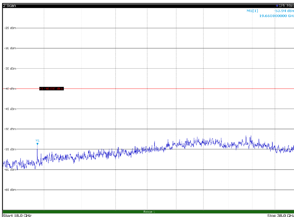
Channel: TOP, Modulation: 256QAM, BW=15MHz, Range: 18GHz - 38GHz, Polarization: Horizontal
