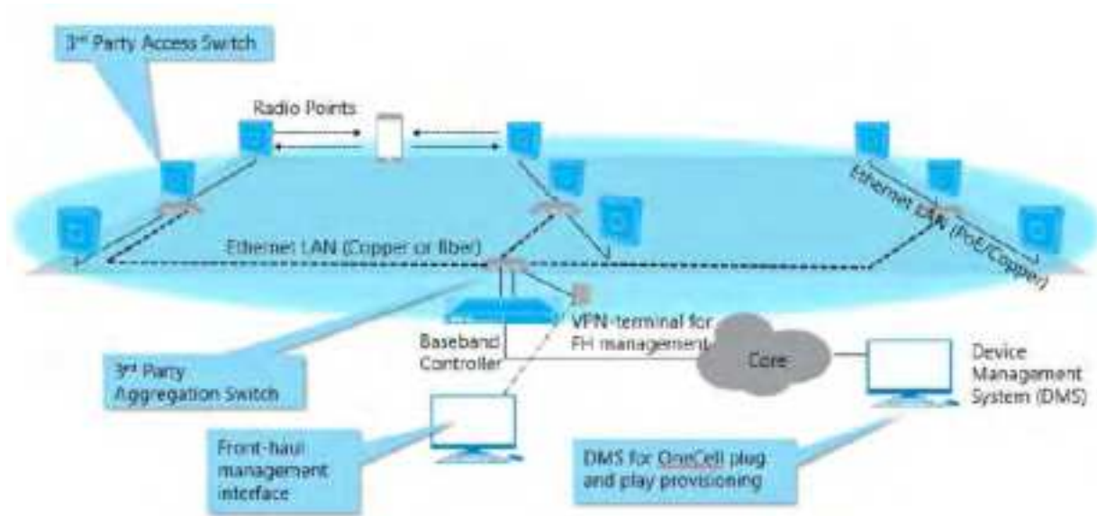
Figure 1-1. ONECELL solution
