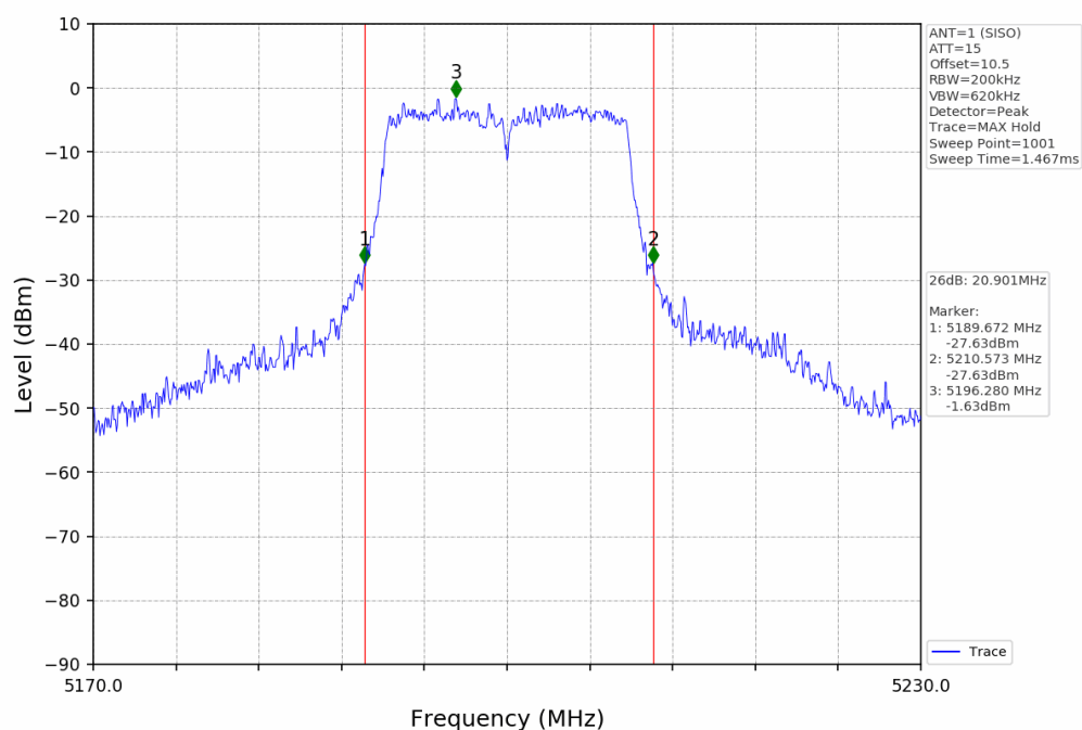
Bandwidth NTNV_802.11ac(VHT20)_SISO_5200MHz_ANT1
