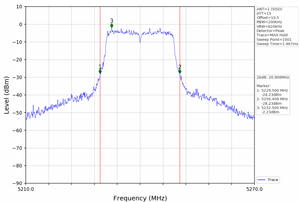
Bandwidth NTNV_802.11n(HT20)_SISO_5240MHz_ANT1
