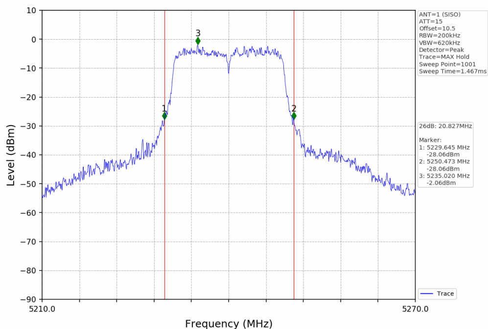
Bandwidth NTNV_802.11ac(VHT20)_SISO_5240MHz_ANT1
