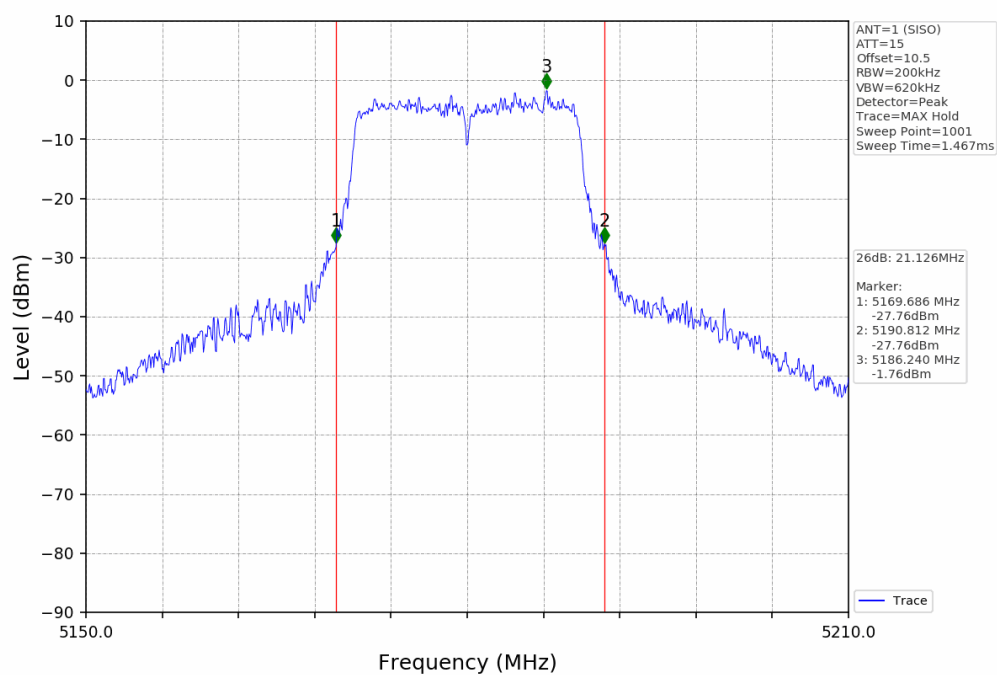
Bandwidth NTNV_802.11ac(VHT20)_SISO_5180MHz_ANT1
