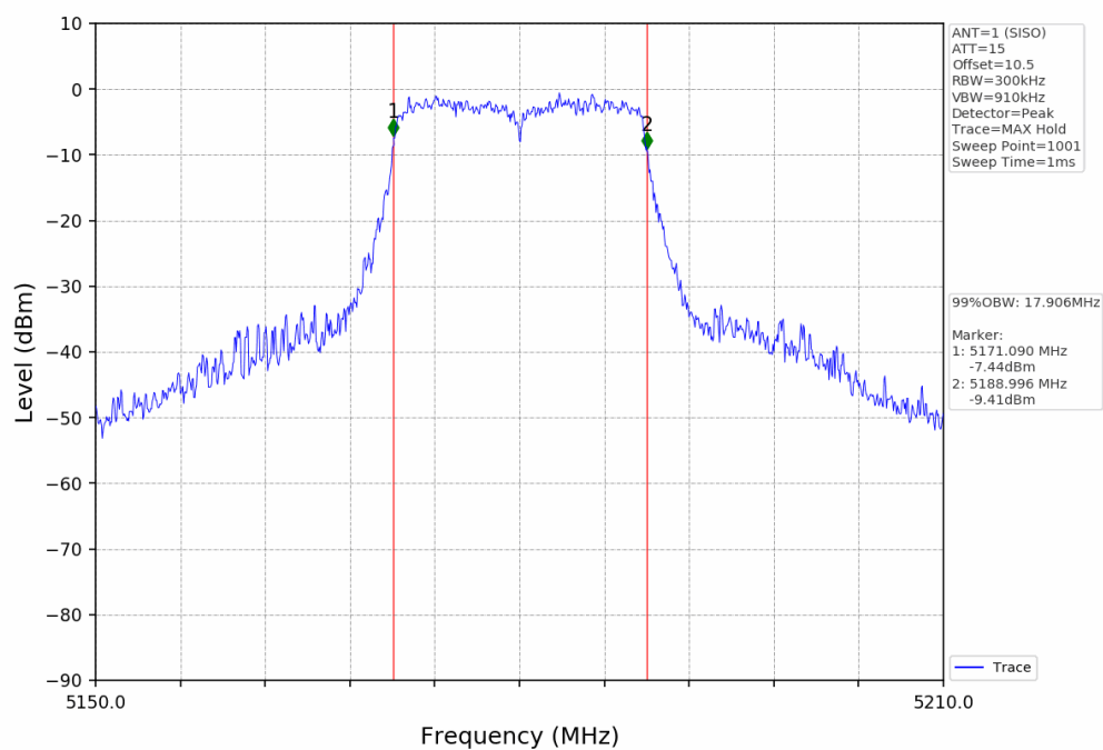
Bandwidth NTNV_802.11ac(VHT20)_SISO_5180MHz_ANT1
