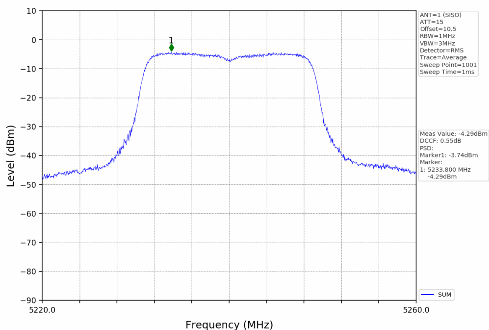
Maximum Power Spectral Density (PSD) NTVN_802.11n(HT20)_SISO_5240MHz_ANT1
