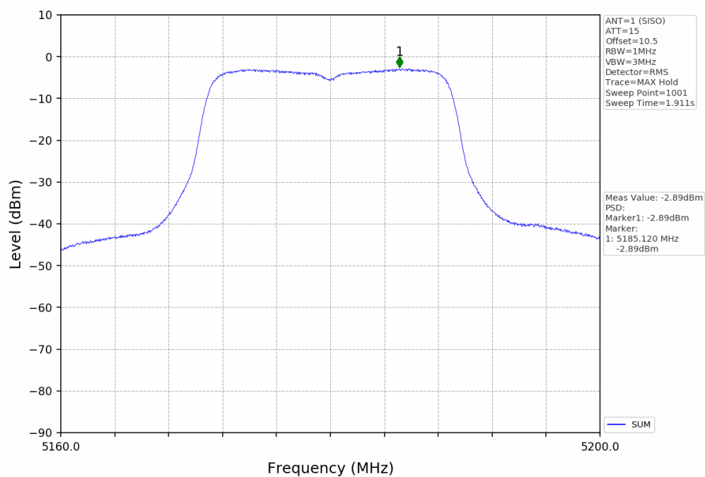
Maximum Power Spectral Density (PSD) NTVN_802.11ac(VHT20)_SISO_5180MHz_ANT1
