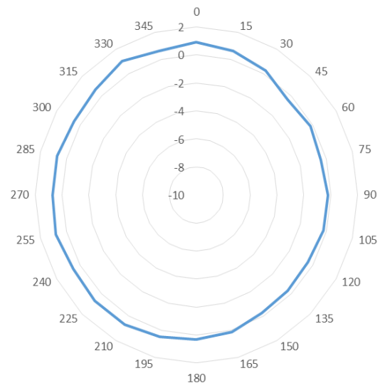
theta90° (XOY) Radiation Pattern at 2.45GHz
