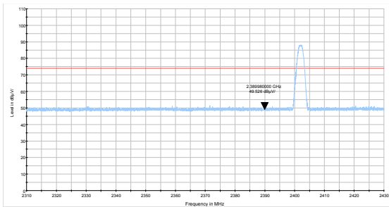
BLE Channel 0 Peak
