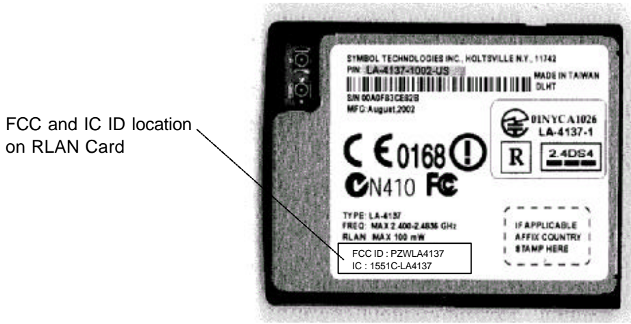
Fig.2 Marking location of Scanner
