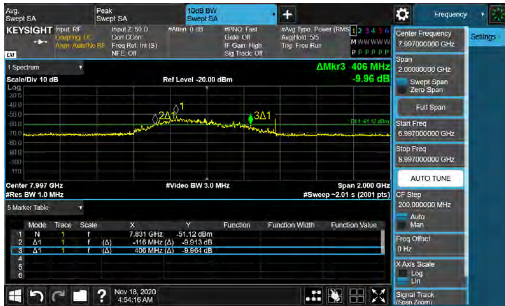
Plot 7-4. BANDWIDTH Plot – ANT2 - CH.9 - SP0 – Preamble 9
