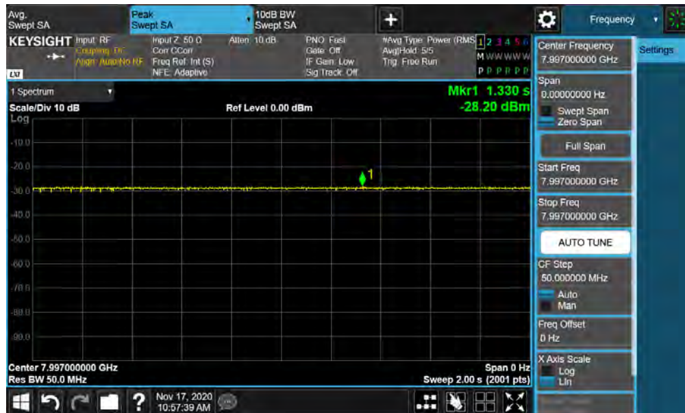
Plot 7-74. UWB Peak Power Measurement - ANT 1 - CH.9 – SP1 – BPRF
