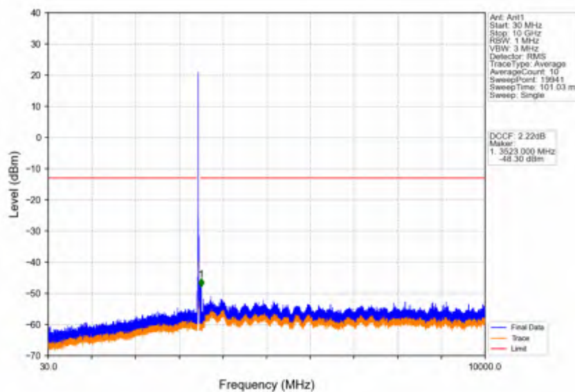
Band42a_20MHz_64QAM_LCH_3460MHz_RB_1_0_NTNV
