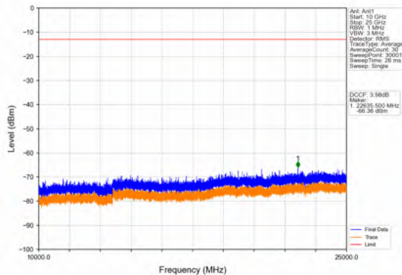
Band42c_15MHz_256QAM_HCH_3592.5MHz_RB_1_0_NTNV
