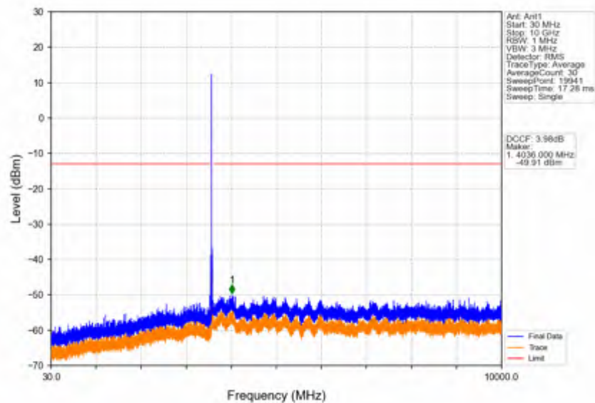
Band42c_20MHz_256QAM_HCH_3590MHz_RB_1_0_NTNV
