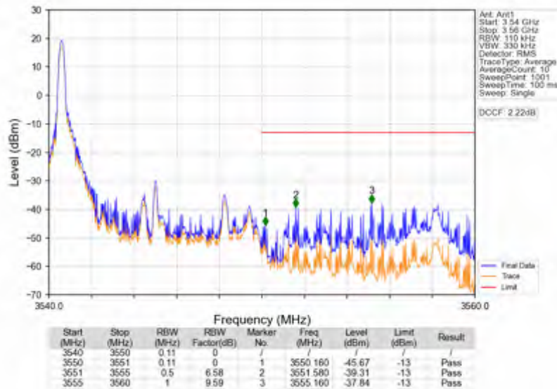
Band42a_10MHz_16QAM_HCH_3545MHz_RB_50_0_NTNV
