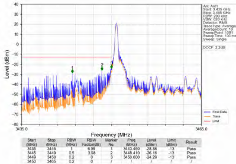
Band42a_15MHz_16QAM_LCH_3457.5MHz_RB_75_0_NTNV
