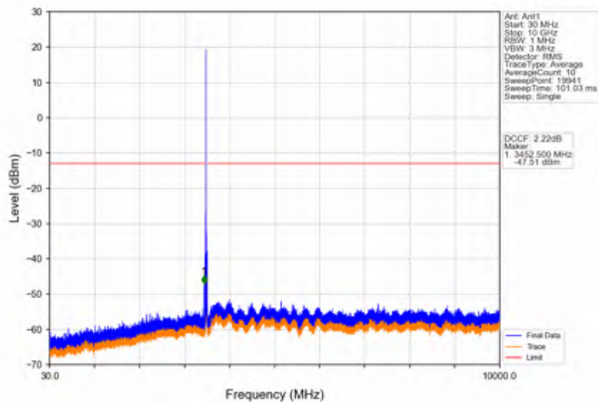
Band42a_15MHz_16QAM_MCH_3500MHz_RB_1_0_NTNV
