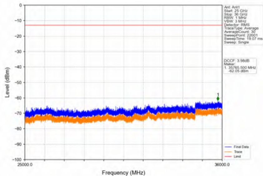
Band42c_15MHz_64QAM_LCH_3557.5MHz_RB_1_0_NTNV
