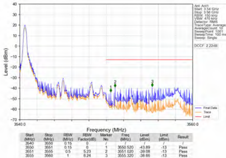
Band42a_10MHz_16QAM_HCH_3545MHz_RB_1_49_NTNV
