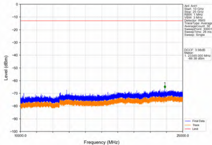
Band42c_5MHz_256QAM_HCH_3597.5MHz_RB_1_0_NTNV
