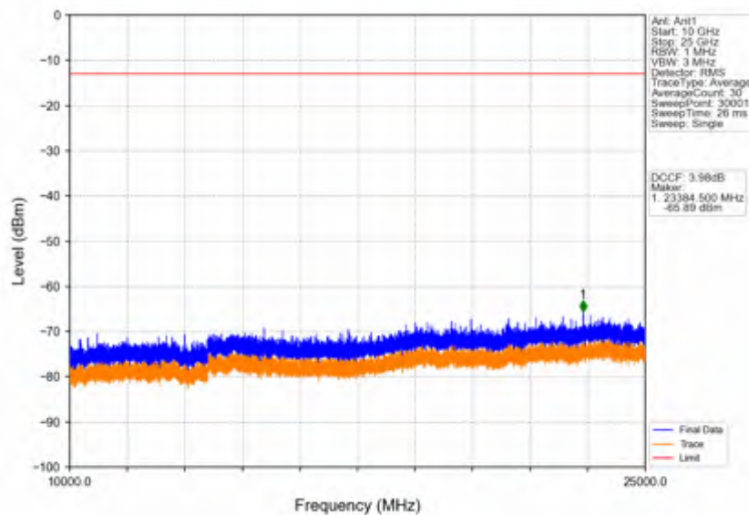
Band42c_20MHz_256QAM_LCH_3560MHz_RB_1_0_NTNV
