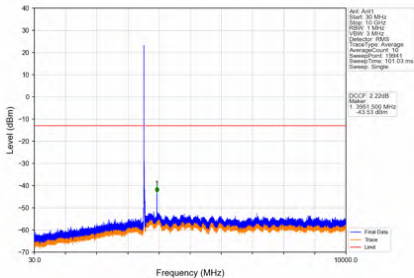
Band42a_15MHz_QPSK_HCH_3542.5MHz_RB_1_0_NTNV
