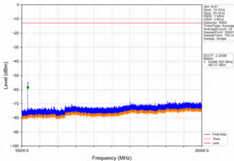
Band42a_10MHz_256QAM_MCH_3500MHz_RB_1_0_NTNV
