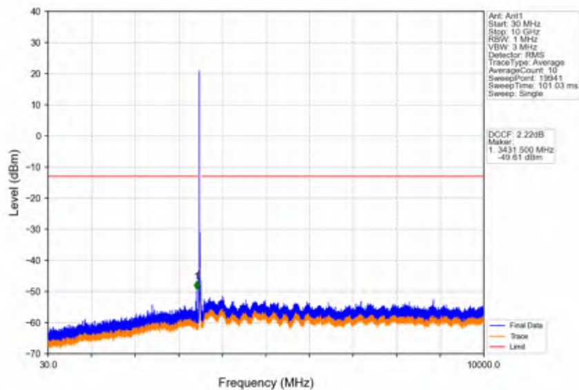
Band42a_20MHz_16QAM_MCH_3500MHz_RB_1_0_NTNV
