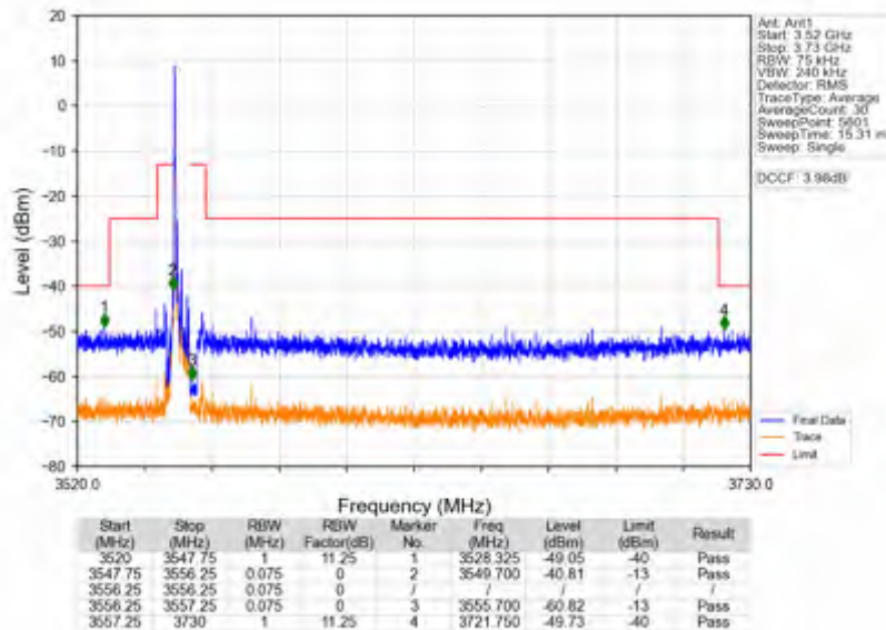
Band42c_5MHz_64QAM_LCH_3552.5MHz_RB_1_0_NTNV
