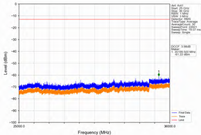
Band42c_20MHz_64QAM_LCH_3560MHz_RB_1_0_NTNV
