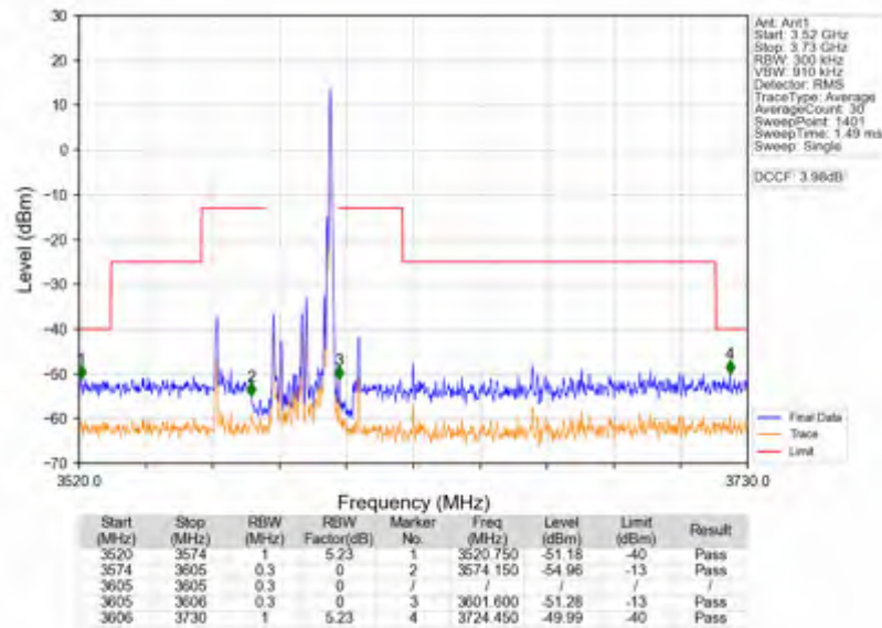
Band42c_20MHz_256QAM_HCH_3590MHz_RB_100_0_NTNV
