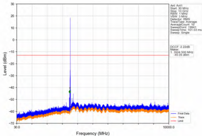
Band42a_10MHz_64QAM_HCH_3545MHz_RB_1_0_NTNV
