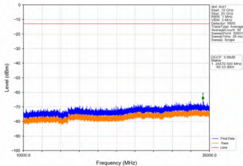
Band42c_15MHz_64QAM_MCH_3575MHz_RB_1_0_NTNV
