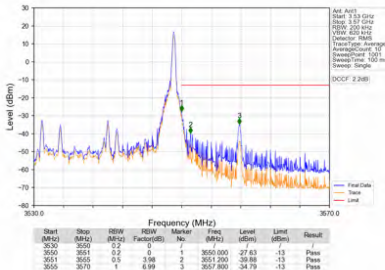
Band42a_20MHz_256QAM_HCH_3540MHz_RB_1_99_NTNV
