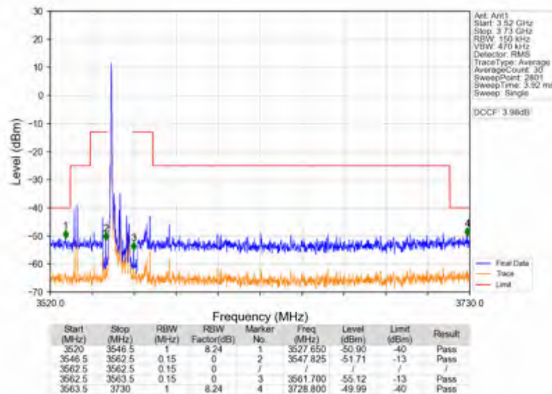
Band42c_10MHz_64QAM_LCH_3555MHz_RB_1_0_NTNV
