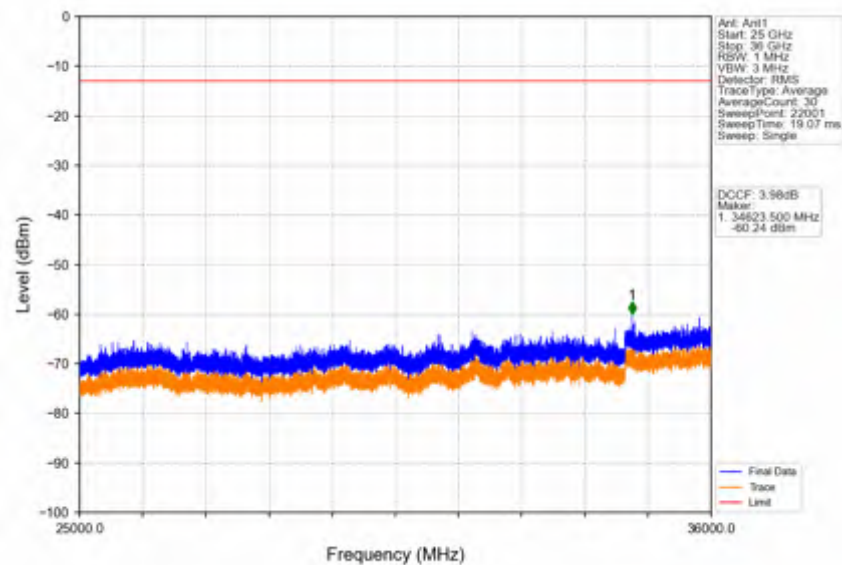
Band42c_15MHz_16QAM_HCH_3592.5MHz_RB_1_0_NTNV
