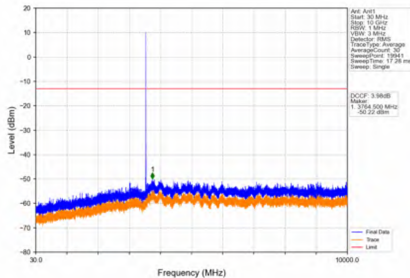
Band42c_10MHz_64QAM_LCH_3555MHz_RB_1_0_NTNV
