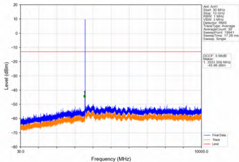
Band42c_10MHz_16QAM_HCH_3595MHz_RB_1_0_NTNV
