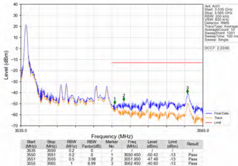
Band42a_15MHz_16QAM_HCH_3542.5MHz_RB_1_74_NTNV
