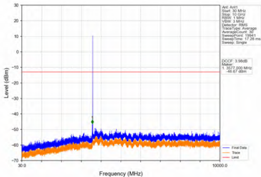
Band42c_5MHz_16QAM_HCH_3597.5MHz_RB_1_0_NTNV
