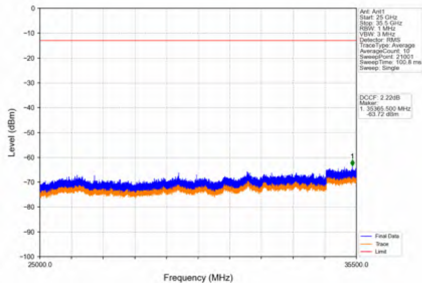
Band42a_15MHz_64QAM_MCH_3500MHz_RB_1_0_NTNV
