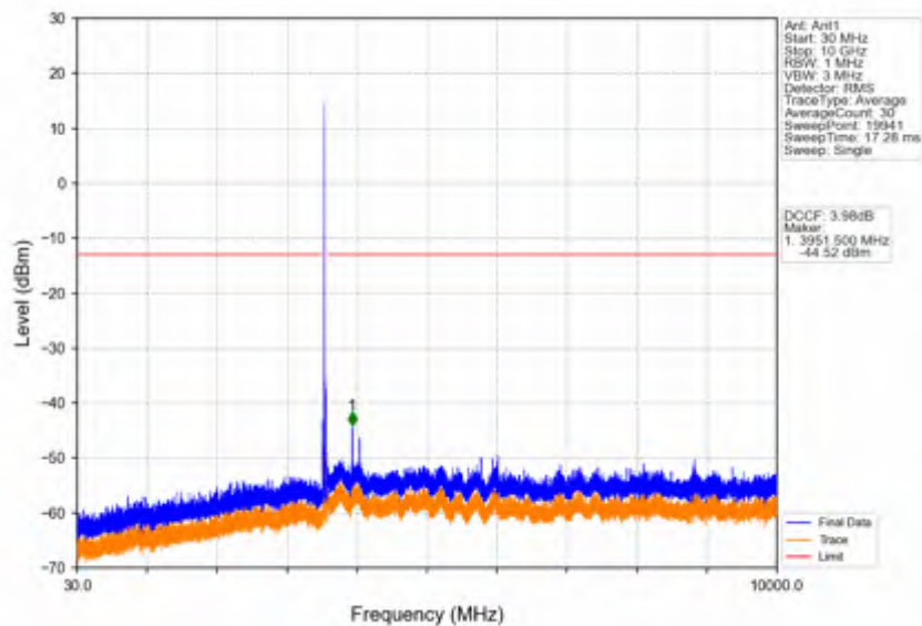
Band42c_20MHz_256QAM_LCH_3560MHz_RB_1_0_NTNV
