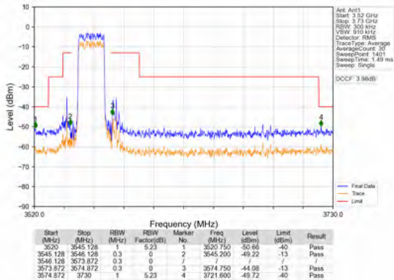
Band42c_20MHz_64QAM_MCH_3575MHz_RB_1_0_NTNV
