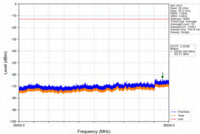
Band42a_15MHz_QPSK_LCH_3457.5MHz_RB_1_0_NTNV
