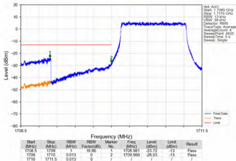
Band66_1.4MHz_16QAM_LCH_1710.7MHz_RB_6_0_NTNV
