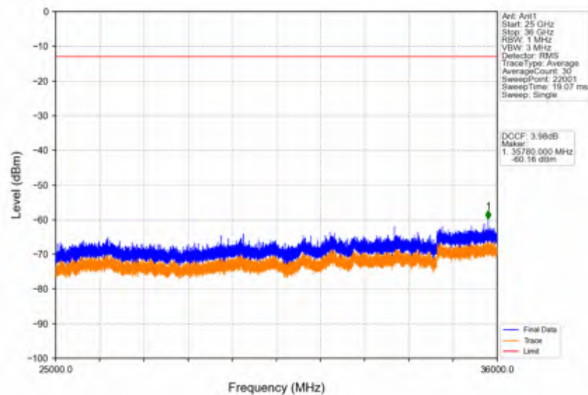
Band42c_10MHz_64QAM_HCH_3595MHz_RB_1_49_NTNV
