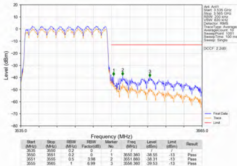
Band42a_15MHz_256QAM_HCH_3542.5MHz_RB_75_0_NTNV
