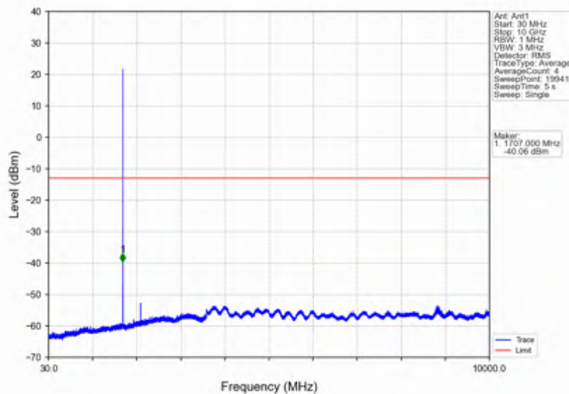
Band66_1.4MHz_16QAM_LCH_1710.7MHz_RB_1_0_NTNV
