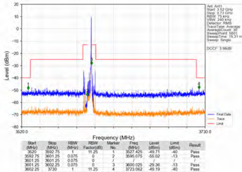
Band42c_5MHz_256QAM_HCH_3597.5MHz_RB_25_0_NTNV
