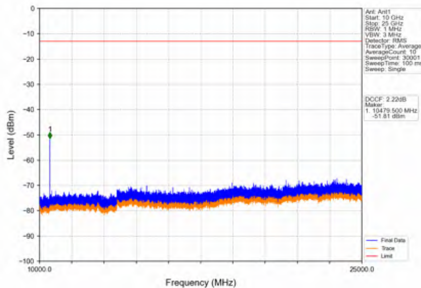
Band42a_15MHz_QPSK_MCH_3500MHz_RB_1_0_NTNV
