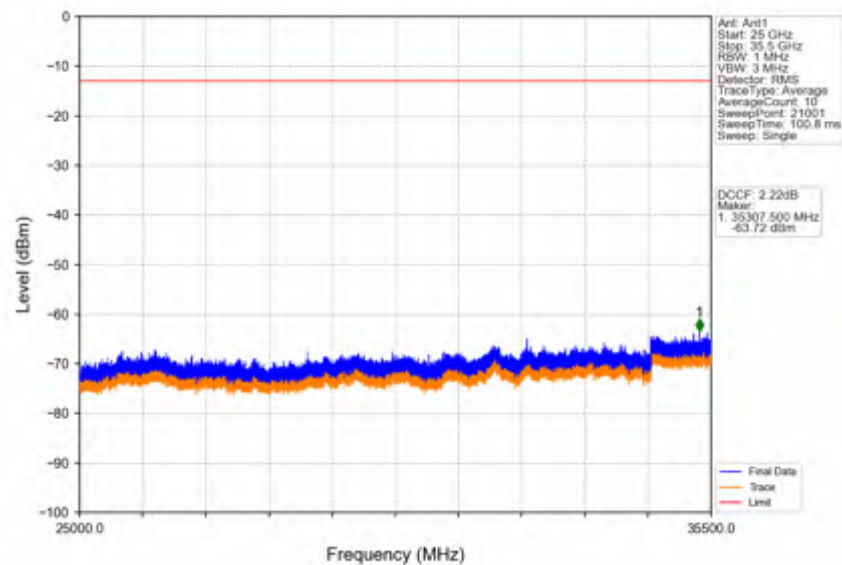
Band42a_20MHz_64QAM_MCH_3500MHz_RB_1_0_NTNV
