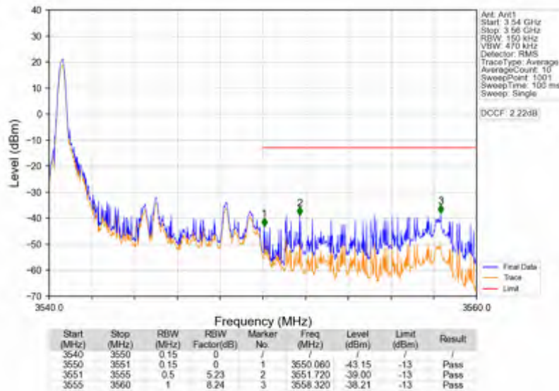
Band42a_10MHz_64QAM_HCH_3545MHz_RB_50_0_NTNV
