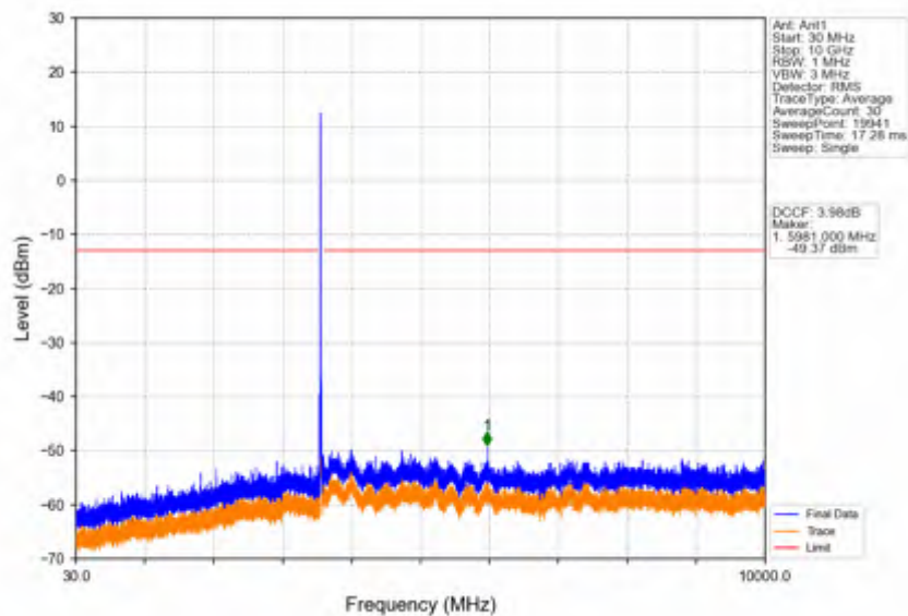
Band42c_20MHz_256QAM_MCH_3575MHz_RB_1_0_NTNV
