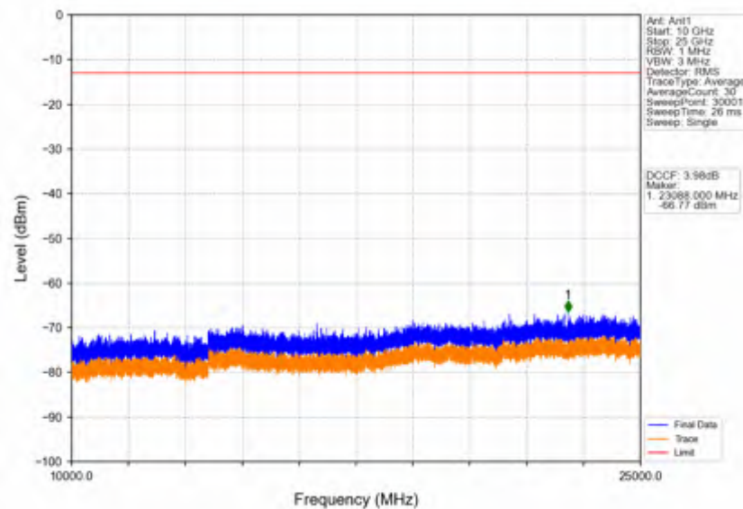
Band42c_5MHz_64QAM_MCH_3575MHz_RB_1_0_NTNV
