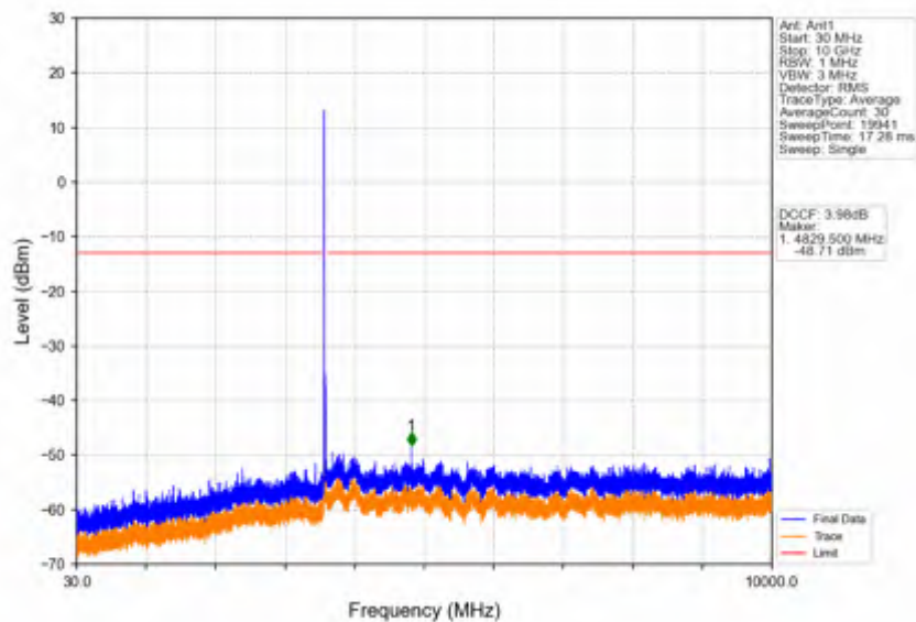
Band42c_20MHz_64QAM_HCH_3590MHz_RB_1_0_NTNV
