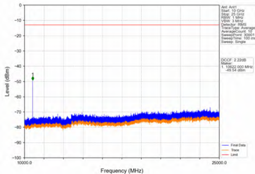
Band42a_10MHz_16QAM_HCH_3545MHz_RB_1_0_NTNV
