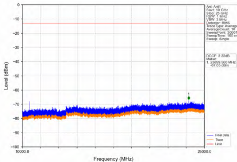
Band42a_15MHz_256QAM_HCH_3542.5MHz_RB_1_0_NTNV
