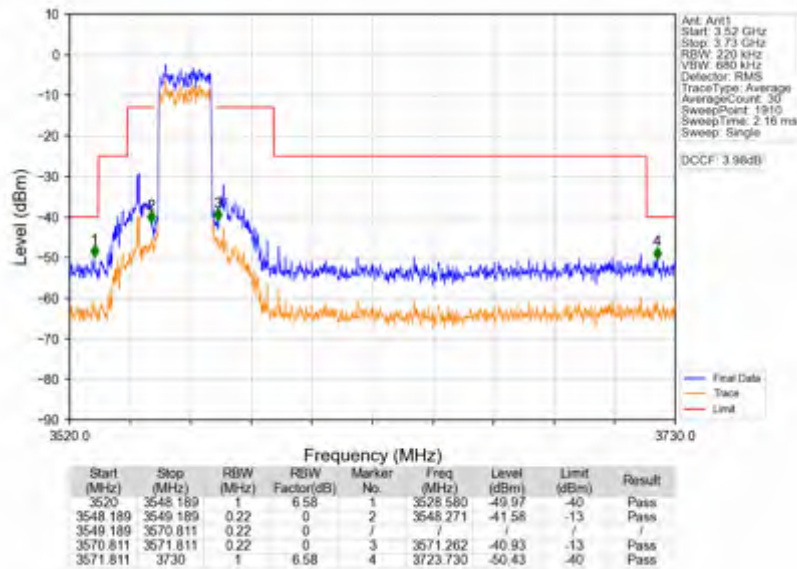
Band42c 20MHz QPSK MCH 3575MHz RB 1 0 NTNV
