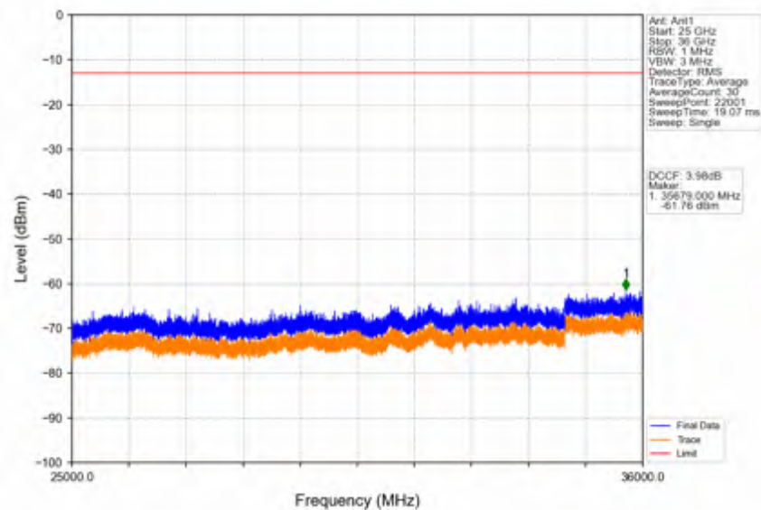
Band42c_5MHz_64QAM_LCH_3552.5MHz_RB_1_0_NTNV
