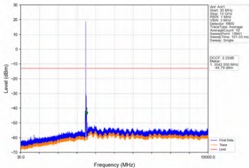
Band42a_15MHz_256QAM_MCH_3500MHz_RB_1_0_NTNV
