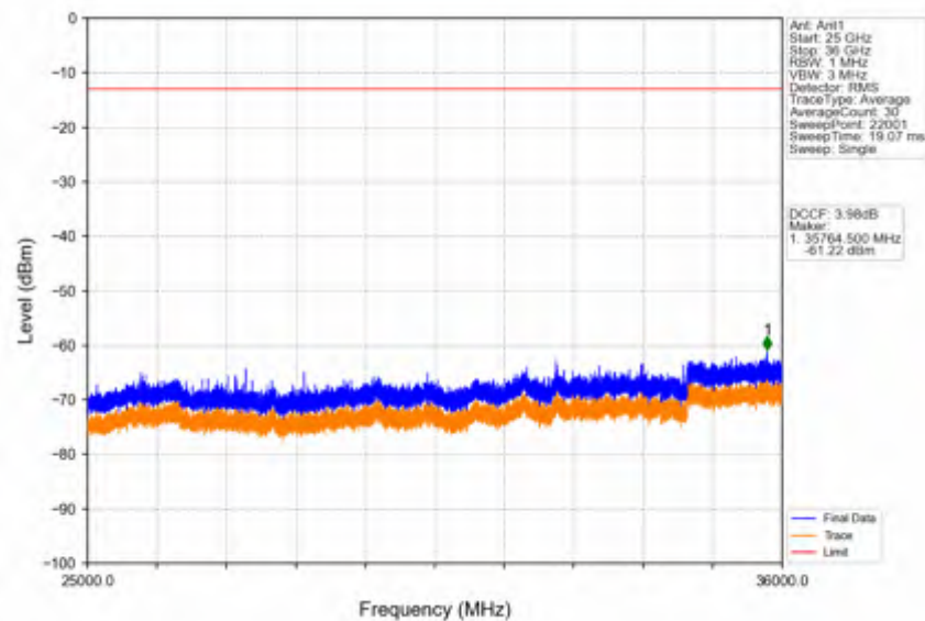
Band42c_5MHz_256QAM_LCH_3552.5MHz_RB_25_0_NTNV
