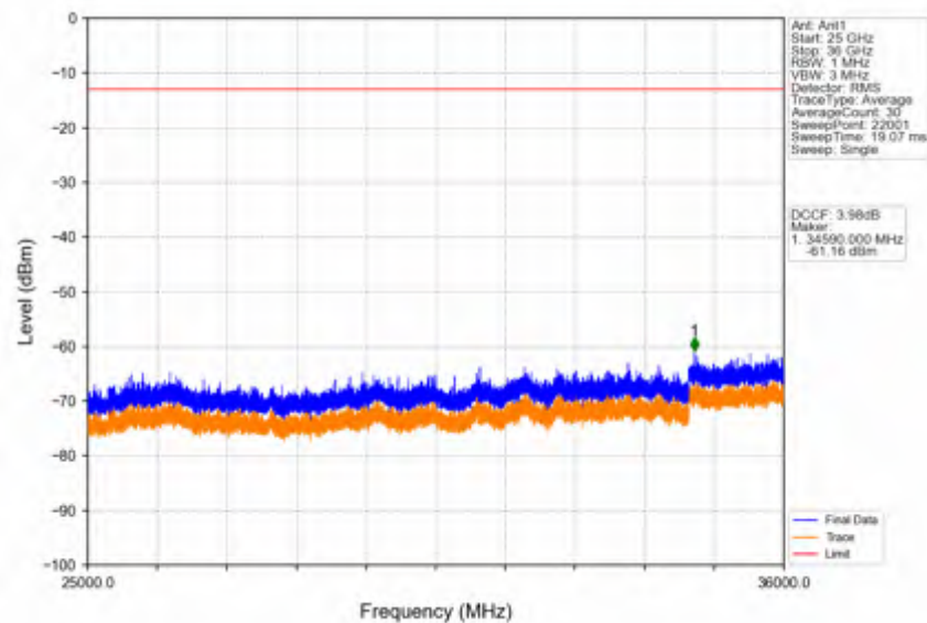
Band42c_20MHz_64QAM_HCH_3590MHz_RB_1_99_NTNV
