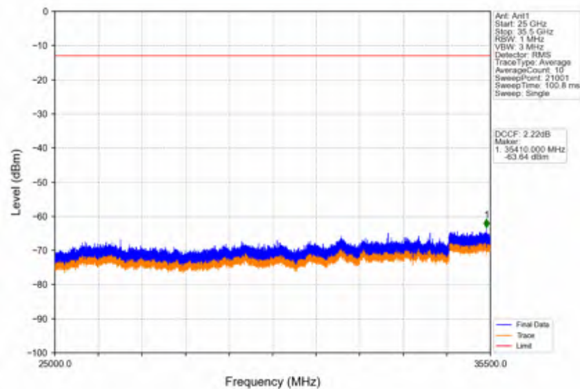
Band42a_15MHz_64QAM_LCH_3457.5MHz_RB_1_0_NTNV
