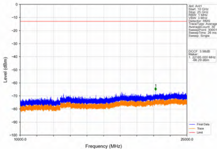
Band42c_15MHz_256QAM_LCH_3557.5MHz_RB_1_0_NTNV
