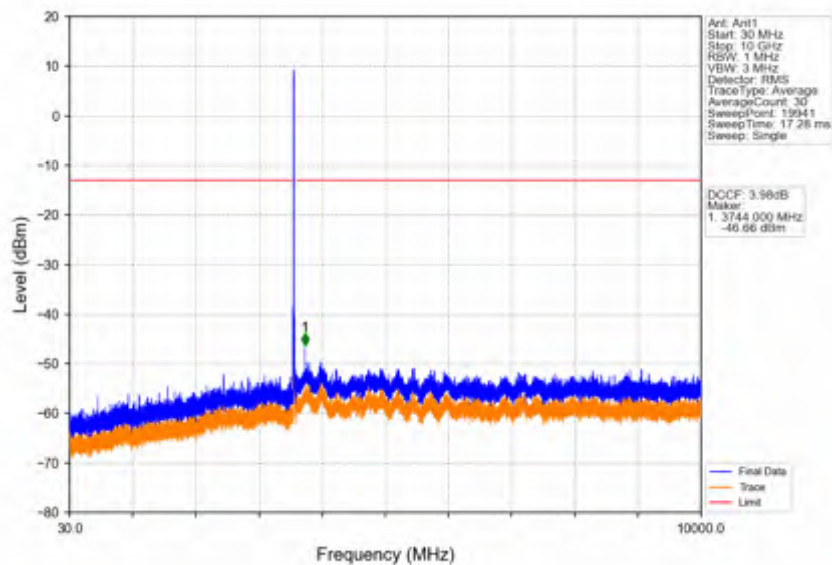
Band42c_15MHz_256QAM_MCH_3575MHz_RB_1_0_NTNV
