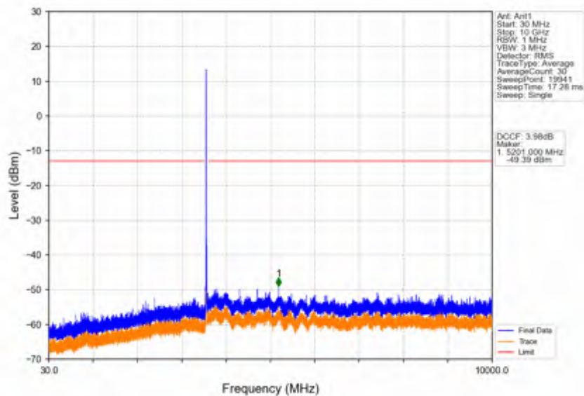
Band42c_20MHz_16QAM_MCH_3575MHz_RB_1_0_NTNV
