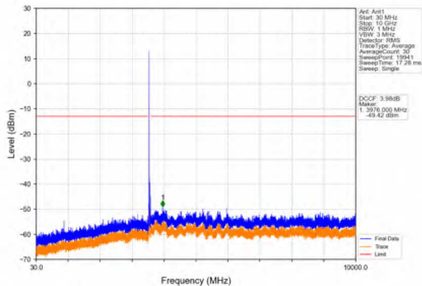
Band42c_20MHz_64QAM_LCH_3560MHz_RB_1_0_NTNV
