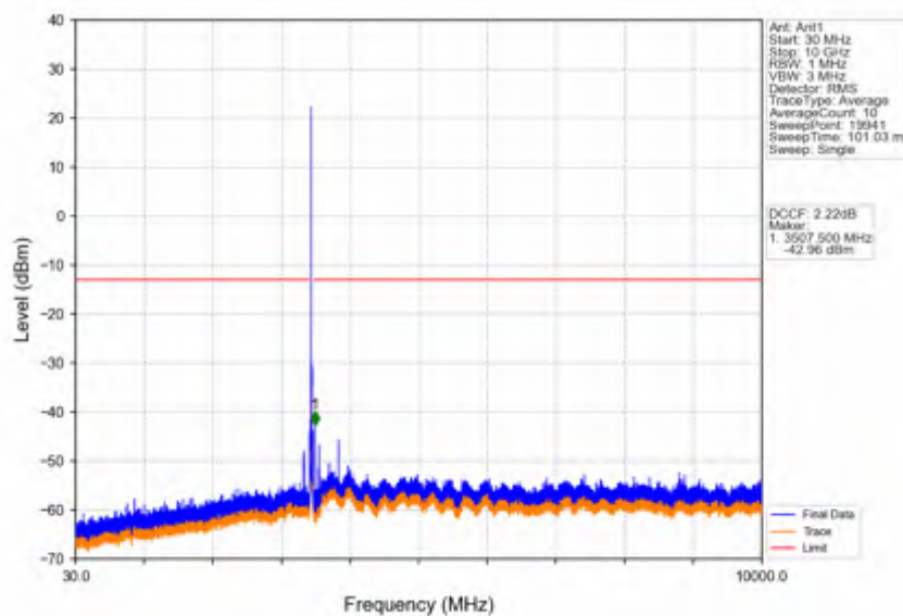
Band42a_15MHz_64QAM_LCH_3457.5MHz_RB_1_0_NTNV
