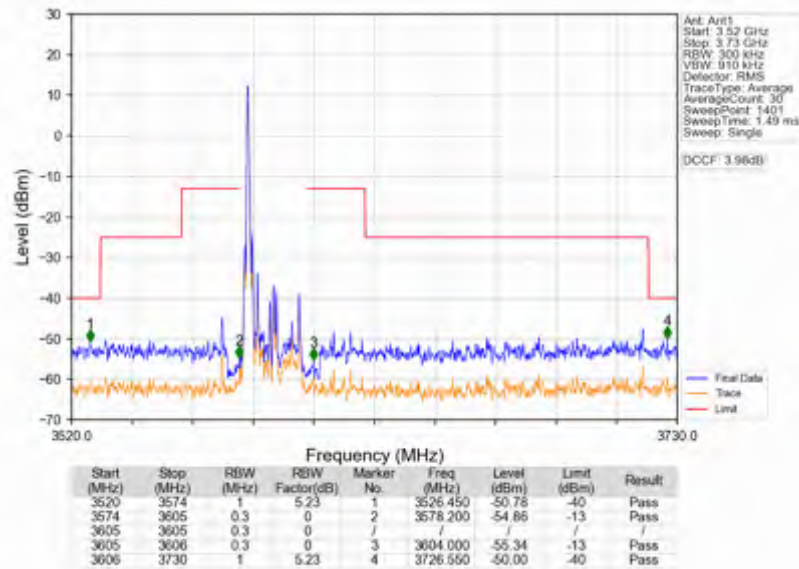
Band42c_20MHz_16QAM_HCH_3590MHz_RB_100_0_NTNV
