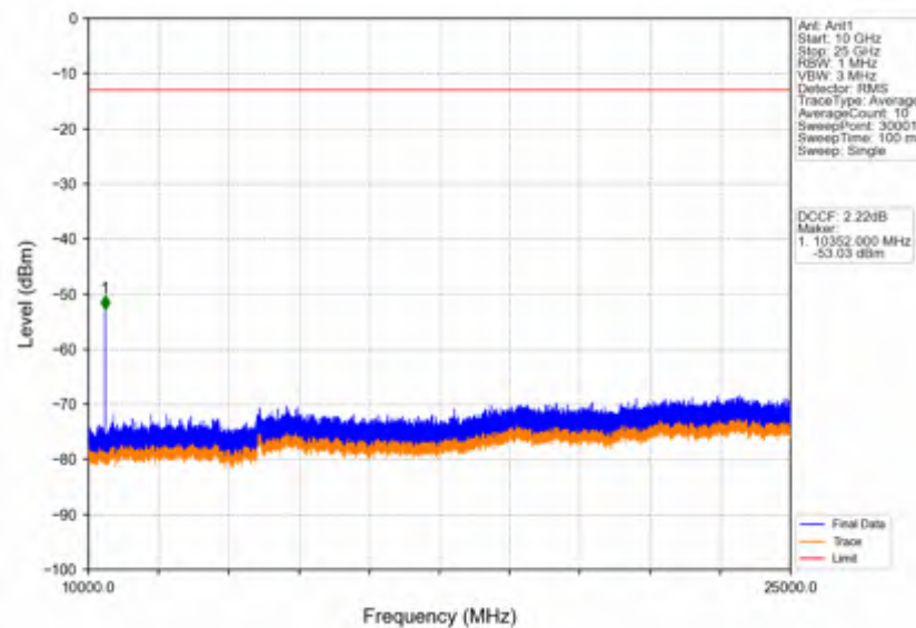
Band42a_15MHz_64QAM_LCH_3457.5MHz_RB_1_0_NTNV
