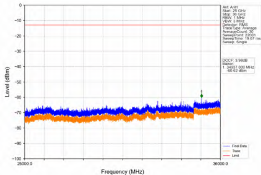
Band42c_10MHz_64QAM_LCH_3555MHz_RB_1_0_NTNV
