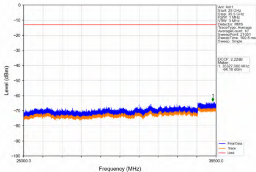
Band42a_15MHz_16QAM_HCH_3542.5MHz_RB_1_0_NTNV
