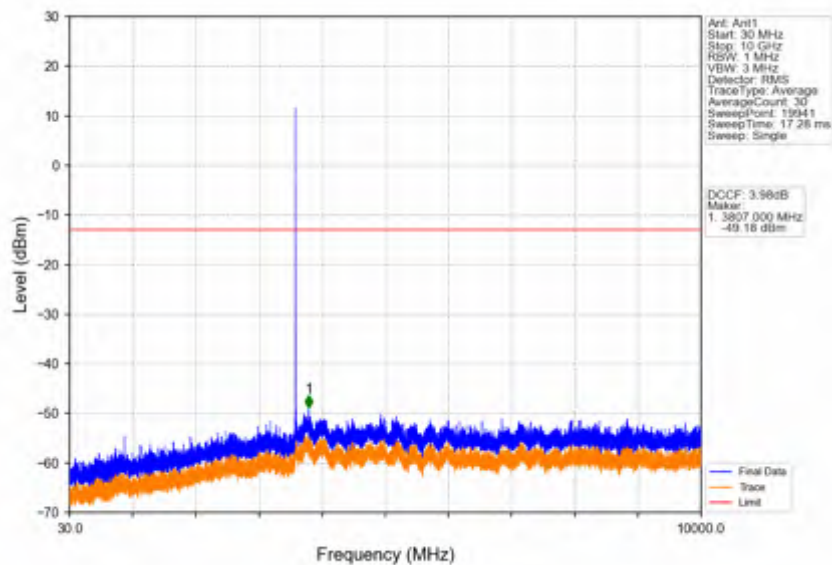
Band42c_5MHz_QPSK_HCH_3597.5MHz_RB_1_0_NTNV
