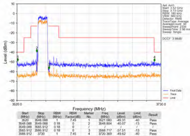
Band42c_15MHz_256QAM_LCH_3557.5MHz_RB_75_0_NTNV
