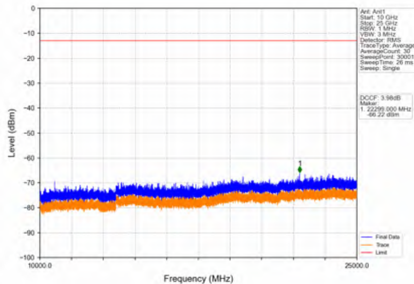
Band42c_15MHz_QPSK_LCH_3557.5MHz_RB_1_0_NTNV
