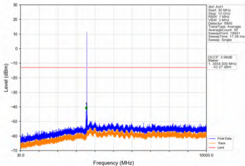
Band42c_15MHz_QPSK_HCH_3592.5MHz_RB_1_0_NTNV
