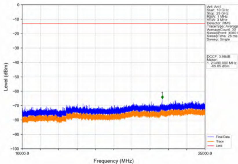
Band42c_15MHz_256QAM_MCH_3575MHz_RB_1_0_NTNV
