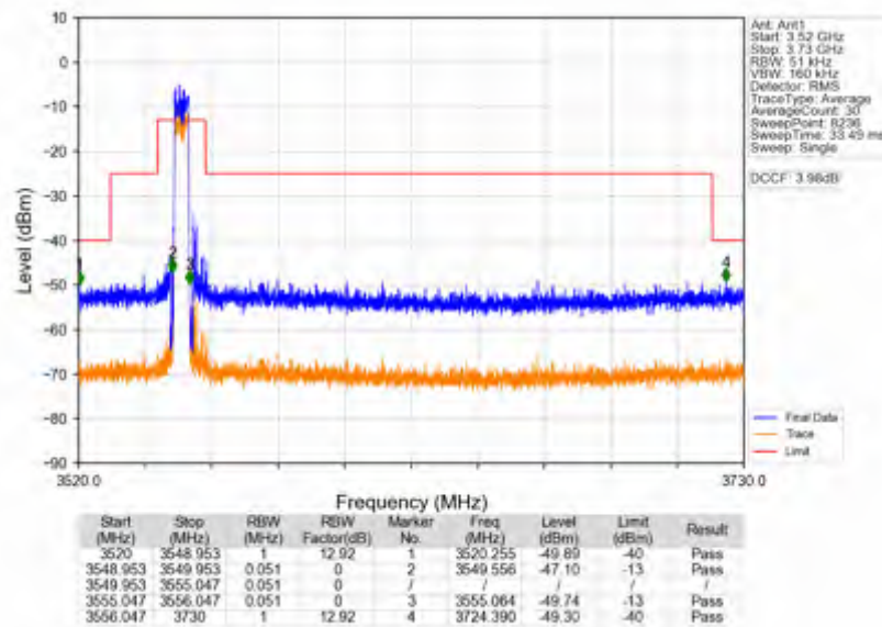
Band42c_5MHz_256QAM_LCH_3552.5MHz_RB_25_0_NTNV
