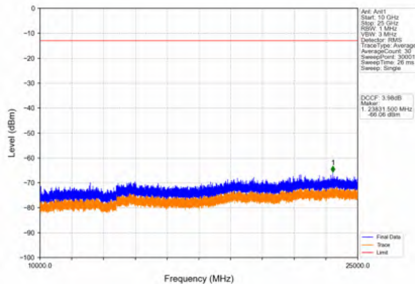
Band42c_20MHz_16QAM_HCH_3590MHz_RB_1_0_NTNV
