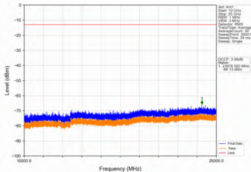
Band42c_10MHz_256QAM_HCH_3595MHz_RB_1_0_NTNV
