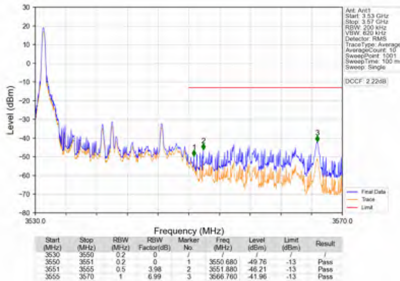
Band42a_20MHz_64QAM_HCH_3540MHz_RB_100_0_NTNV
