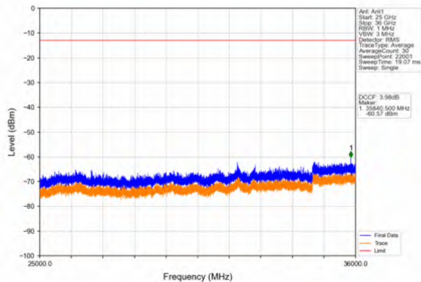
Band42c_20MHz_16QAM_HCH_3590MHz_RB_1_0_NTNV
