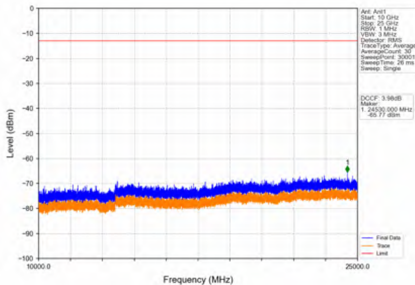
Band42c_15MHz_64QAM_HCH_3592.5MHz_RB_1_0_NTNV
