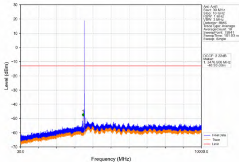
Band42a_10MHz_256QAM_HCH_3545MHz_RB_1_0_NTNV
