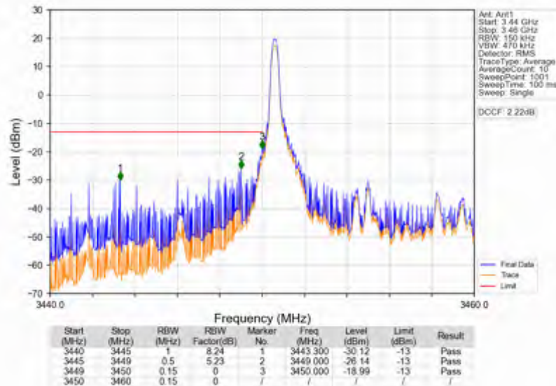
Band42a_10MHz_64QAM_LCH_3455MHz_RB_1_0_NTNV
