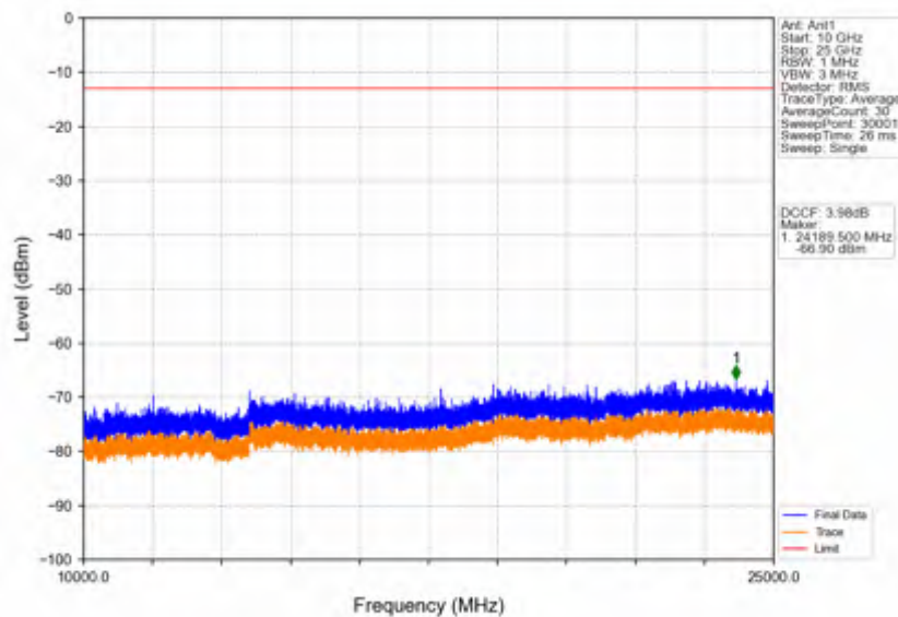
Band42c_5MHz_256QAM_MCH_3575MHz_RB_1_0_NTNV
