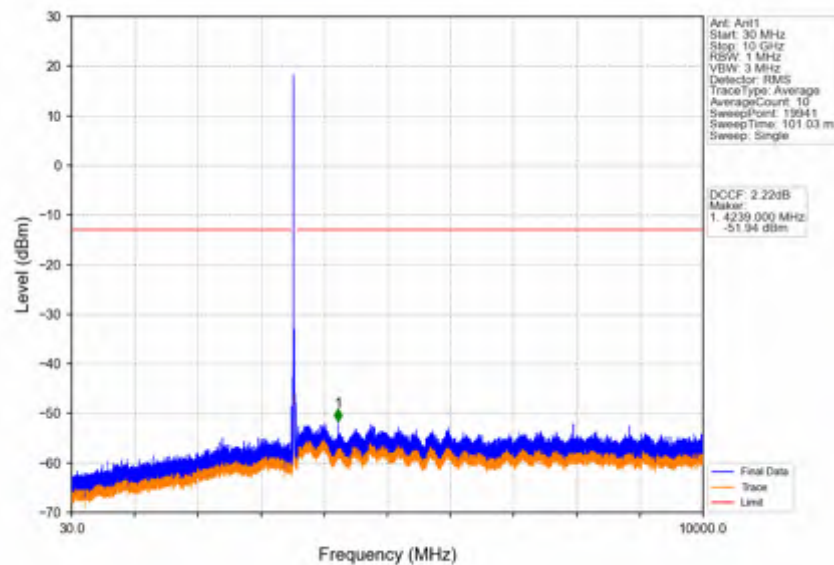
Band42a_20MHz_256QAM_HCH_3540MHz_RB_1_0_NTNV
