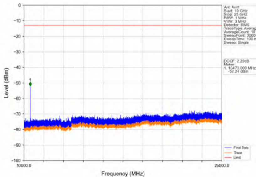
Band42a_20MHz_16QAM_MCH_3500MHz_RB_1_0_NTNV
