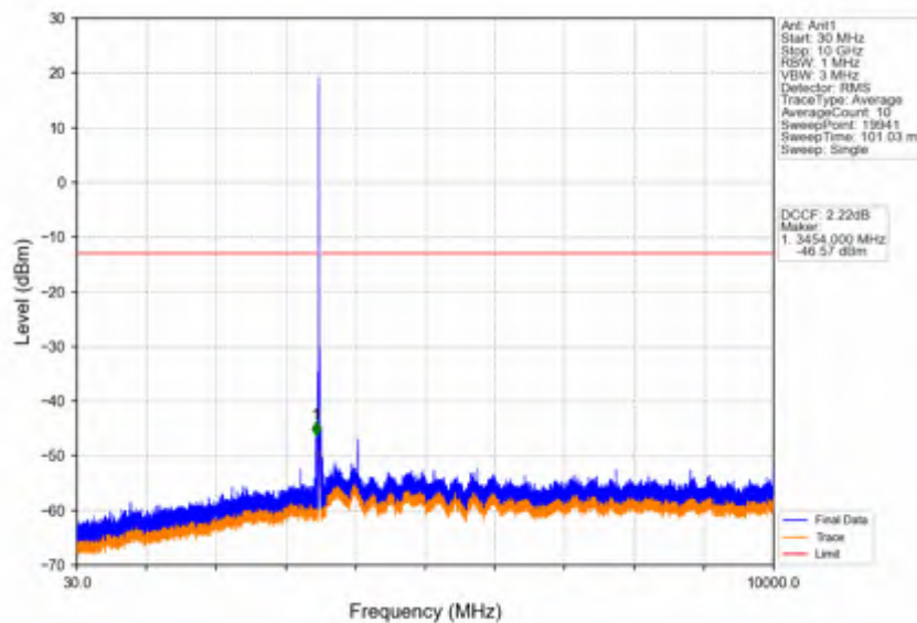
Band42a_15MHz_QPSK_MCH_3500MHz_RB_1_0_NTNV
