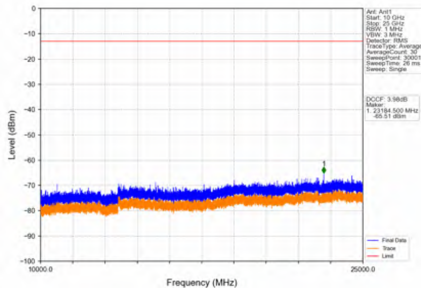
Band42c_20MHz_64QAM_LCH_3560MHz_RB_1_0_NTNV
