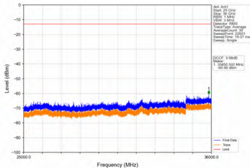
Band42c_5MHz_64QAM_HCH_3597.5MHz_RB_1_24_NTNV
