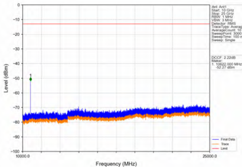
Band42a_10MHz_64QAM_HCH_3545MHz_RB_1_0_NTNV
