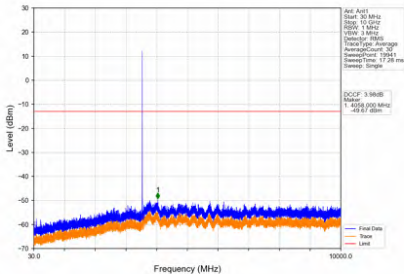
Band42c_5MHz_64QAM_LCH_3552.5MHz_RB_1_0_NTNV
