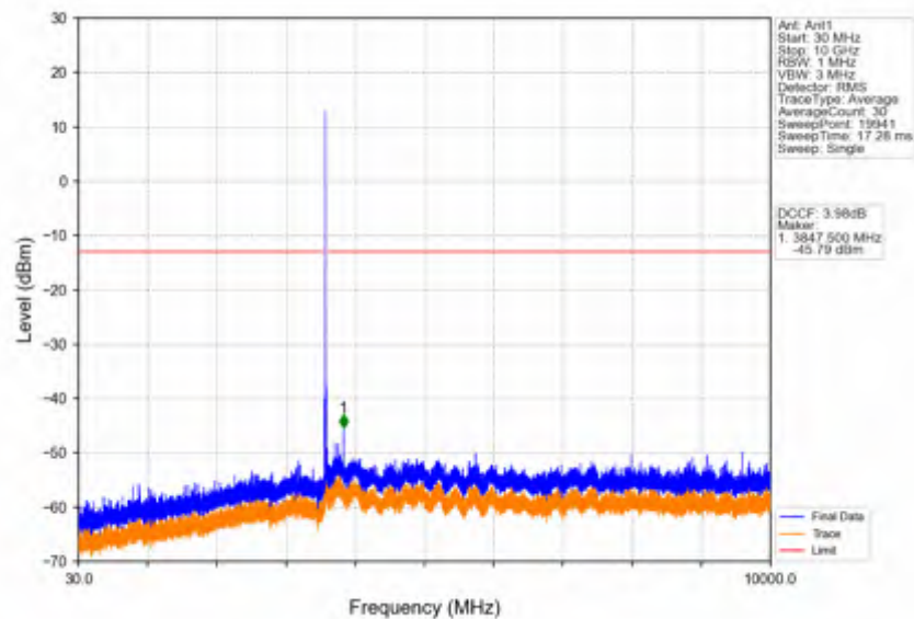
Band42c_15MHz_256QAM_HCH_3592.5MHz_RB_1_0_NTNV
