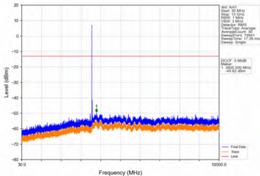
Band42c_10MHz_16QAM_MCH_3575MHz_RB_1_0_NTNV
