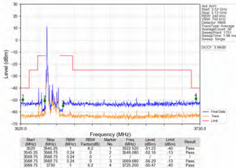
Band42c_15MHz_64QAM_LCH_3557.5MHz_RB_1_0_NTNV
