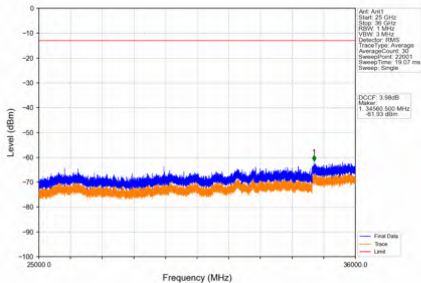
Band42c_5MHz_256QAM_HCH_3597.5MHz_RB_1_0_NTNV
