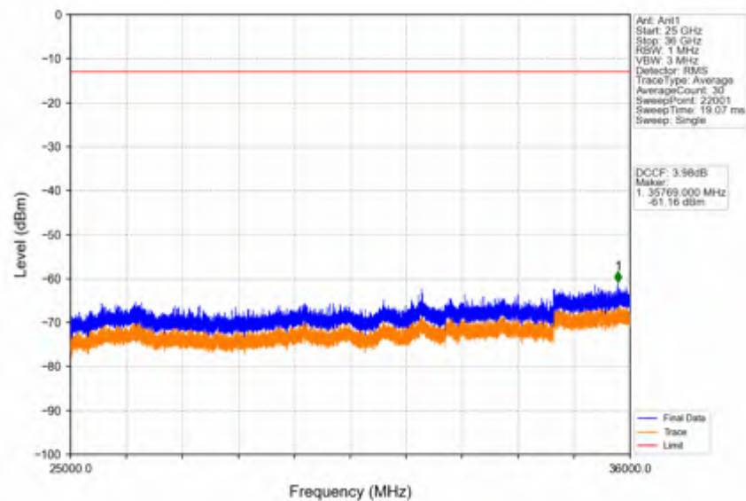
Band42c_20MHz_256QAM_HCH_3590MHz_RB_1_0_NTNV
