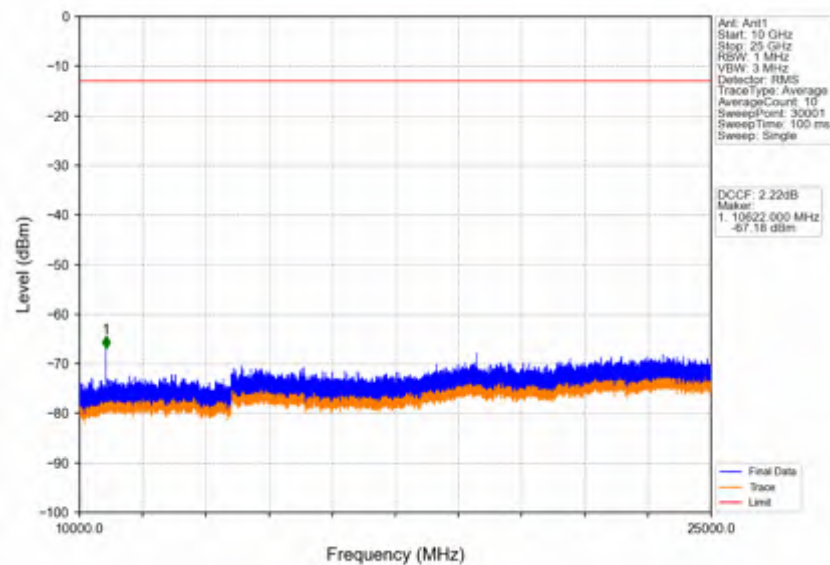
Band42a_10MHz_256QAM_HCH_3545MHz_RB_1_0_NTNV
