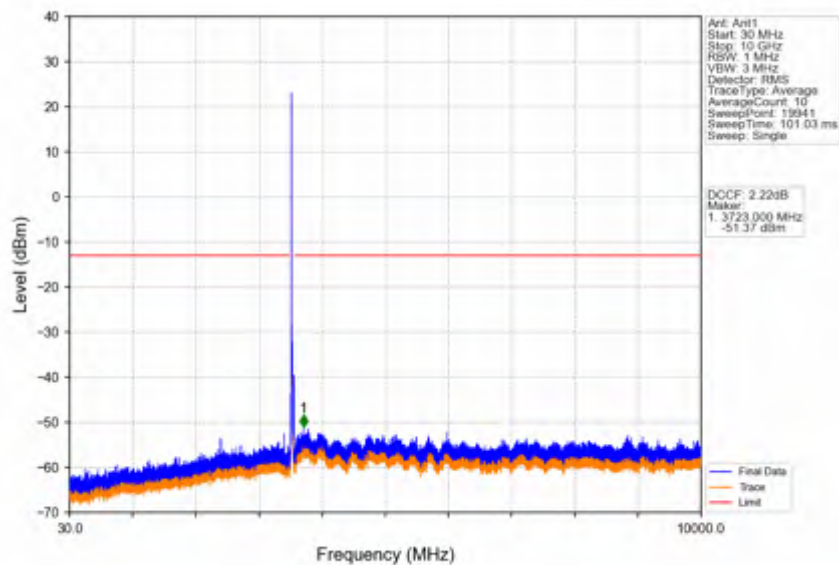
Band42a_20MHz_64QAM_HCH_3540MHz_RB_1_0_NTNV
