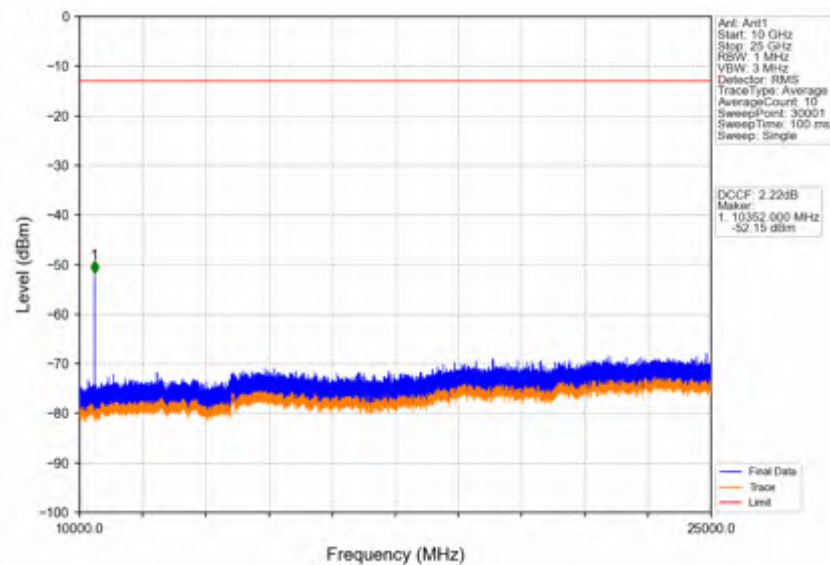
Band42a_15MHz_QPSK_LCH_3457.5MHz_RB_1_0_NTNV
