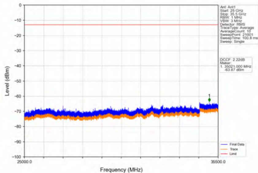
Band42a_15MHz_64QAM_HCH_3542.5MHz_RB_1_74_NTNV
