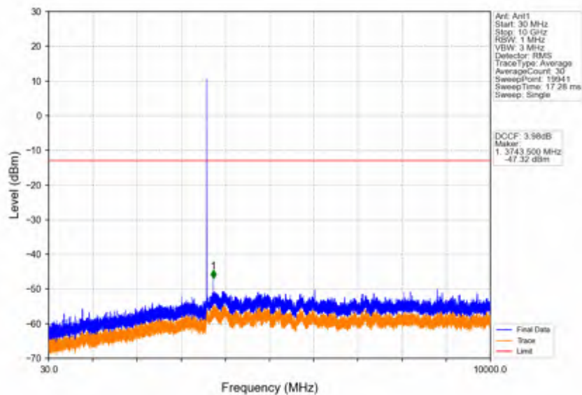
Band42c_5MHz_256QAM_HCH_3597.5MHz_RB_1_0_NTNV
