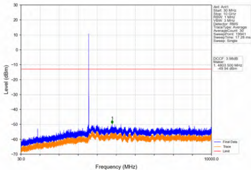
Band42c_5MHz_QPSK_MCH_3575MHz_RB_1_0_NTNV
