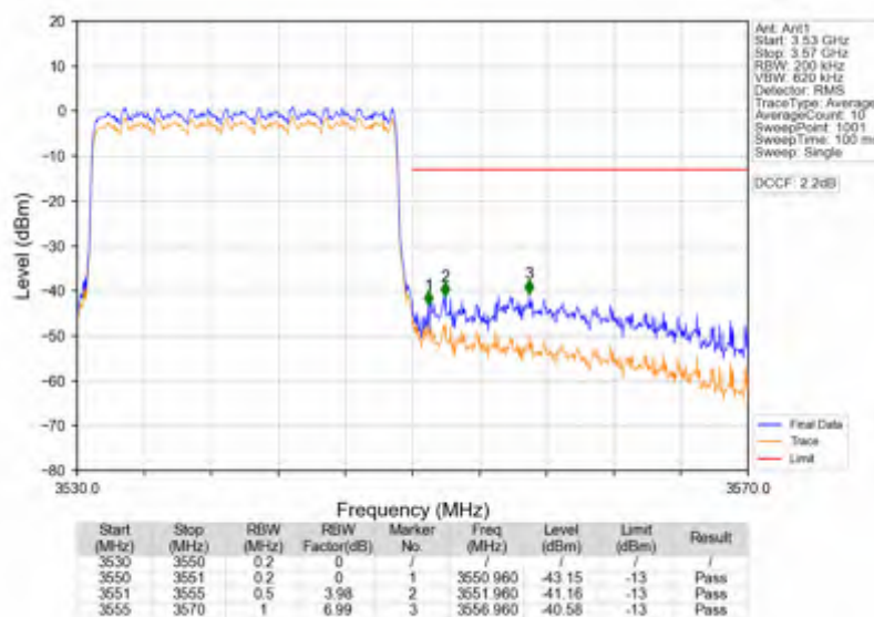
Band42a_20MHz_256QAM_HCH_3540MHz_RB_100_0_NTNV
