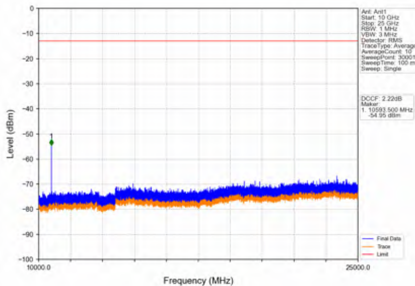
Band42a_20MHz_64QAM_HCH_3540MHz_RB_1_0_NTNV
