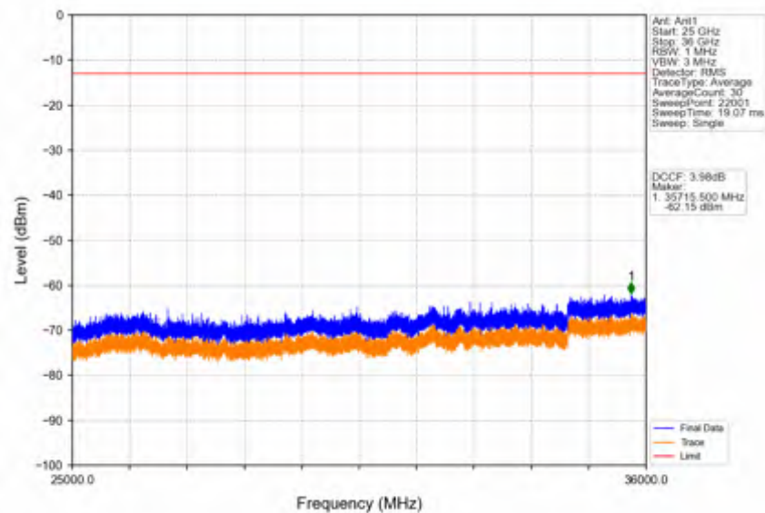
Band42c_5MHz_QPSK_LCH_3552.5MHz_RB_1_0_NTNV
