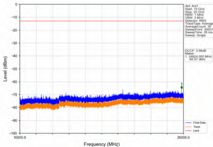
Band42c_10MHz_64QAM_HCH_3595MHz_RB_1_0_NTNV
