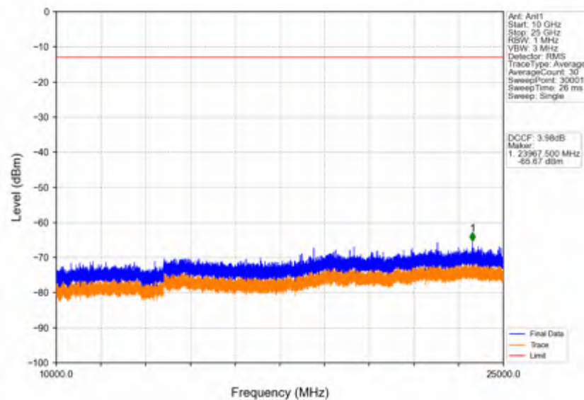
Band42c_10MHz_16QAM_HCH_3595MHz_RB_1_0_NTNV
