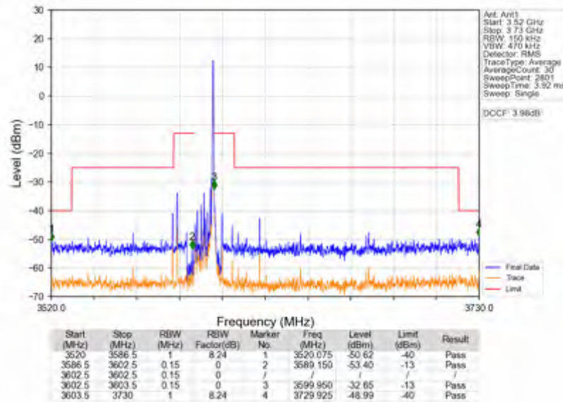
Band42c_10MHz_256QAM_HCH_3595MHz_RB_50_0_NTNV
