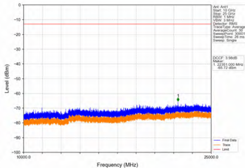
Band42c_5MHz_16QAM_HCH_3597.5MHz_RB_1_0_NTNV
