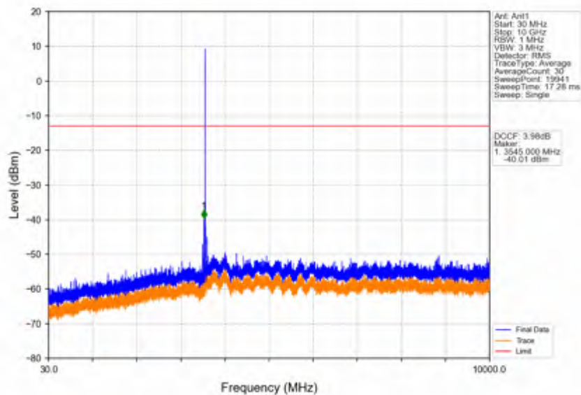
Band42c_10MHz_256QAM_MCH_3575MHz_RB_1_0_NTNV
