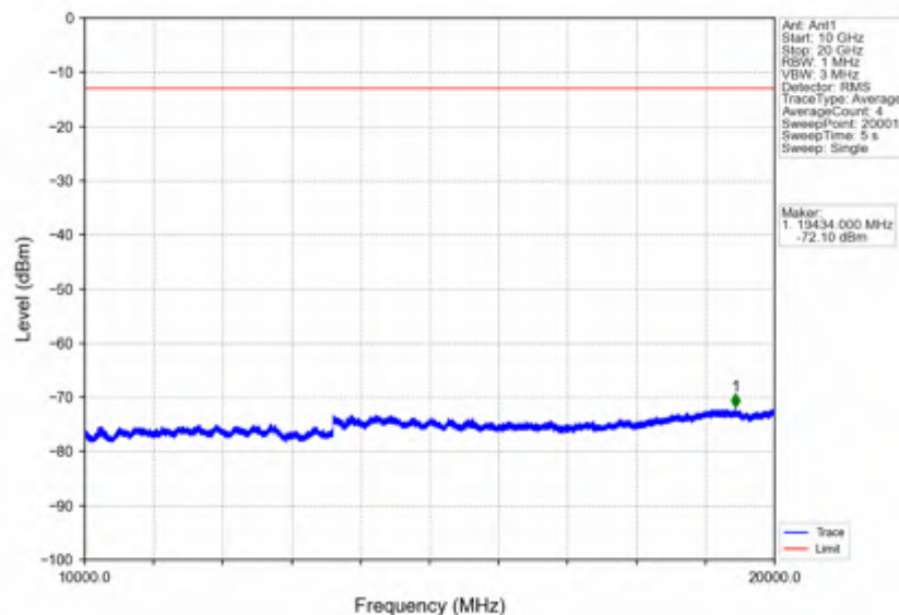
Band66_1.4MHz_16QAM_LCH_1710.7MHz_RB_6_0_NTNV
