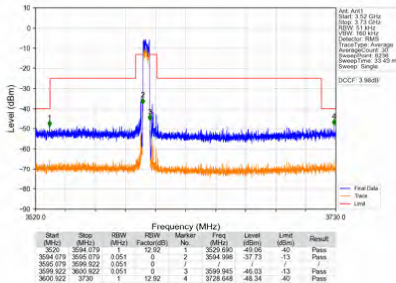
Band42c_5MHz_256QAM_HCH_3597.5MHz_RB_25_0_NTNV
