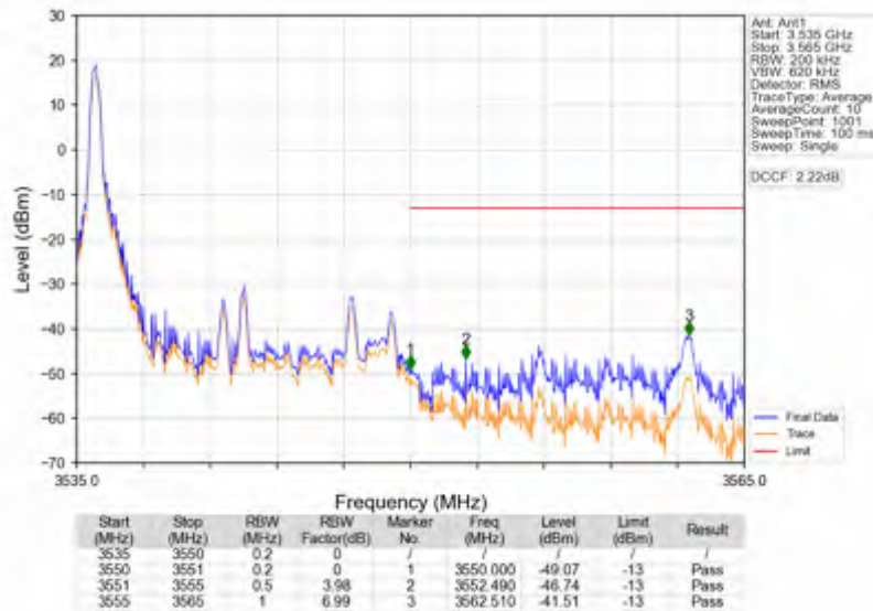
Band42a_15MHz_64QAM_HCH_3542.5MHz_RB_75_0_NTNV
