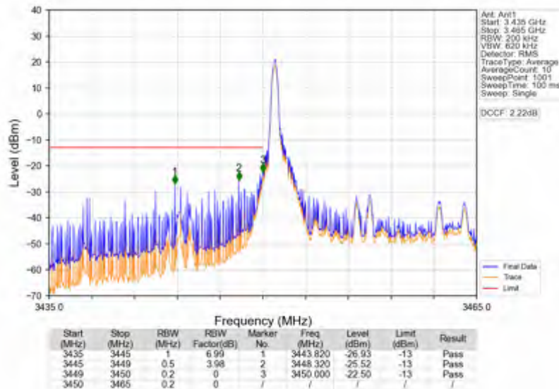
Band42a_15MHz_64QAM_LCH_3457.5MHz_RB_1_0_NTNV
