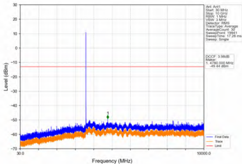
Band42c_10MHz_64QAM_HCH_3595MHz_RB_1_0_NTNV
