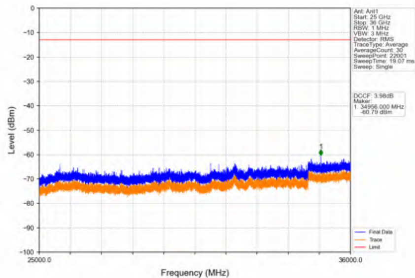
Band42c_15MHz_QPSK_LCH_3557.5MHz_RB_1_0_NTNV
