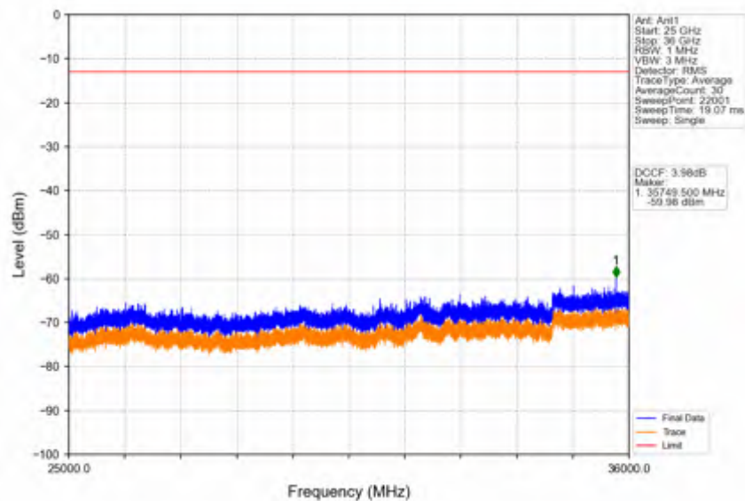
Band42c_20MHz_16QAM_HCH_3590MHz_RB_1_0_NTNV
