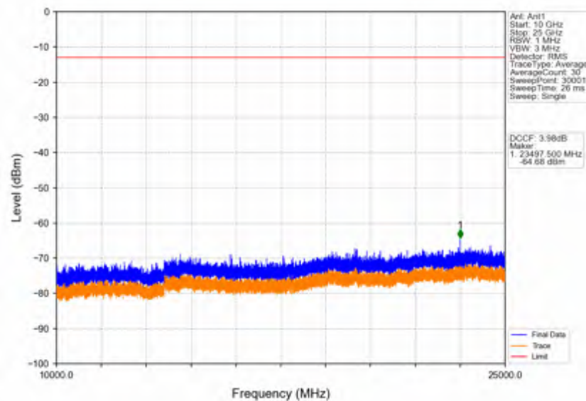
Band42c_5MHz_QPSK_LCH_3552.5MHz_RB_1_0_NTNV
