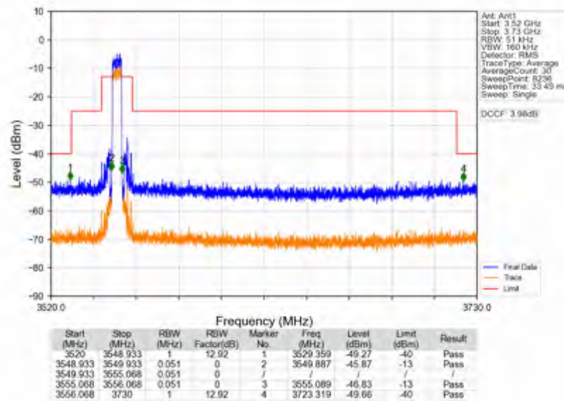
Band42c_5MHz_16QAM_LCH_3552.5MHz_RB_25_0_NTNV
