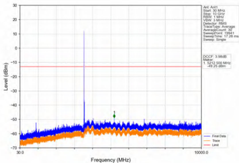
Band42c_15MHz_64QAM_LCH_3557.5MHz_RB_1_0_NTNV
