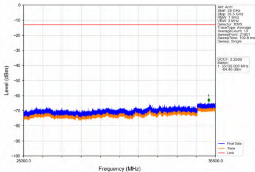
Band42a_15MHz_256QAM_HCH_3542.5MHz_RB_1_0_NTNV
