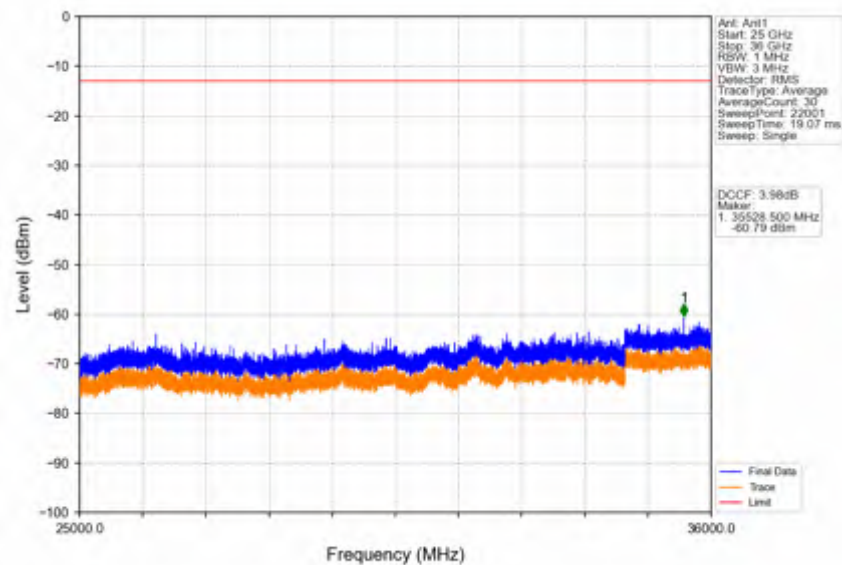
Band42c_5MHz_64QAM_MCH_3575MHz_RB_1_0_NTNV
