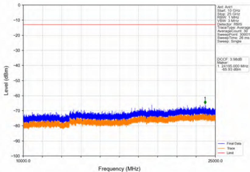
Band42c_20MHz_16QAM_MCH_3575MHz_RB_1_0_NTNV
