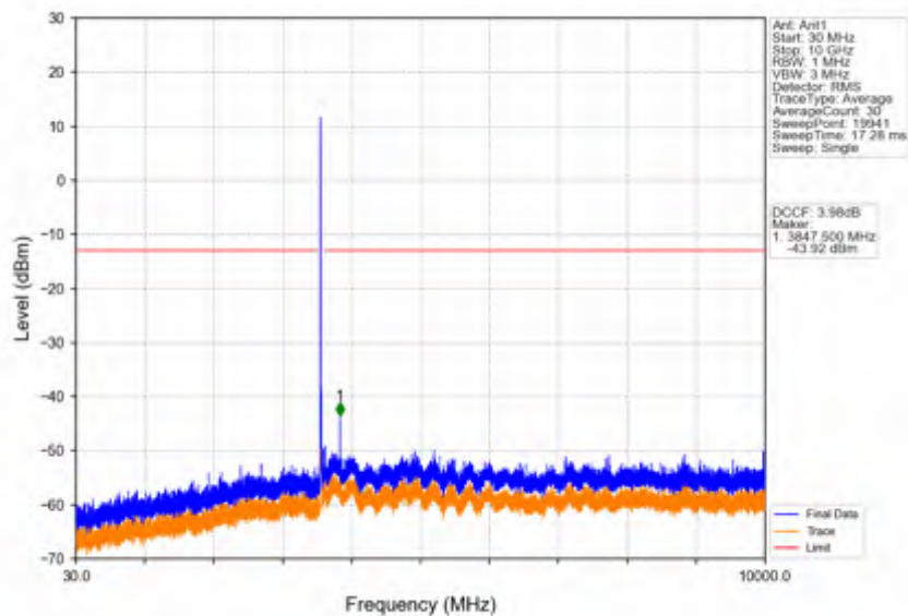
Band42c 20MHz QPSK MCH 3575MHz RB 1 0 NTNV
