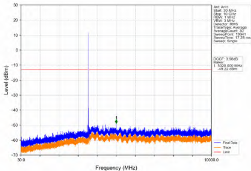
Band42c_15MHz_256QAM_LCH_3557.5MHz_RB_1_0_NTNV
