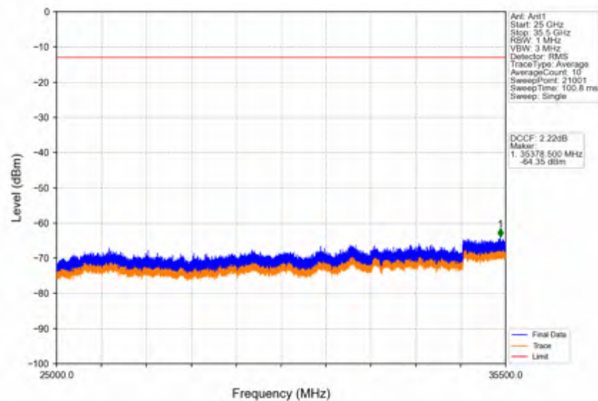
Band42a_10MHz_16QAM_HCH_3545MHz_RB_1_0_NTNV
