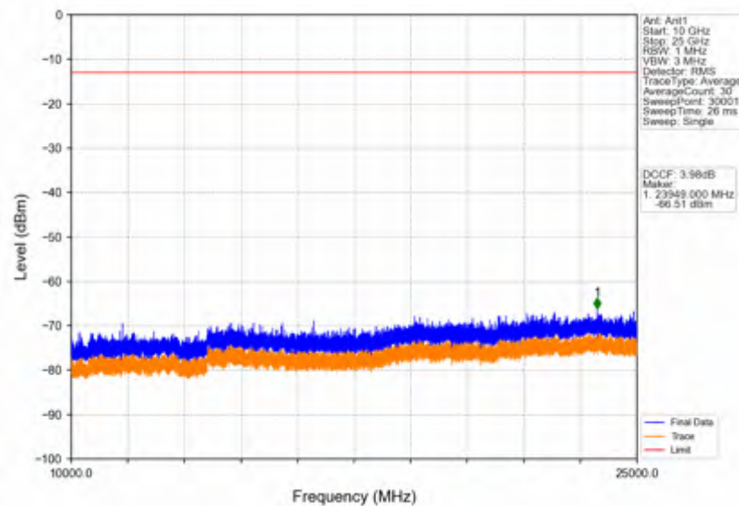
Band42c_15MHz_QPSK_MCH_3575MHz_RB_1_0_NTNV
