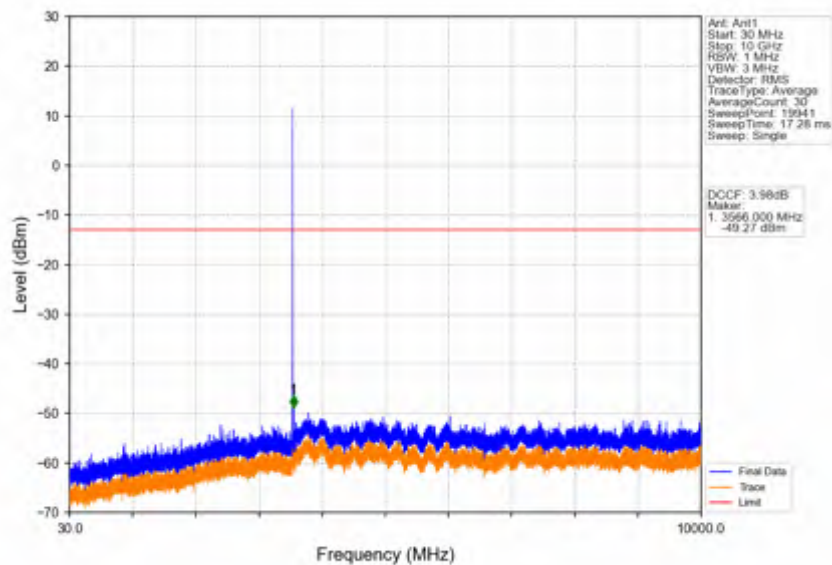
Band42c_5MHz_256QAM_LCH_3552.5MHz_RB_1_0_NTNV
