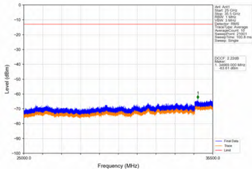
Band42a_10MHz_256QAM_HCH_3545MHz_RB_1_0_NTNV
