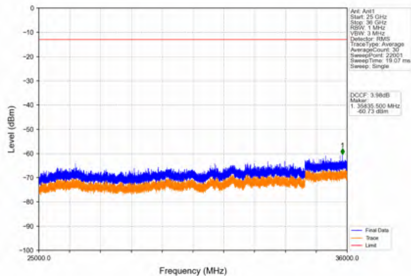
Band42c_5MHz_16QAM_LCH_3552.5MHz_RB_25_0_NTNV
