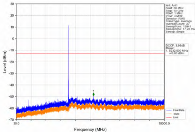
Band42c_5MHz_16QAM_LCH_3552.5MHz_RB_1_0_NTNV
