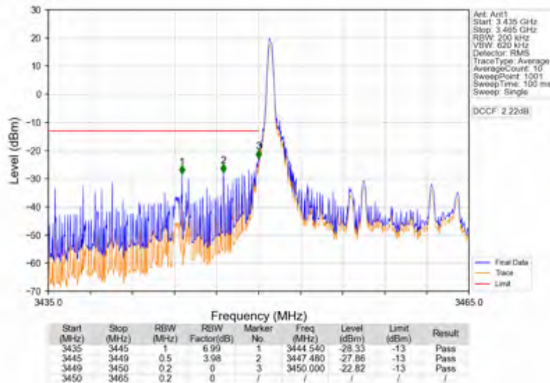
Band42a_15MHz_64QAM_LCH_3457.5MHz_RB_75_0_NTNV
