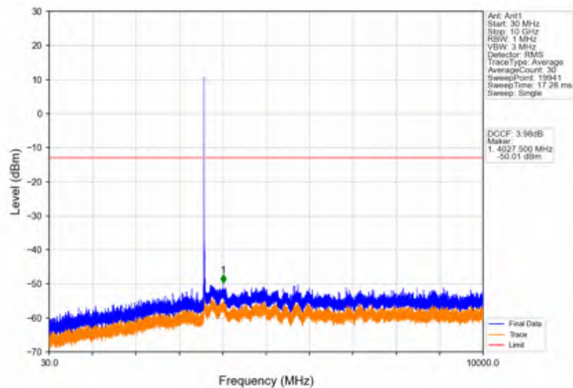
Band42c_15MHz_16QAM_HCH_3592.5MHz_RB_1_0_NTNV
