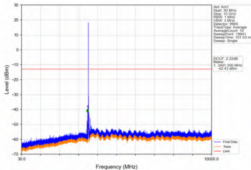
Band42a_15MHz_256QAM_HCH_3542.5MHz_RB_1_0_NTNV
