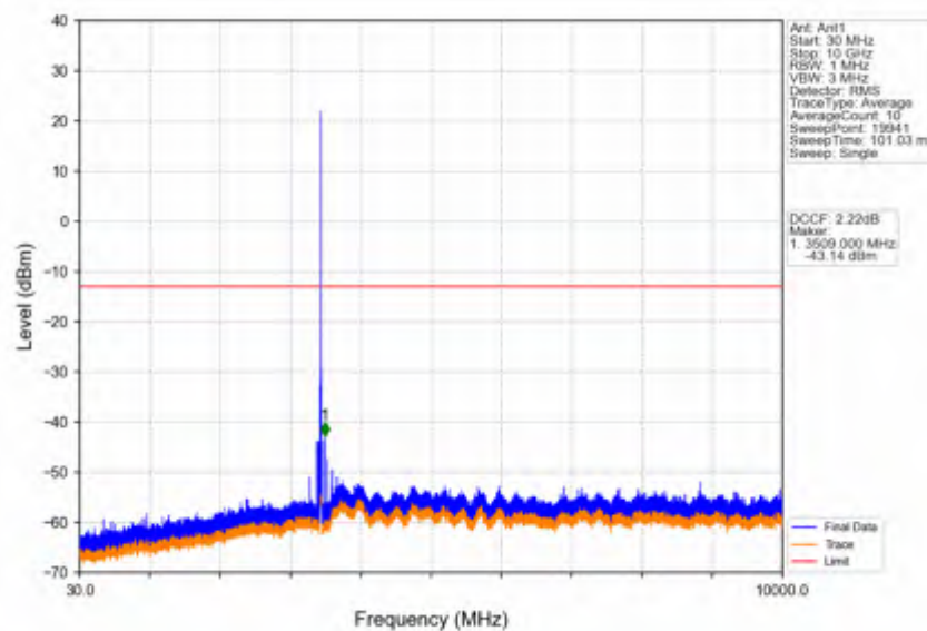
Band42a_10MHz_64QAM_LCH_3455MHz_RB_1_0_NTNV
