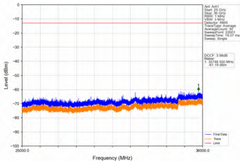
Band42c_10MHz_64QAM_MCH_3575MHz_RB_1_0_NTNV
