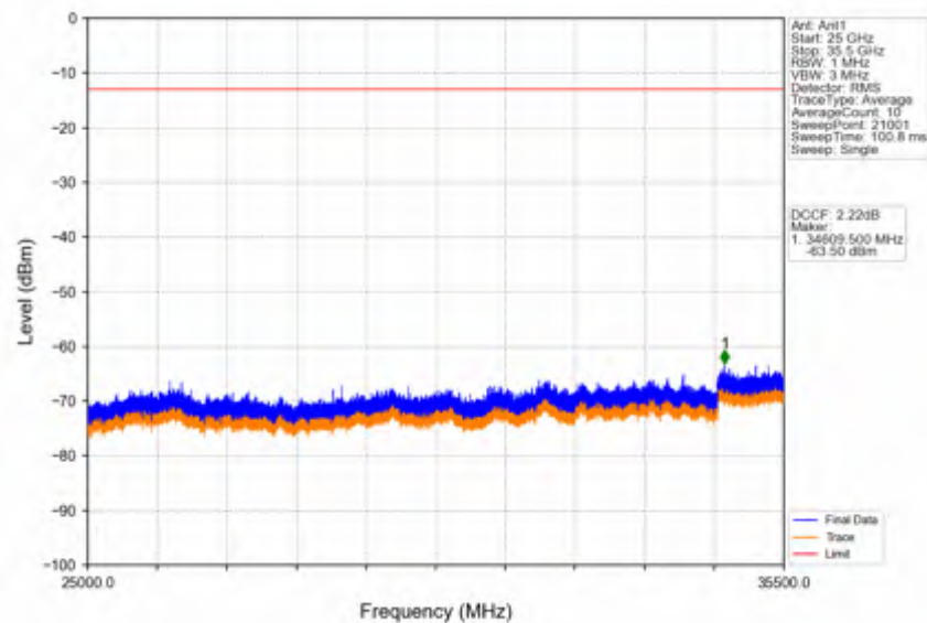
Band42a_15MHz_QPSK_HCH_3542.5MHz_RB_1_74_NTNV
