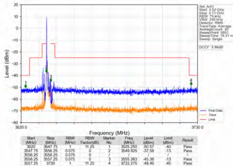
Band42c_5MHz_16QAM_LCH_3552.5MHz_RB_1_0_NTNV
