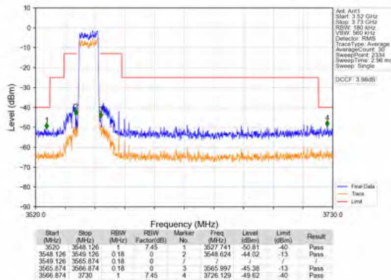
Band42c_15MHz_16QAM_LCH_3557.5MHz_RB_75_0_NTNV
