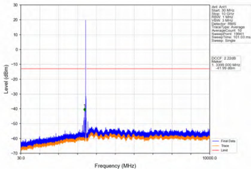
Band42a_15MHz_16QAM_LCH_3457.5MHz_RB_1_0_NTNV
