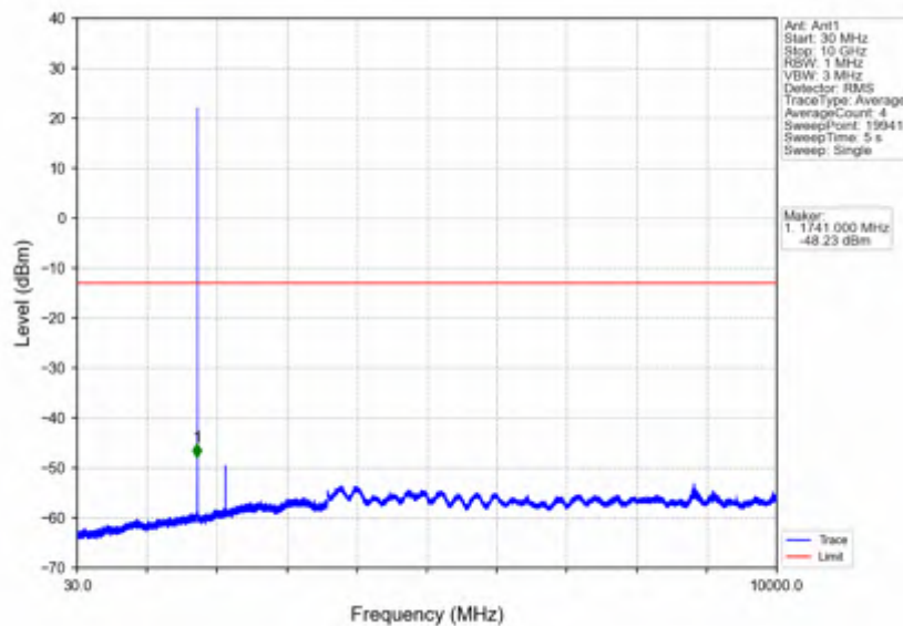
Band66_1.4MHz_16QAM_MCH_1745MHz_RB_1_0_NTNV
