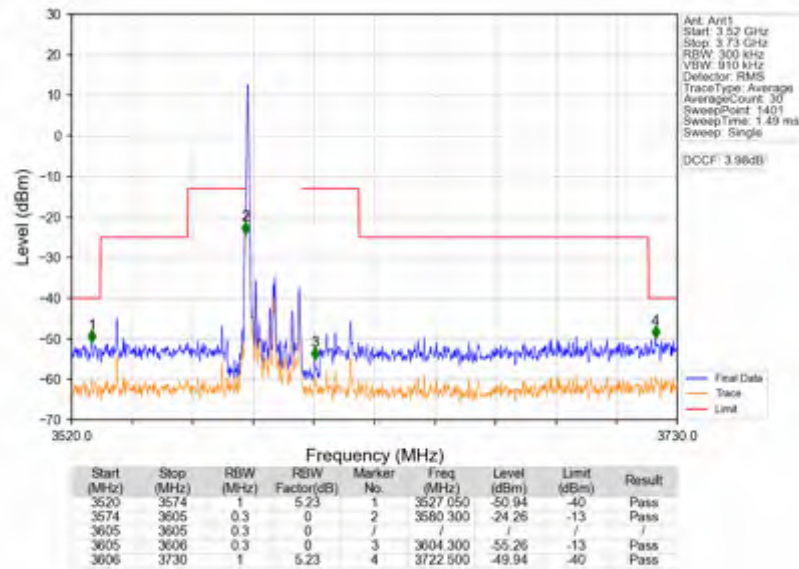
Band42c_20MHz_64QAM_HCH_3590MHz_RB_1_99_NTNV
