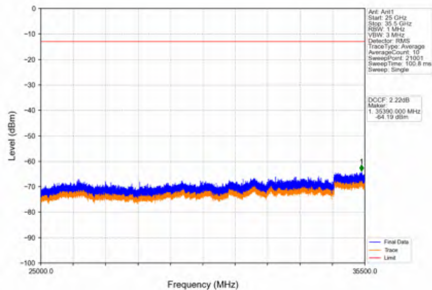
Band42a_10MHz_64QAM_LCH_3455MHz_RB_1_0_NTNV
