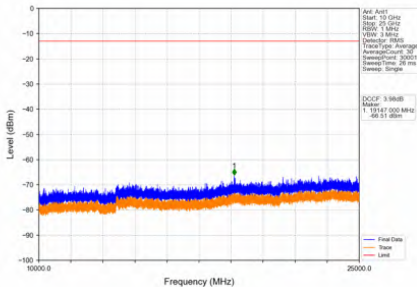
Band42c_10MHz_256QAM_MCH_3575MHz_RB_1_0_NTNV
