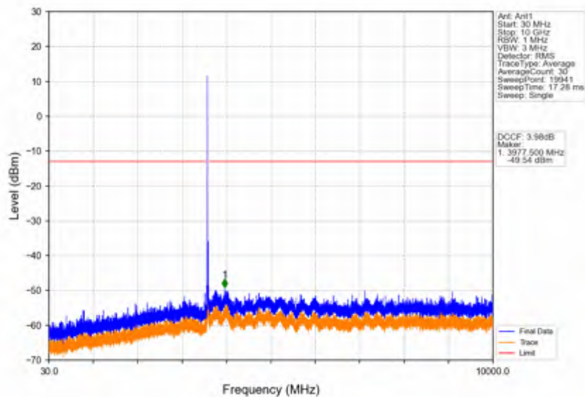
Band42c_15MHz_64QAM_HCH_3592.5MHz_RB_1_0_NTNV
