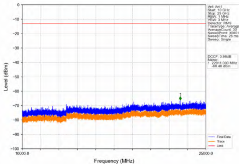
Band42c_20MHz_64QAM_HCH_3590MHz_RB_1_0_NTNV
