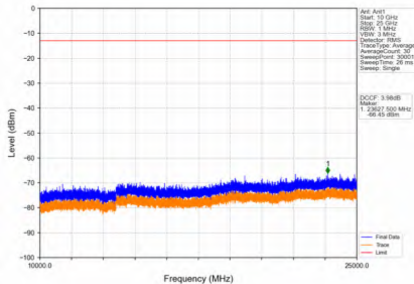
Band42c_15MHz_64QAM_LCH_3557.5MHz_RB_1_0_NTNV
