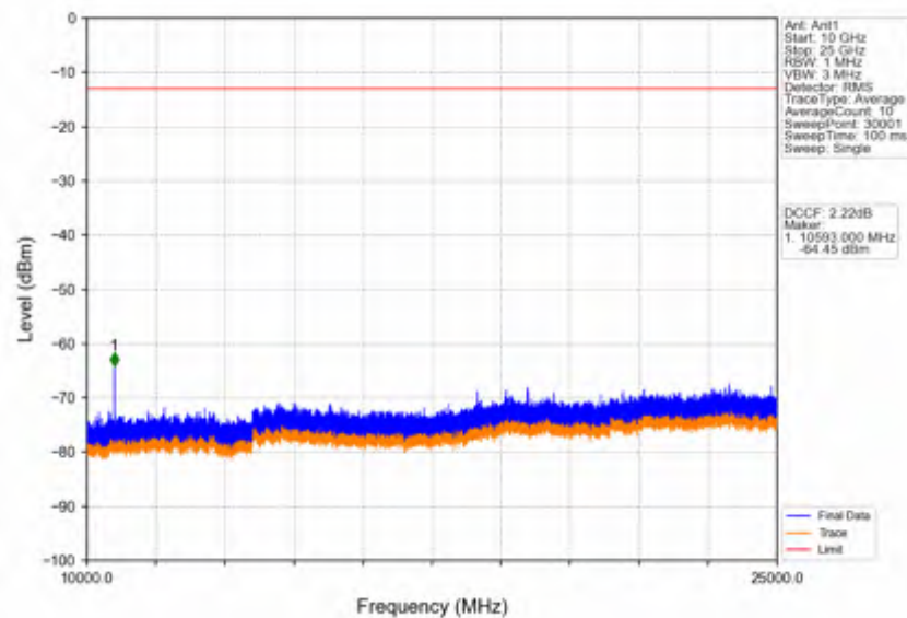
Band42a_20MHz_256QAM_HCH_3540MHz_RB_1_0_NTNV
