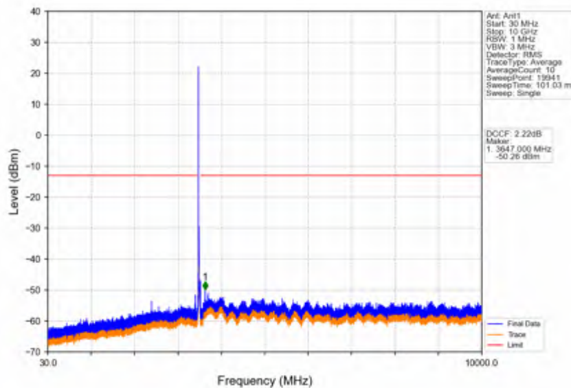
Band42a_20MHz_64QAM_MCH_3500MHz_RB_1_0_NTNV
