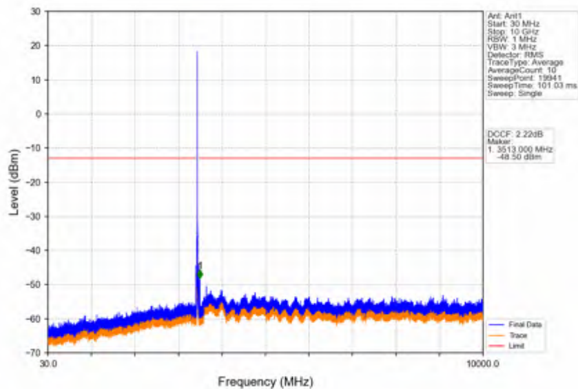
Band42a_15MHz_256QAM_LCH_3457.5MHz_RB_1_0_NTNV
