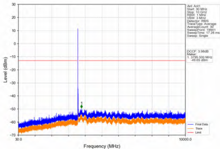
Band42c_20MHz_16QAM_HCH_3590MHz_RB_1_0_NTNV
