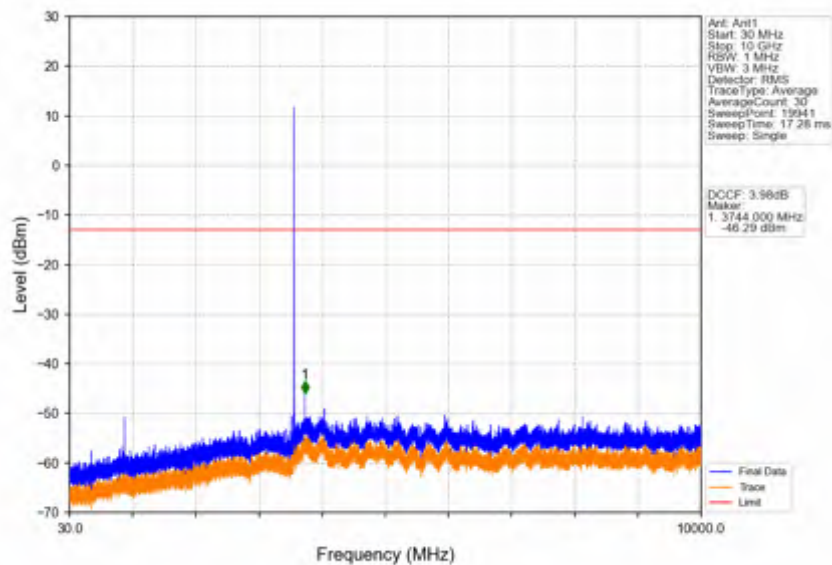
Band42c_5MHz_256QAM_MCH_3575MHz_RB_1_0_NTNV
