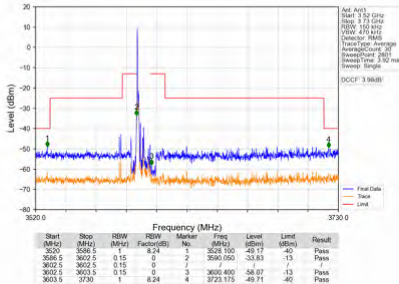
Band42c_10MHz_64QAM_HCH_3595MHz_RB_1_49_NTNV
