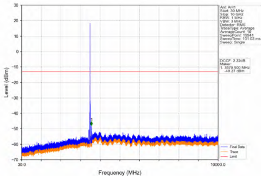
Band42a_10MHz_256QAM_MCH_3500MHz_RB_1_0_NTNV
