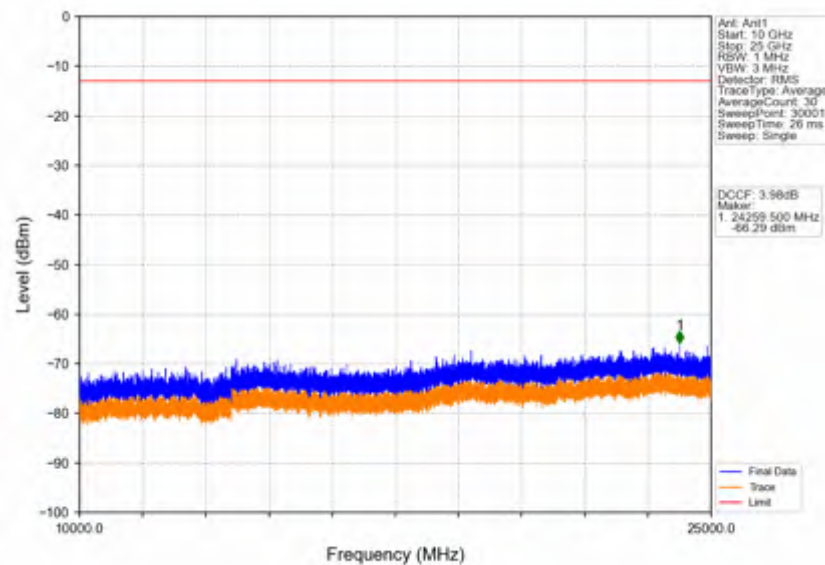
Band42c_20MHz_64QAM_MCH_3575MHz_RB_1_0_NTNV
