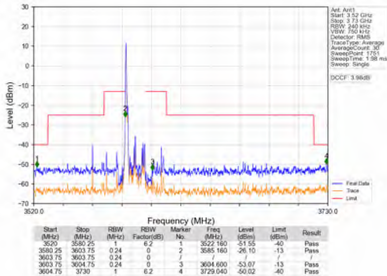
Band42c_15MHz_16QAM_HCH_3592.5MHz_RB_75_0_NTNV
