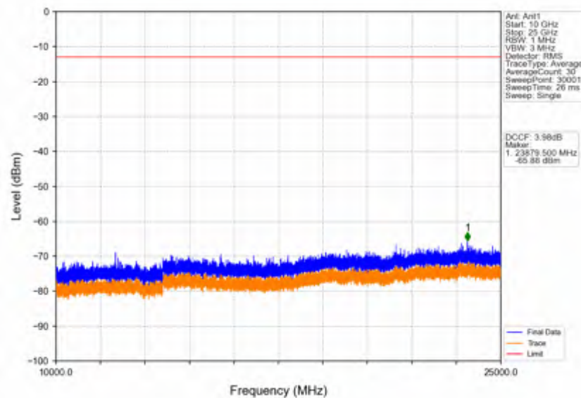
Band42c_15MHz_16QAM_HCH_3592.5MHz_RB_1_0_NTNV
