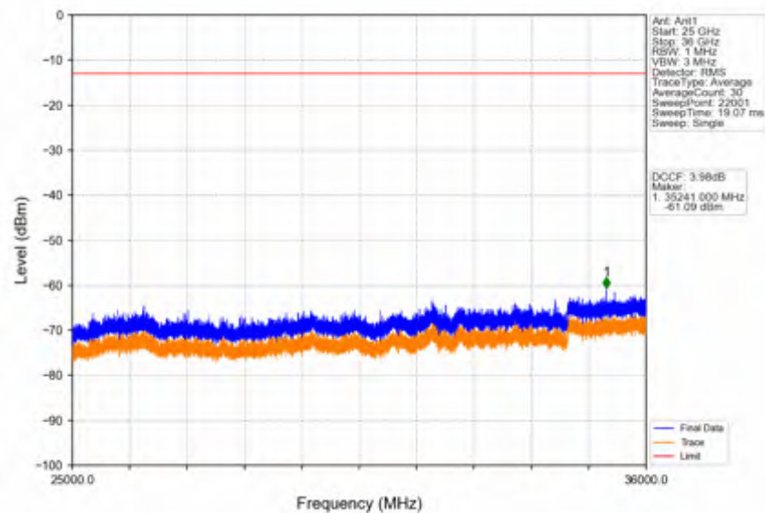
Band42c_5MHz_16QAM_HCH_3597.5MHz_RB_1_0_NTNV
