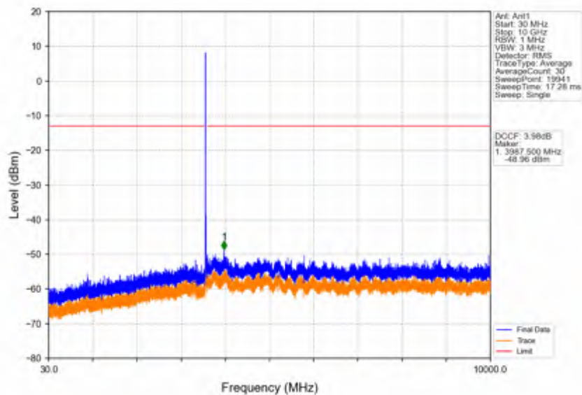
Band42c_15MHz_16QAM_MCH_3575MHz_RB_1_0_NTNV
