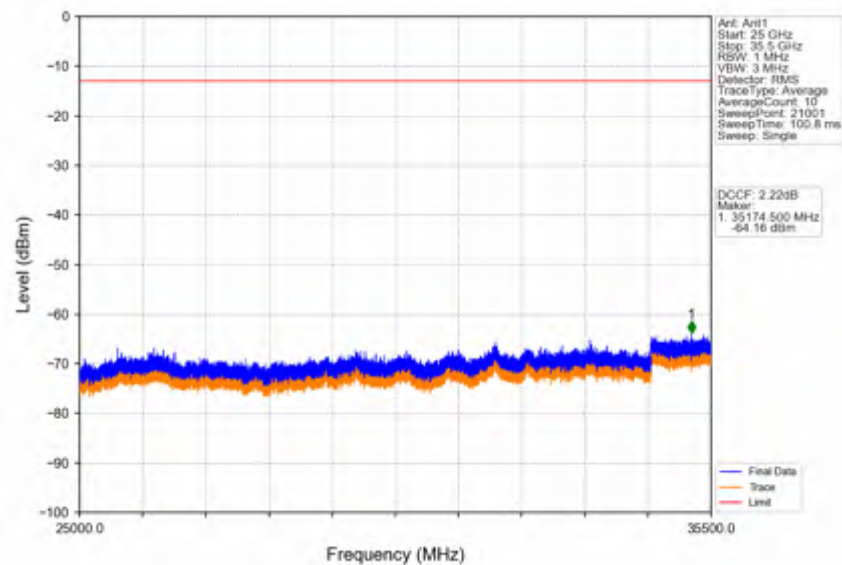
Band42a_10MHz_64QAM_MCH_3500MHz_RB_1_0_NTNV
