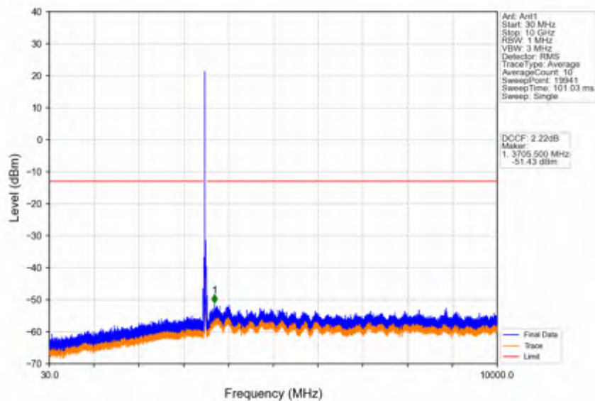
Band42a_20MHz_256QAM_MCH_3500MHz_RB_1_0_NTNV
