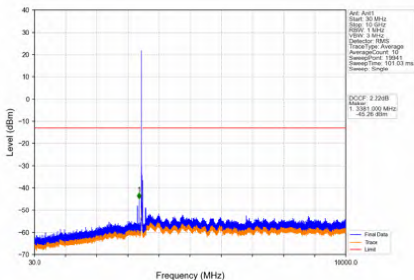
Band42a_15MHz_QPSK_LCH_3457.5MHz_RB_1_0_NTNV
