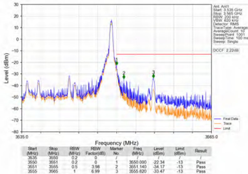
Band42a_15MHz_256QAM_HCH_3542.5MHz_RB_1_74_NTNV
