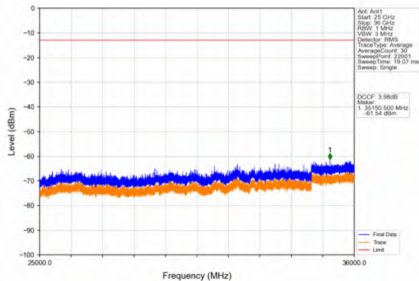
Band42c_5MHz_QPSK_HCH_3597.5MHz_RB_1_24_NTNV
