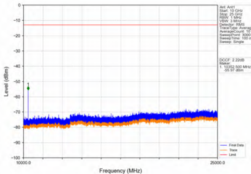
Band42a_15MHz_256QAM_LCH_3457.5MHz_RB_1_0_NTNV
