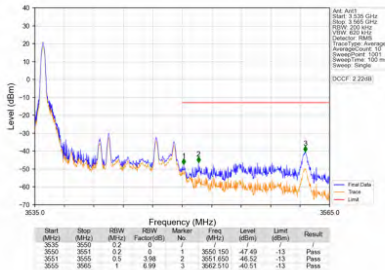
Band42a_15MHz_QPSK_HCH_3542.5MHz_RB_1_74_NTNV
