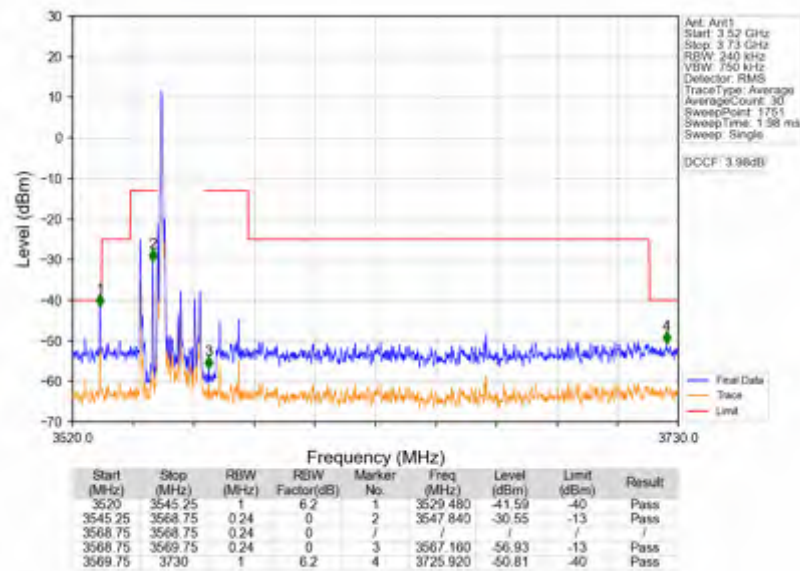
Band42c_15MHz_16QAM_LCH_3557.5MHz_RB_1_0_NTNV
