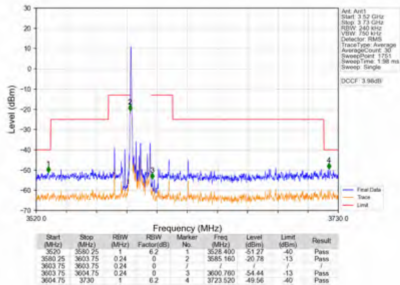
Band42c_15MHz_64QAM_HCH_3592.5MHz_RB_1_74_NTNV
