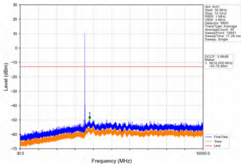
Band42c_15MHz_16QAM_LCH_3557.5MHz_RB_1_0_NTNV
