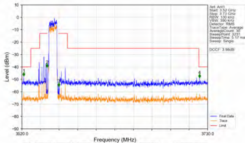
Band42c_10MHz_256QAM_LCH_3555MHz_RB_50_0_NTNV
