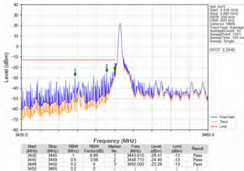
Band42a_15MHz_QPSK_LCH_3457.5MHz_RB_1_0_NTNV
