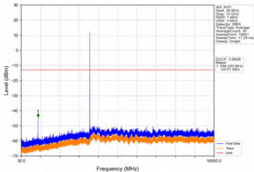
Band42c_5MHz_64QAM_MCH_3575MHz_RB_1_0_NTNV
