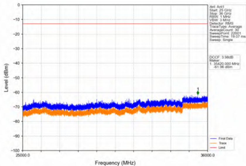
Band42c_5MHz_16QAM_HCH_3597.5MHz_RB_1_0_NTNV
