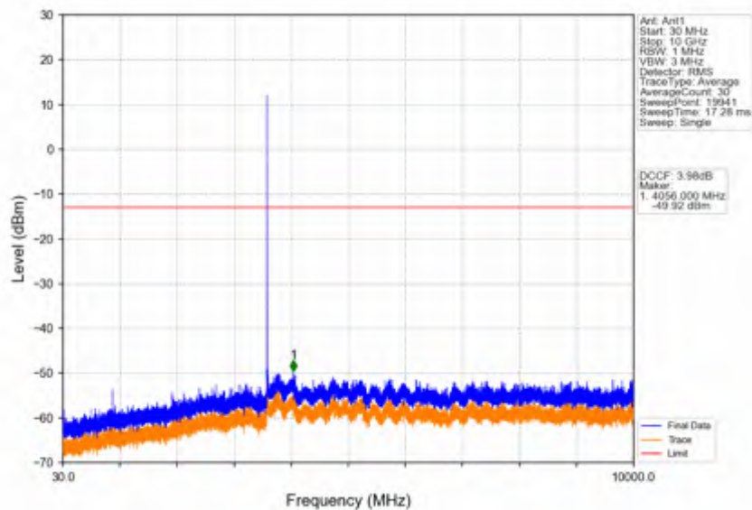
Band42c_5MHz_64QAM_HCH_3597.5MHz_RB_1_0_NTNV
