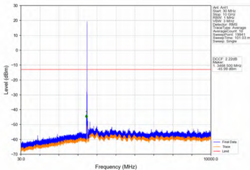
Band42a_10MHz_64QAM_MCH_3500MHz_RB_1_0_NTNV
