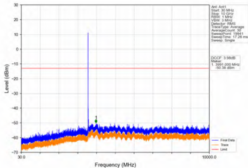
Band42c_15MHz_64QAM_MCH_3575MHz_RB_1_0_NTNV
