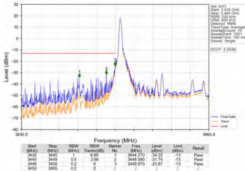
Band42a_15MHz_256QAM_LCH_3457.5MHz_RB_1_0_NTNV
