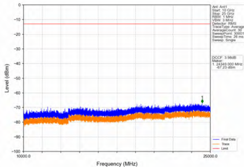
Band42c_5MHz_QPSK_MCH_3575MHz_RB_1_0_NTNV
