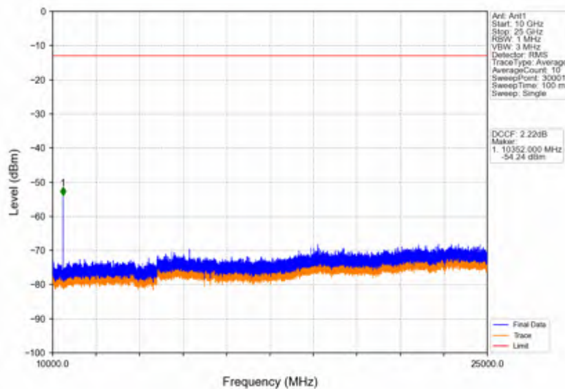
Band42a_15MHz_16QAM_LCH_3457.5MHz_RB_1_0_NTNV
