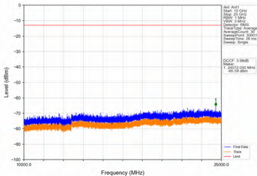
Band42c_15MHz_QPSK_HCH_3592.5MHz_RB_1_0_NTNV
