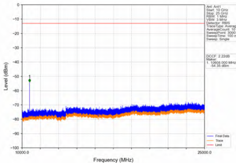
Band42a_15MHz_QPSK_HCH_3542.5MHz_RB_1_0_NTNV
