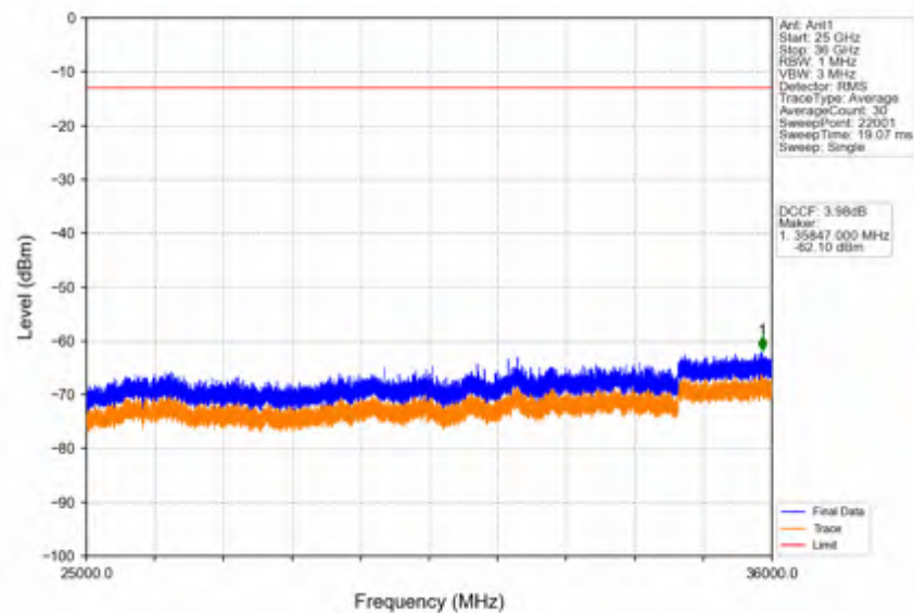
Band42c_5MHz_256QAM_HCH_3597.5MHz_RB_1_0_NTNV
