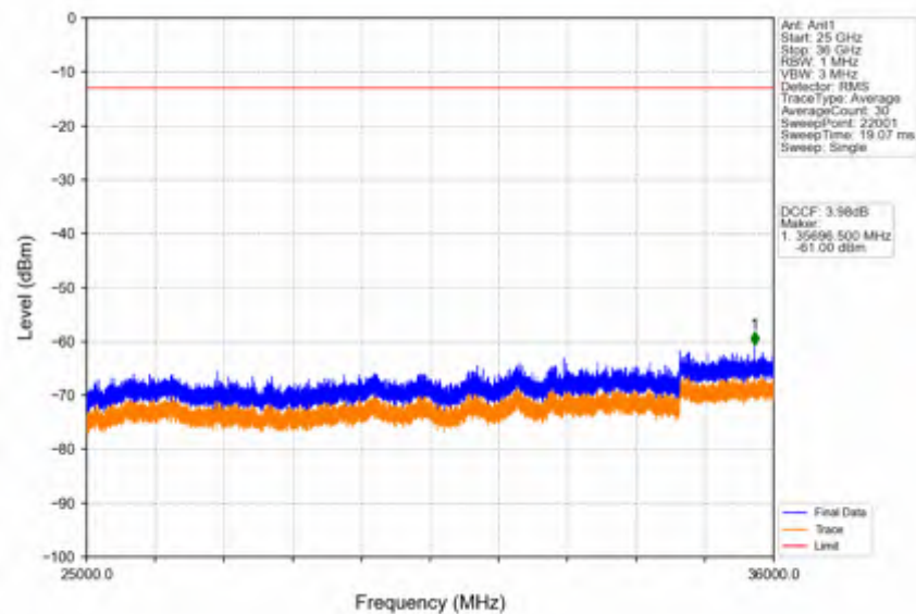
Band42c_15MHz_64QAM_MCH_3575MHz_RB_1_0_NTNV
