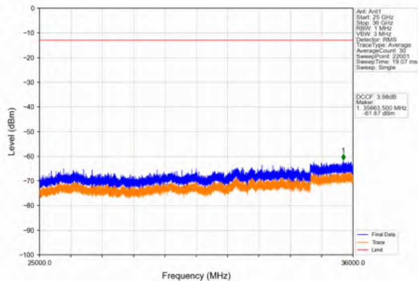
Band42c_10MHz_256QAM_LCH_3555MHz_RB_50_0_NTNV
