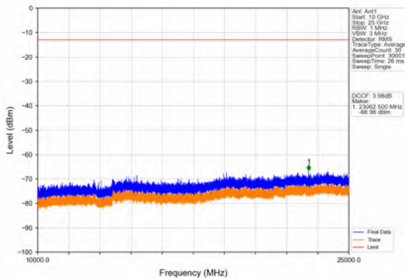
Band42c_5MHz_QPSK_HCH_3597.5MHz_RB_1_0_NTNV
