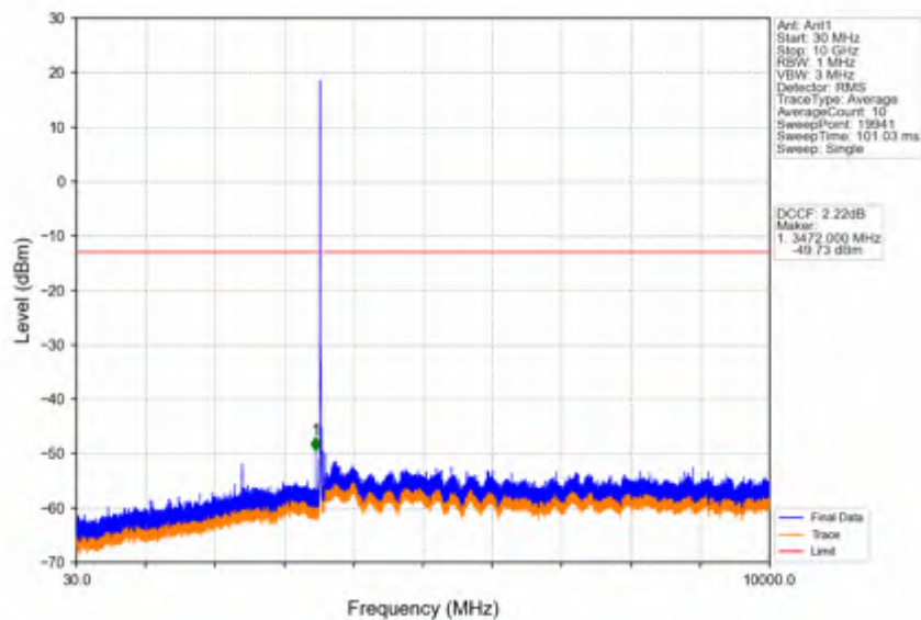
Band42a_15MHz_64QAM_HCH_3542.5MHz_RB_1_0_NTNV
