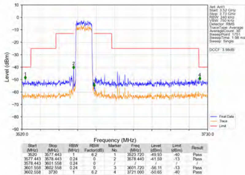
Band42c_20MHz_256QAM_HCH_3590MHz_RB_100_0_NTNV
