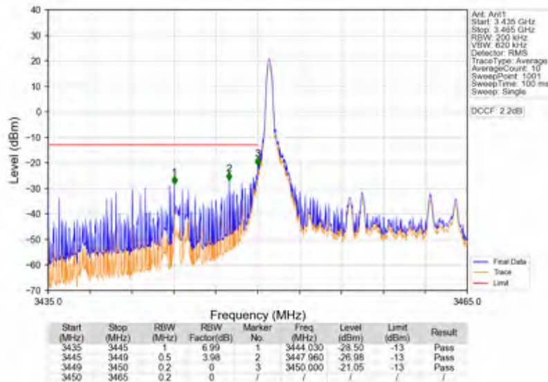
Band42a_15MHz_QPSK_LCH_3457.5MHz_RB_75_0_NTNV
