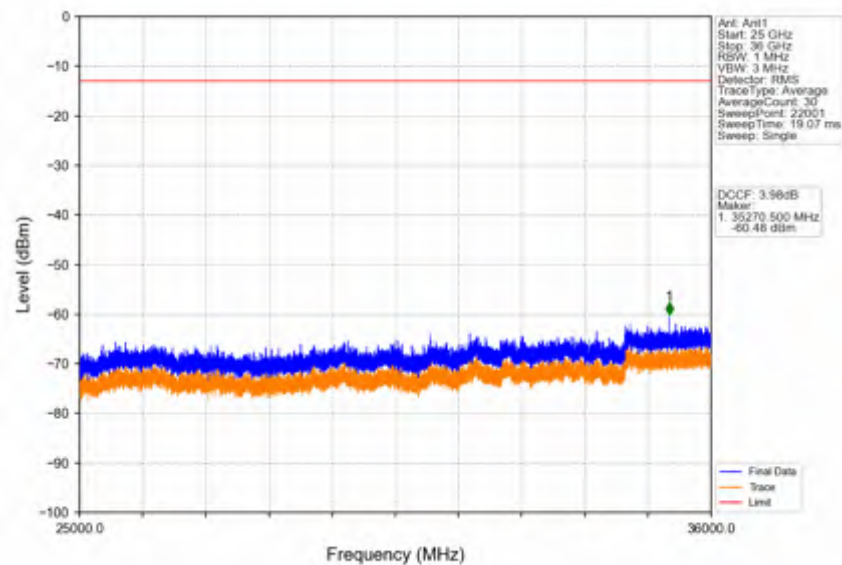
Band42c_20MHz_64QAM_MCH_3575MHz_RB_1_0_NTNV
