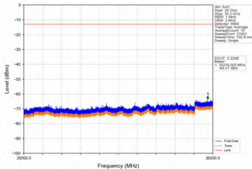
Band42a_20MHz_256QAM_HCH_3540MHz_RB_1_0_NTNV
