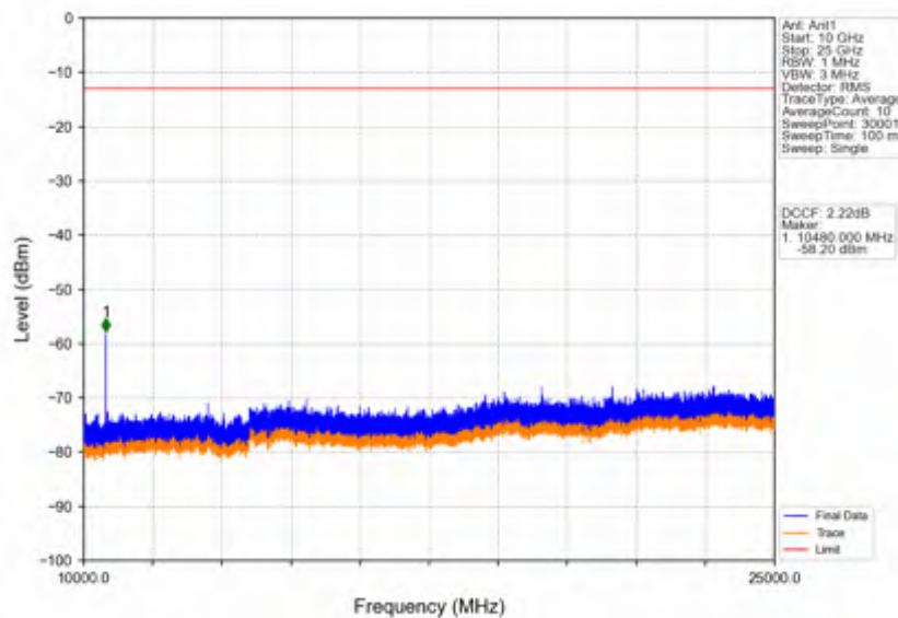
Band42a_15MHz_256QAM_MCH_3500MHz_RB_1_0_NTNV
