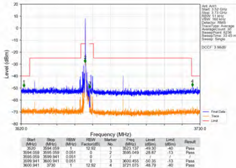
Band42c_5MHz_16QAM_HCH_3597.5MHz_RB_25_0_NTNV
