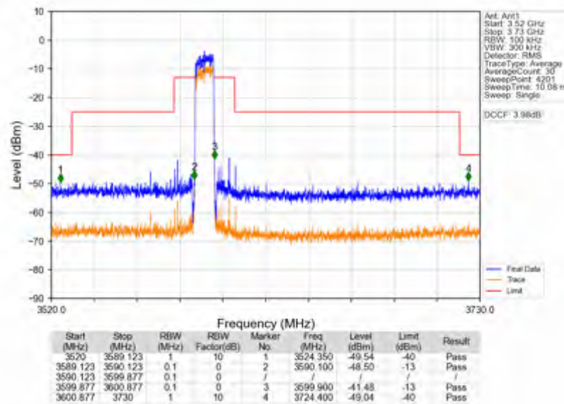
Band42c_10MHz_256QAM_HCH_3595MHz_RB_50_0_NTNV
