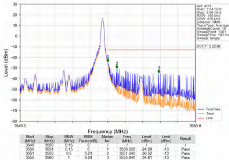
Band42a_10MHz_256QAM_HCH_3545MHz_RB_1_49_NTNV
