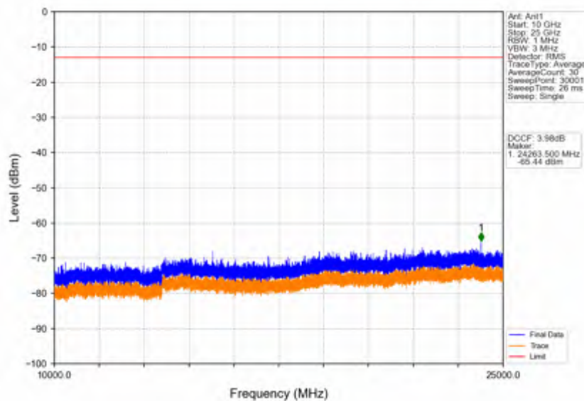
Band42c_5MHz_256QAM_LCH_3552.5MHz_RB_1_0_NTNV
