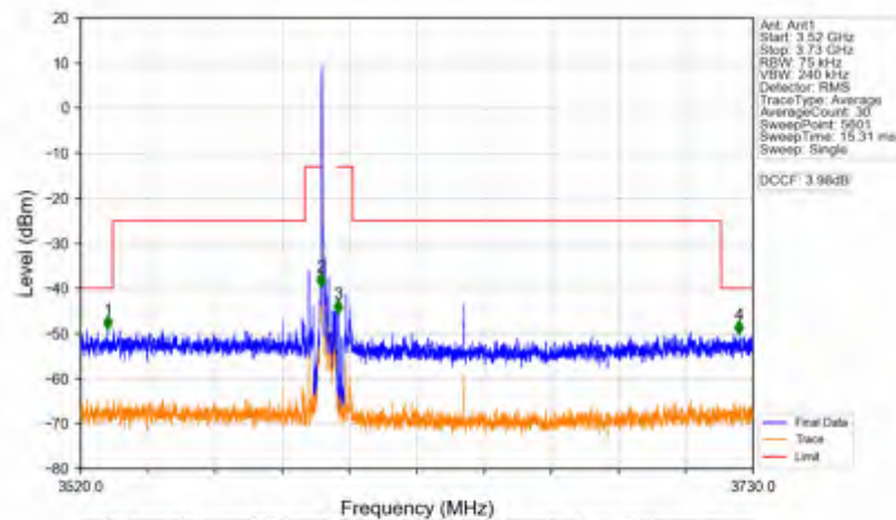
Band42c_5MHz_QPSK_HCH_3597.5MHz_RB_1_24_NTNV
