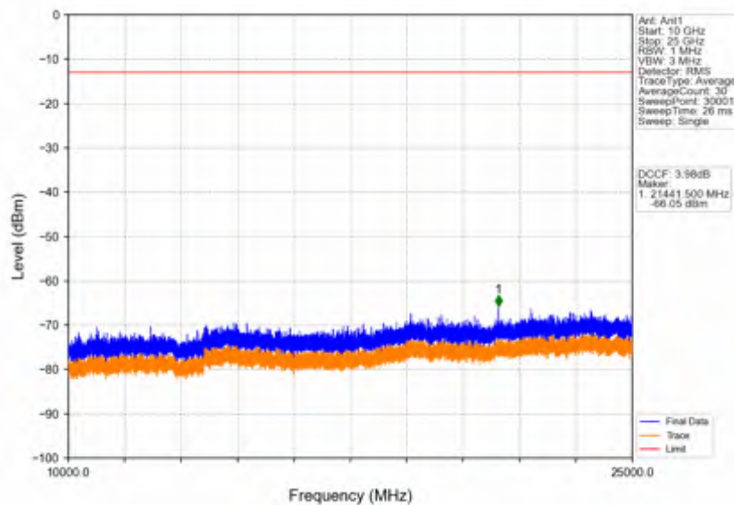
Band42c_15MHz_16QAM_LCH_3557.5MHz_RB_1_0_NTNV
