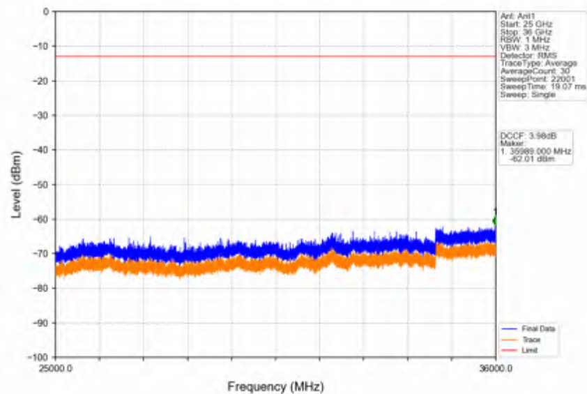
Band42c_5MHz_QPSK_MCH_3575MHz_RB_1_0_NTNV
