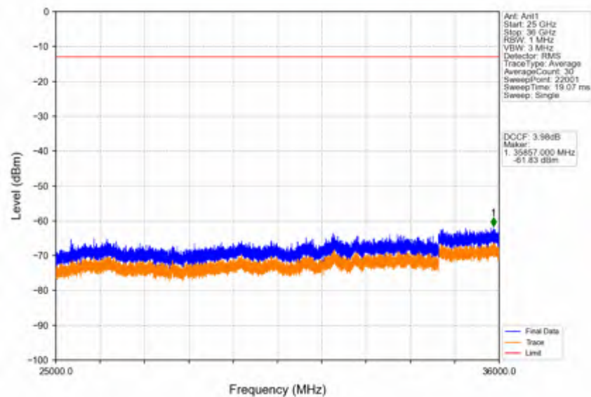
Band42c_15MHz_256QAM_HCH_3592.5MHz_RB_1_0_NTNV
