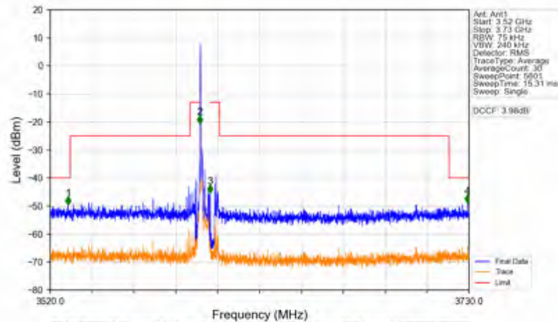
Band42c_5MHz_64QAM_HCH_3597.5MHz_RB_1_24_NTNV
