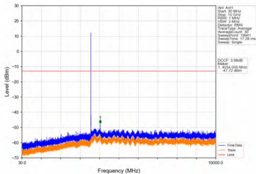
Band42c_10MHz_64QAM_MCH_3575MHz_RB_1_0_NTNV
