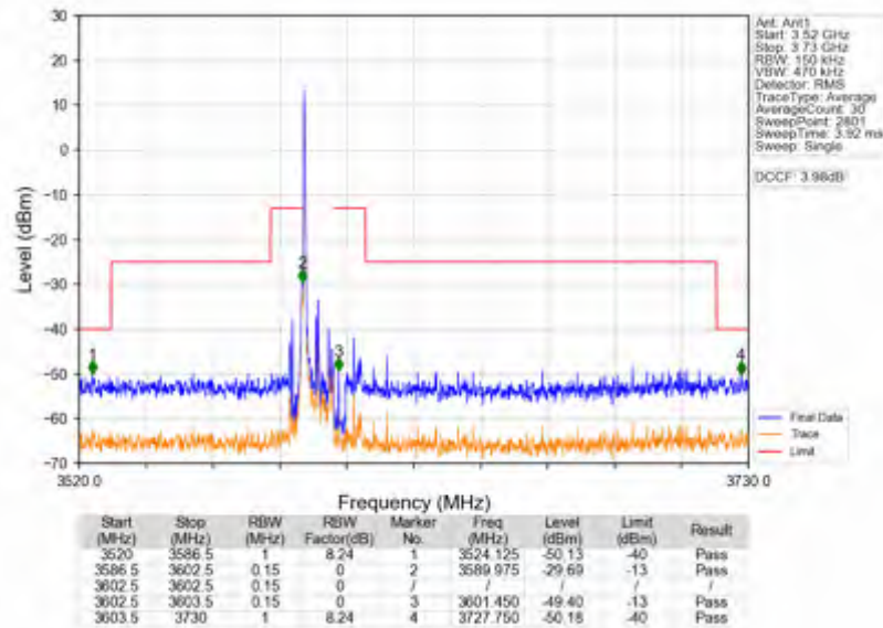
Band42c_10MHz_16QAM_HCH_3595MHz_RB_50_0_NTNV
