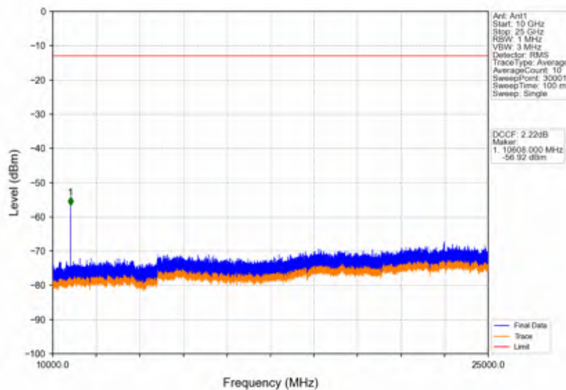
Band42a_15MHz_64QAM_HCH_3542.5MHz_RB_1_0_NTNV
