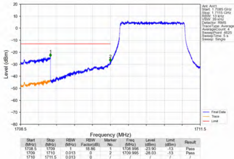
Band66_1.4MHz_16QAM_LCH_1710.7MHz_RB_1_0_NTNV
