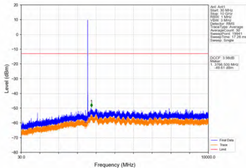
Band42c_15MHz_QPSK_MCH_3575MHz_RB_1_0_NTNV
