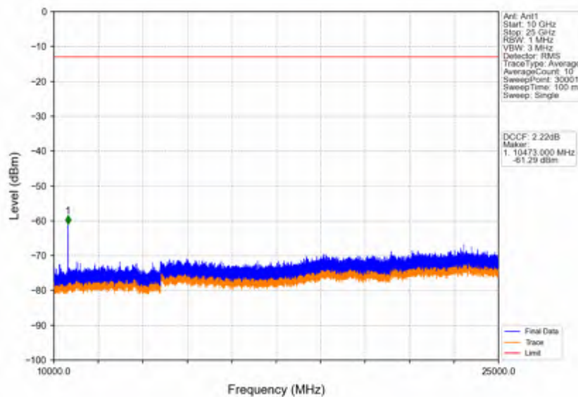
Band42a_20MHz_256QAM_MCH_3500MHz_RB_1_0_NTNV
