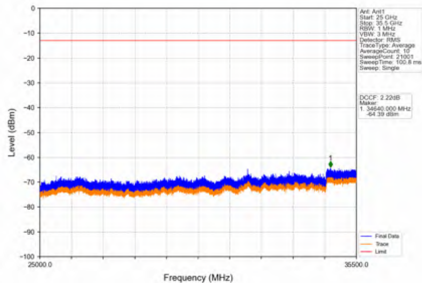
Band42a_15MHz_16QAM_HCH_3542.5MHz_RB_1_0_NTNV
