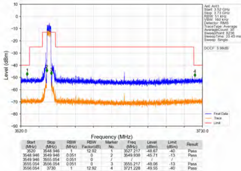
Band42c_5MHz_64QAM_MCH_3575MHz_RB_1_0_NTNV
