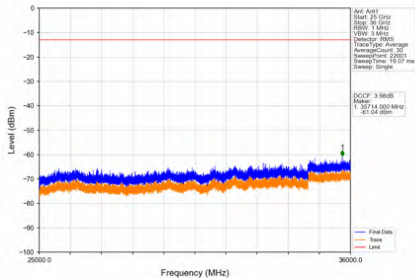
Band42c_15MHz_QPSK_MCH_3575MHz_RB_1_0_NTNV
