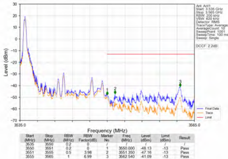
Band42a_15MHz_16QAM_HCH_3542.5MHz_RB_75_0_NTNV
