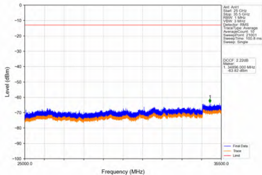
Band42a_15MHz_256QAM_HCH_3542.5MHz_RB_1_0_NTNV
