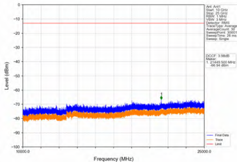
Band42c_10MHz_64QAM_LCH_3555MHz_RB_1_0_NTNV
