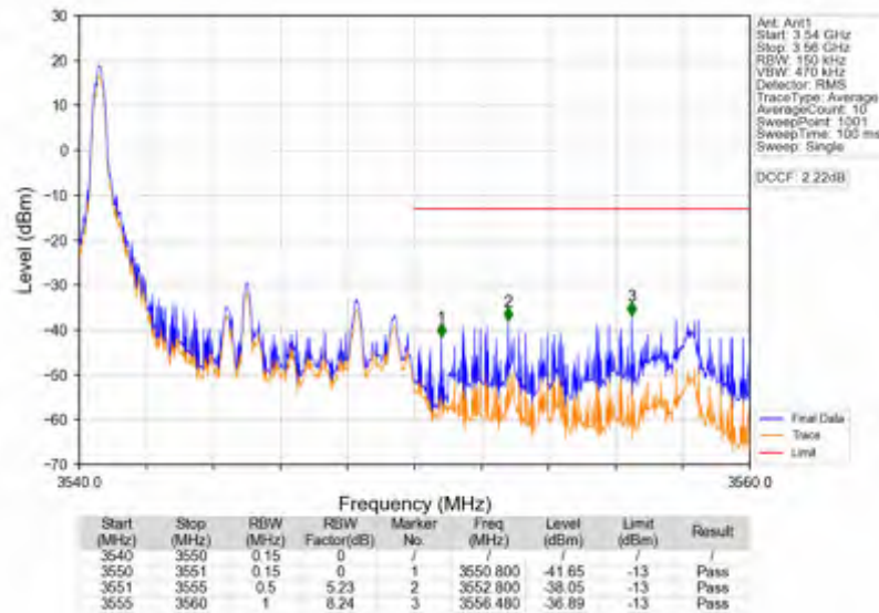
Band42a_10MHz_64QAM_HCH_3545MHz_RB_1_49_NTNV
