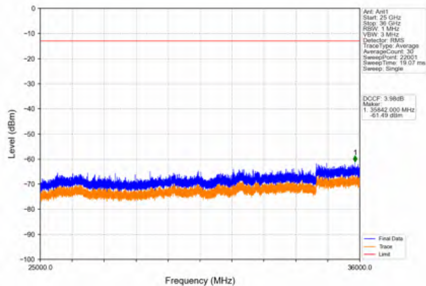
Band42c_10MHz_16QAM_HCH_3595MHz_RB_1_0_NTNV
