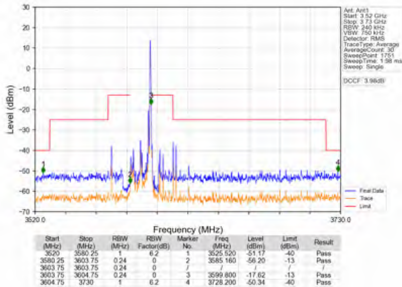
Band42c_15MHz_256QAM_HCH_3592.5MHz_RB_75_0_NTNV
