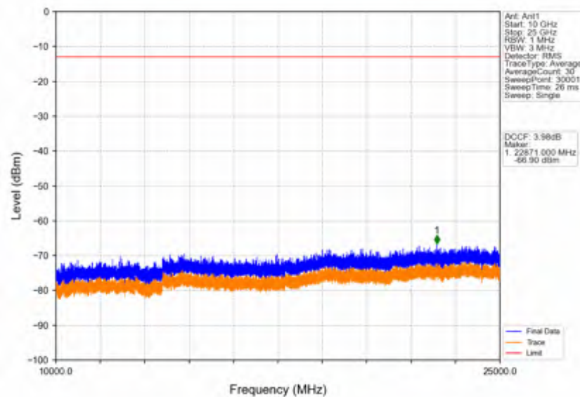
Band42c_5MHz_64QAM_LCH_3552.5MHz_RB_1_0_NTNV
