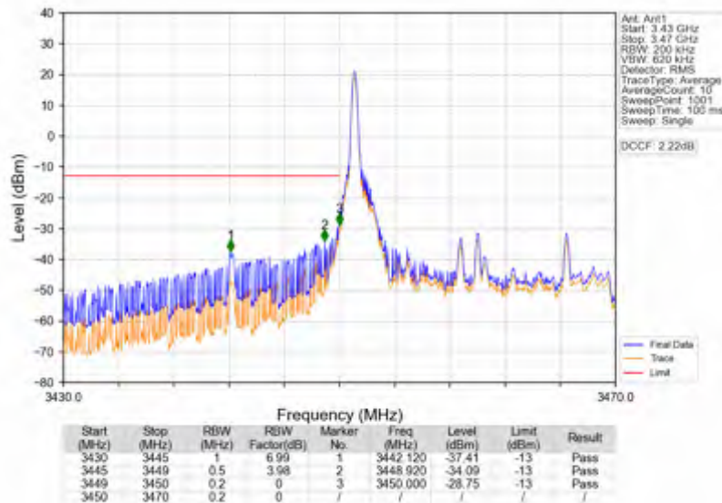
Band42a_20MHz_64QAM_LCH_3460MHz_RB_100_0_NTNV
