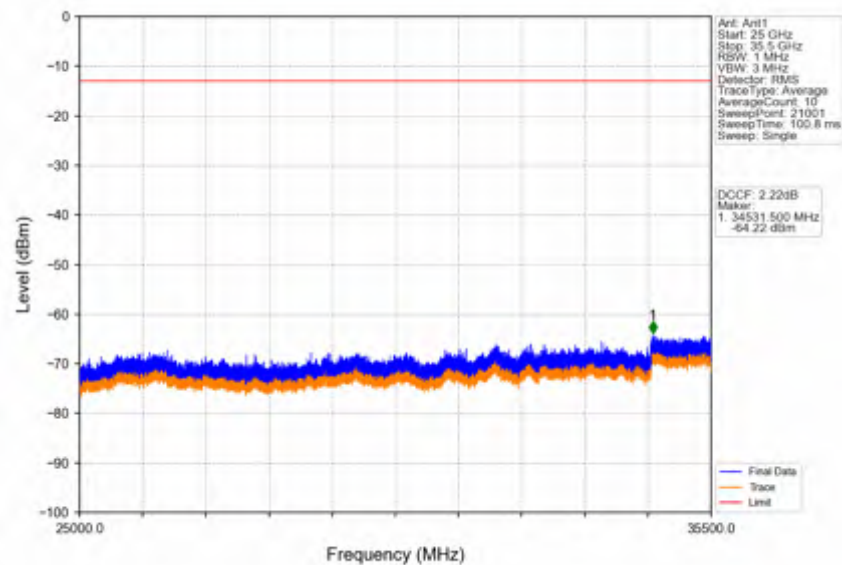
Band42a_20MHz_16QAM_HCH_3540MHz_RB_1_0_NTNV
