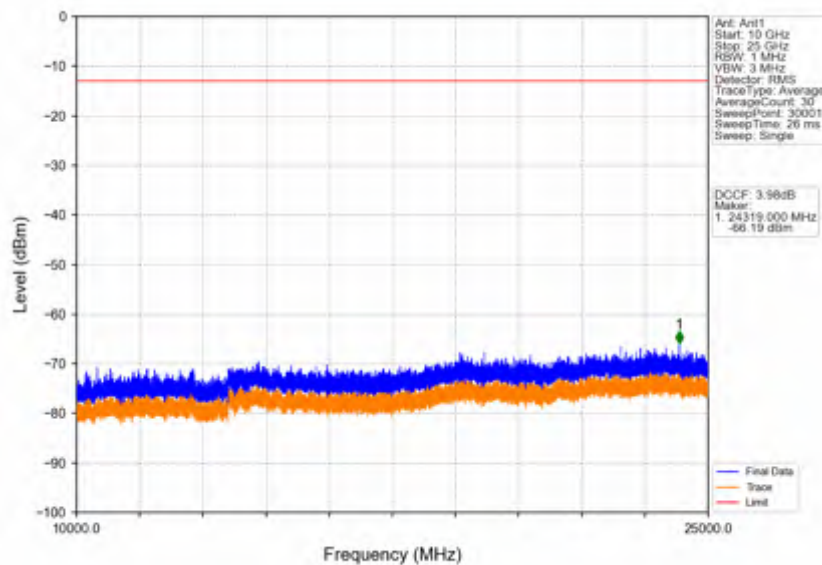
Band42c_5MHz_64QAM_HCH_3597.5MHz_RB_1_0_NTNV
