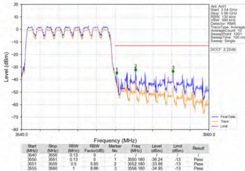
Band42a_10MHz_256QAM_HCH_3545MHz_RB_50_0_NTNV
