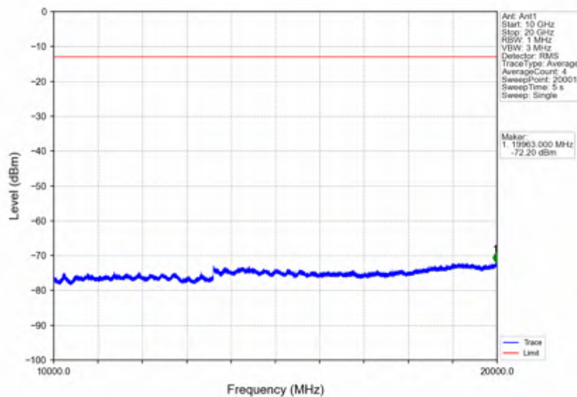
Band66 1.4MHz 16QAM HCH 1779.3MHz RB 1 0 NTNV
