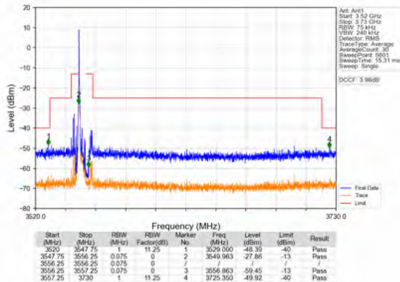
Band42c_5MHz_QPSK_LCH_3552.5MHz_RB_1_0_NTNV
