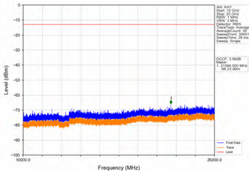
Band42c_20MHz_256QAM_MCH_3575MHz_RB_1_0_NTNV
