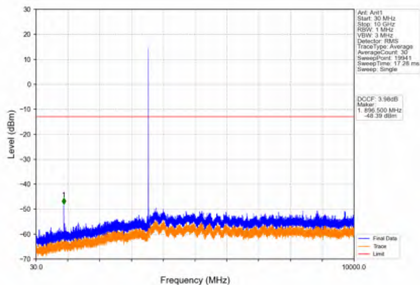
Band42c_5MHz_QPSK_LCH_3552.5MHz_RB_1_0_NTNV
