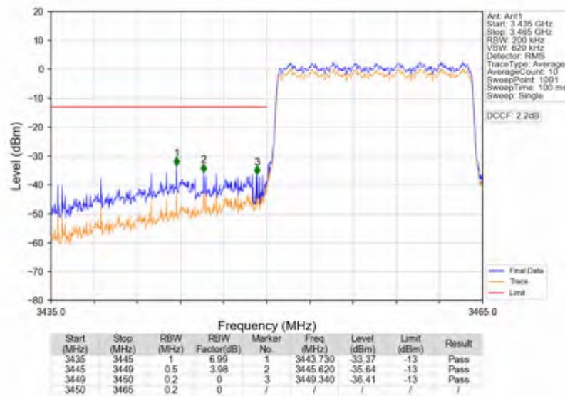
Band42a_15MHz_256QAM_LCH_3457.5MHz_RB_75_0_NTNV
