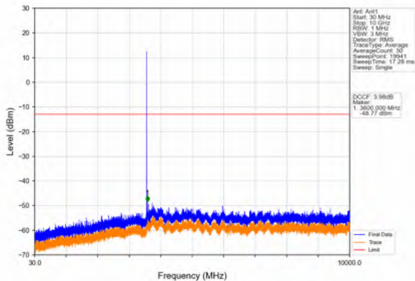
Band42c_5MHz_16QAM_MCH_3575MHz_RB_1_0_NTNV
