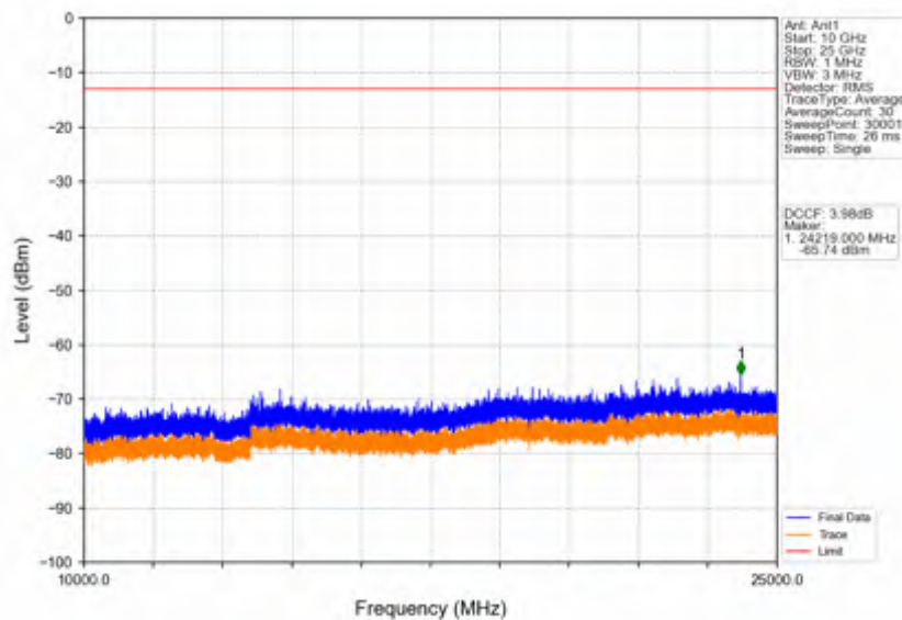
Band42c_15MHz_16QAM_MCH_3575MHz_RB_1_0_NTNV
