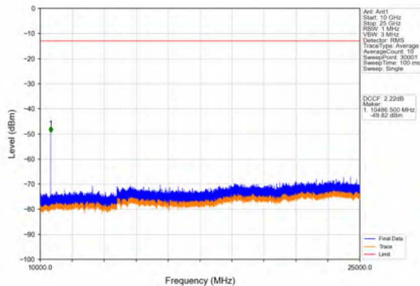
Band42a_10MHz_64QAM_MCH_3500MHz_RB_1_0_NTNV
