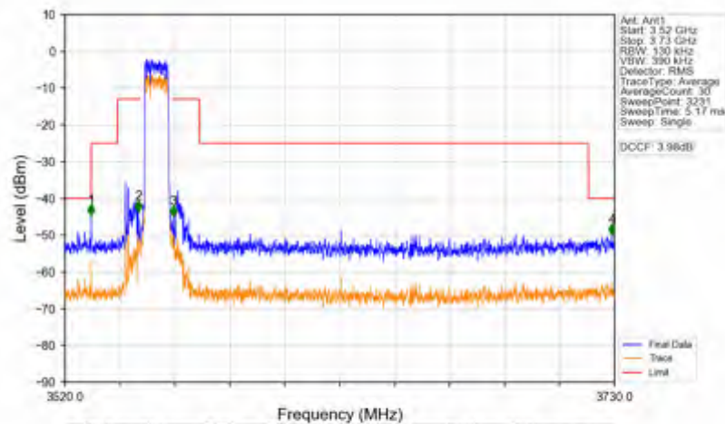
Band42c_10MHz_16QAM_LCH_3555MHz_RB_50_0_NTNV
