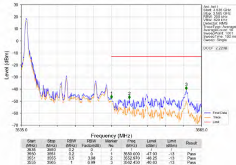
Band42a_15MHz_64QAM_HCH_3542.5MHz_RB_1_74_NTNV
