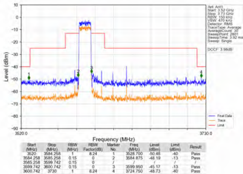
Band42c_15MHz_256QAM_HCH_3592.5MHz_RB_75_0_NTNV
