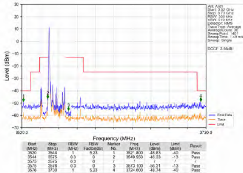
Band42c_20MHz_64QAM_LCH_3560MHz_RB_1_0_NTNV
