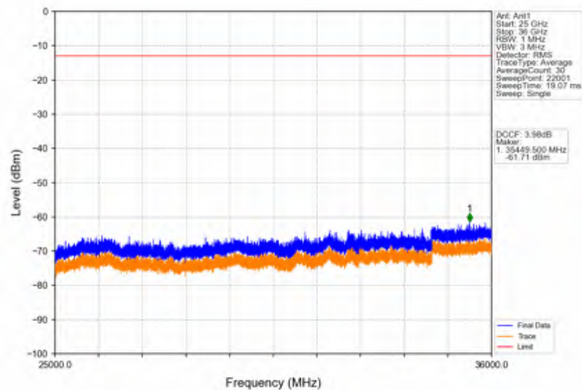
Band42c_15MHz_64QAM_HCH_3592.5MHz_RB_1_74_NTNV
