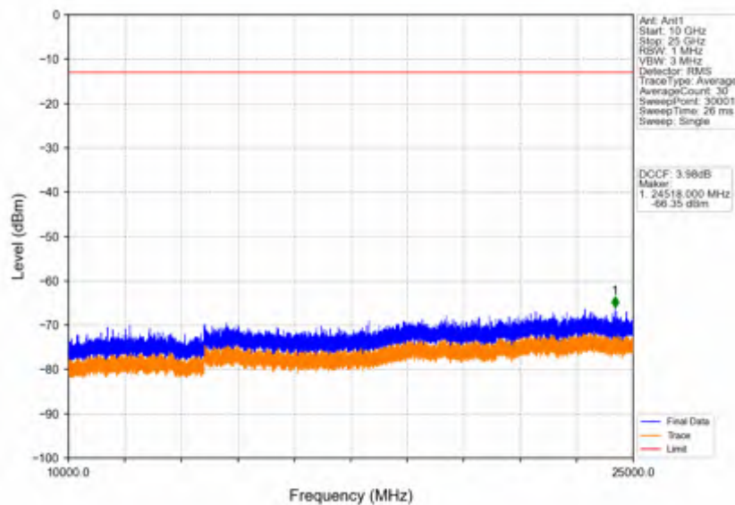
Band42c_5MHz_16QAM_LCH_3552.5MHz_RB_1_0_NTNV
