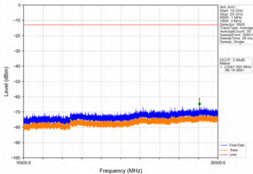
Band42c_5MHz_16QAM_MCH_3575MHz_RB_1_0_NTNV
