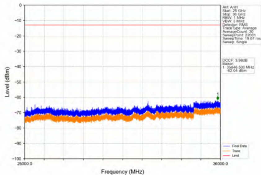
Band42c_15MHz_256QAM_LCH_3557.5MHz_RB_75_0_NTNV
