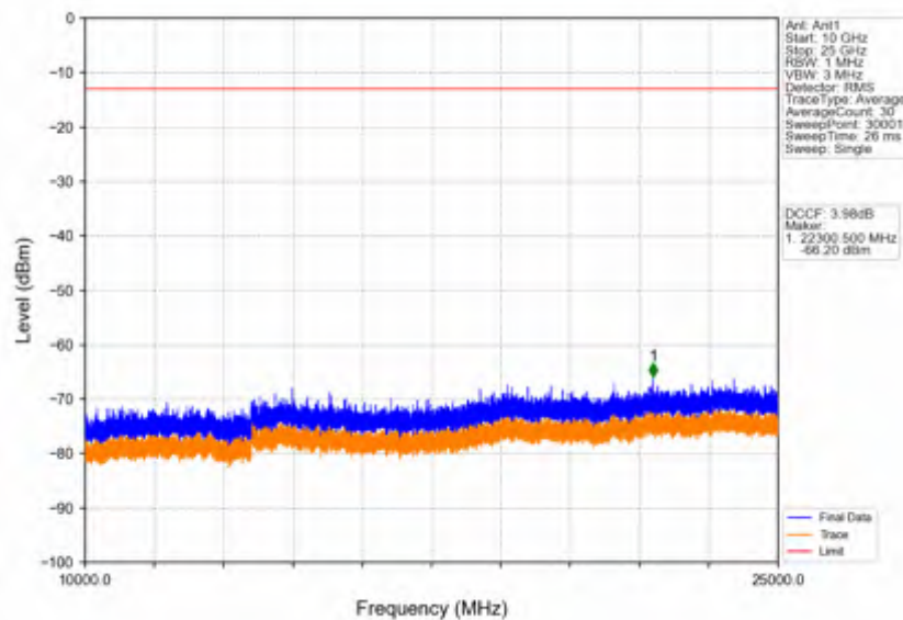
Band42c_10MHz_64QAM_MCH_3575MHz_RB_1_0_NTNV
