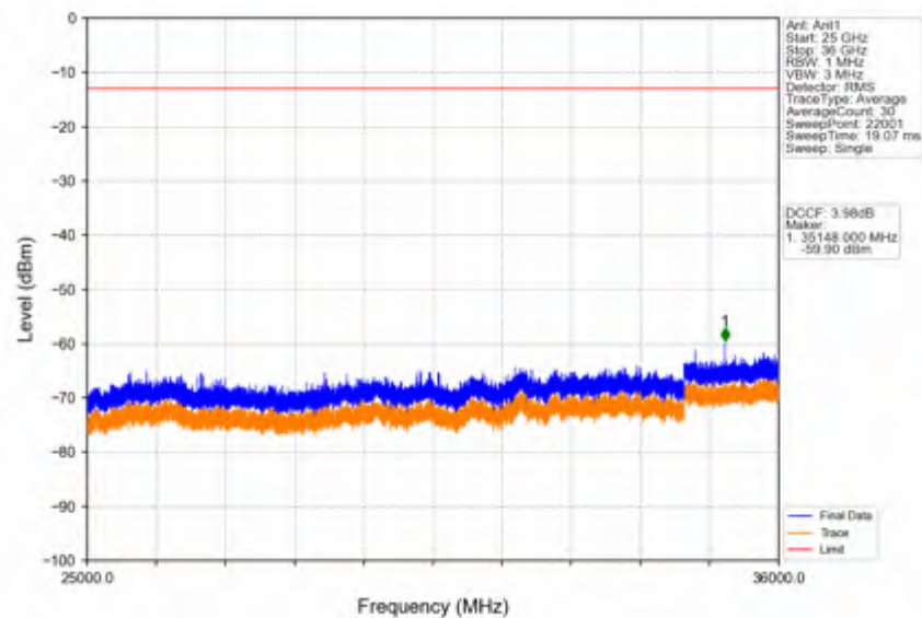
Band42c_10MHz_16QAM_LCH_3555MHz_RB_50_0_NTNV
