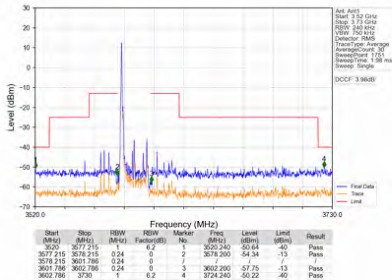
Band42c_20MHz_16QAM_HCH_3590MHz_RB_100_0_NTNV
