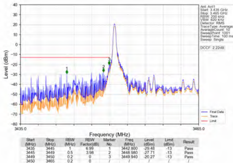
Band42a_15MHz_16QAM_LCH_3457.5MHz_RB_1_0_NTNV
