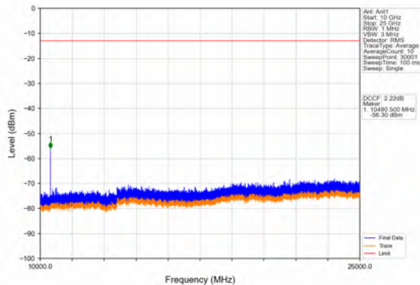
Band42a_15MHz_64QAM_MCH_3500MHz_RB_1_0_NTNV
