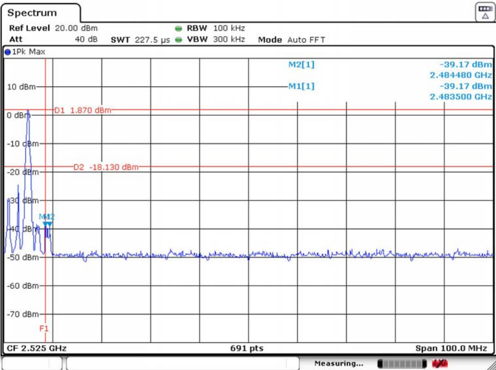
\pi /4-DQPSK High Channel Hopping OFF
