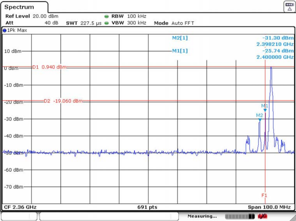
\pi /4-DQPSK Low Channel Hopping OFF
