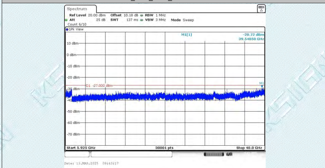
11A_Ant1_5745_5925~40000
