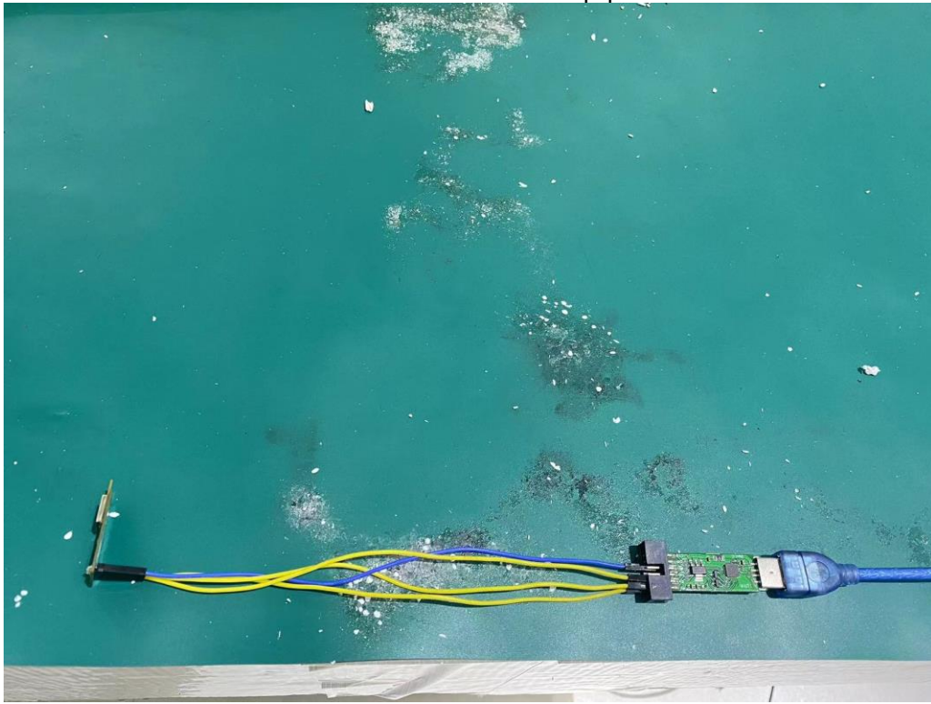
Radiated emission close-up photo
