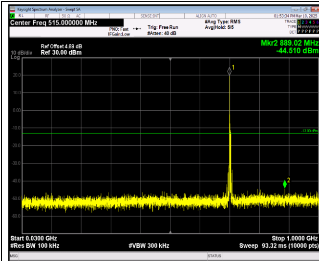
Band17-5MHz-64QAM-23825-1RB#0-Range1:30~1000MHz
