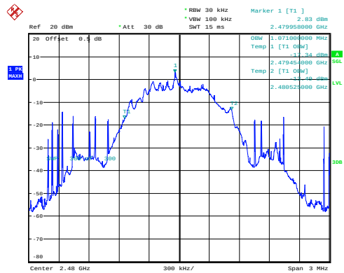
High 1.071MHz
