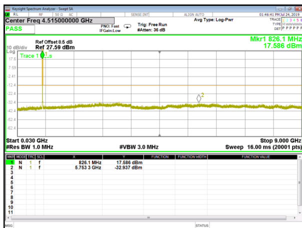
B5_HSDPA_Lower_Conducted Spurious
