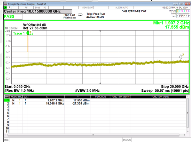
B2_HSDPA_Higher_Conducted Spurious
