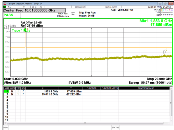
B2_HSDPA_Lower_Conducted Spurious
