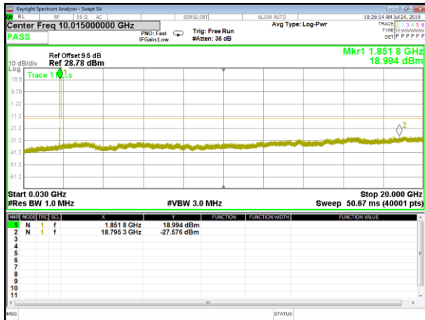
B2_WCDMA_Lower_Conducted Spurious
