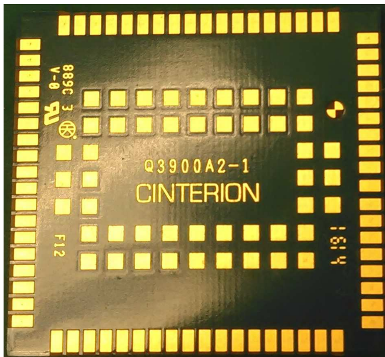
BGS8 - Bottom view
