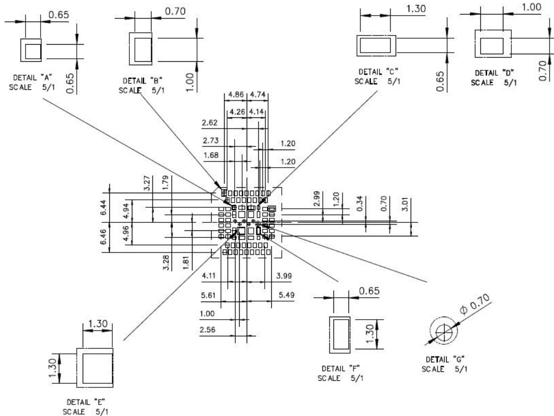
Figure 4-4. Pin dimensions
