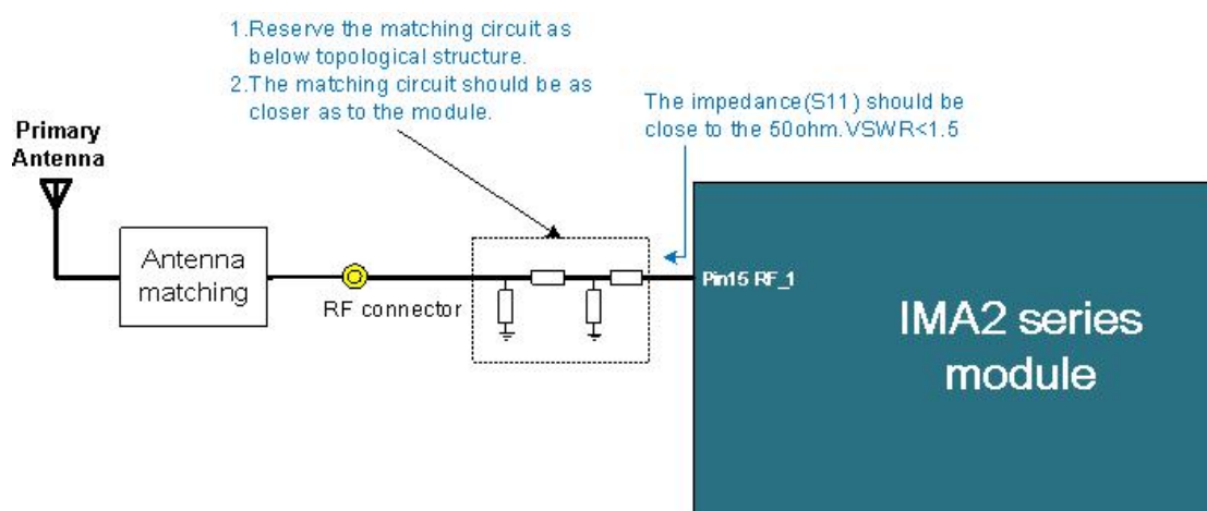
Figure 6-2. RF matching guide
