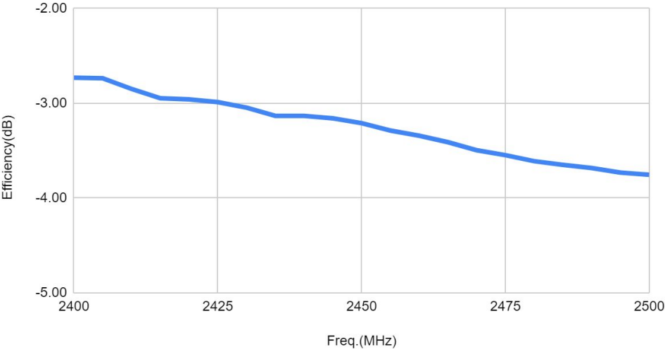
Antenna Efficiency
