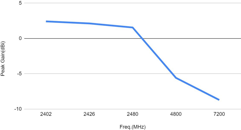
Peak Gain
