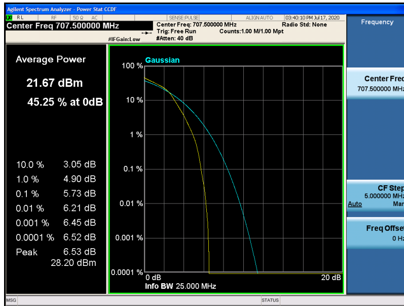
Band12-1.4MHz-16QAM-23095-6RB#0
