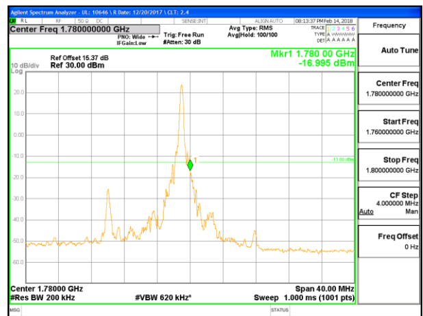
LTE B66 20MHz 16QAM High Channel RB1-74
