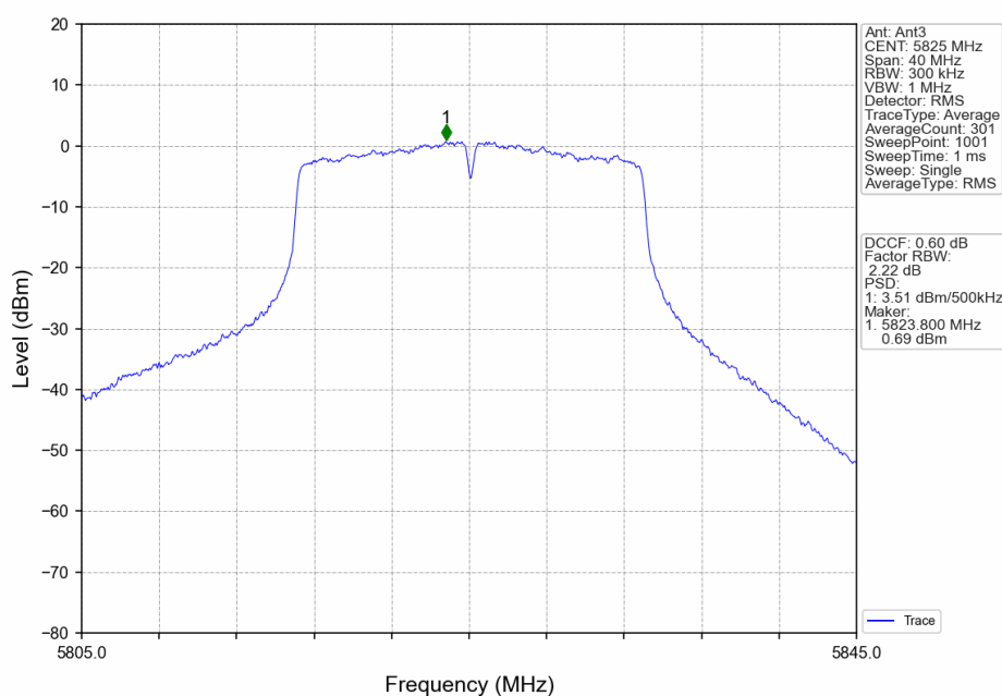
802.11ac(VHT20)_HCH_5825MHz_Ant3_NTNV
