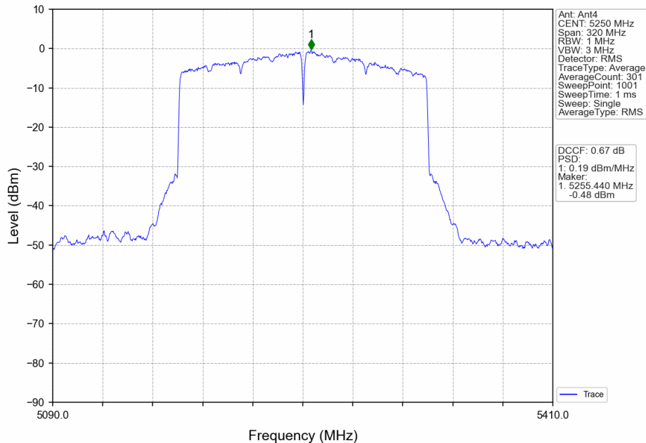
802.11ax(HEW160)_MCH_5250MHz_2xRU996_Left_MIMO_NTNV
