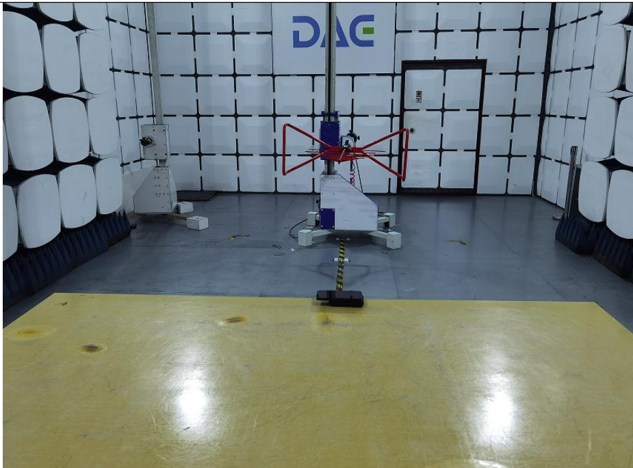
Emissions in frequency bands (below 30MHz) -TM7
