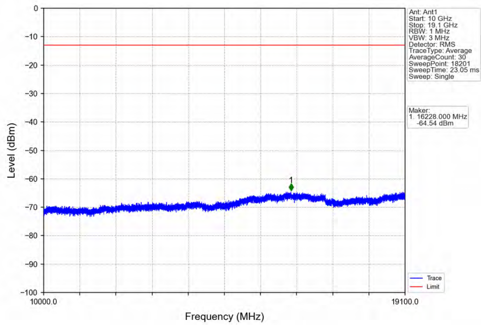
Band2_HSUPA_HCH_1907.6MHz_Subtest 1_NTNV
