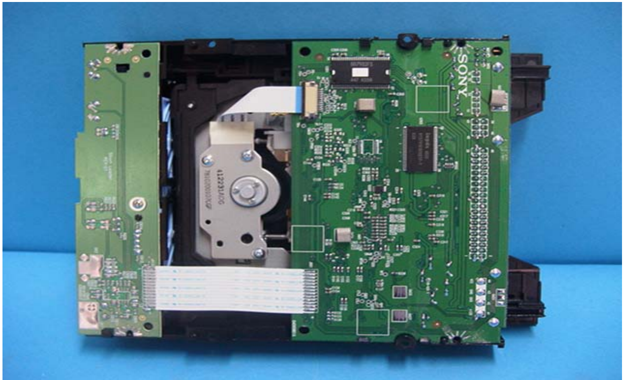
DVD Deck Bottom View(Removed Cover)
